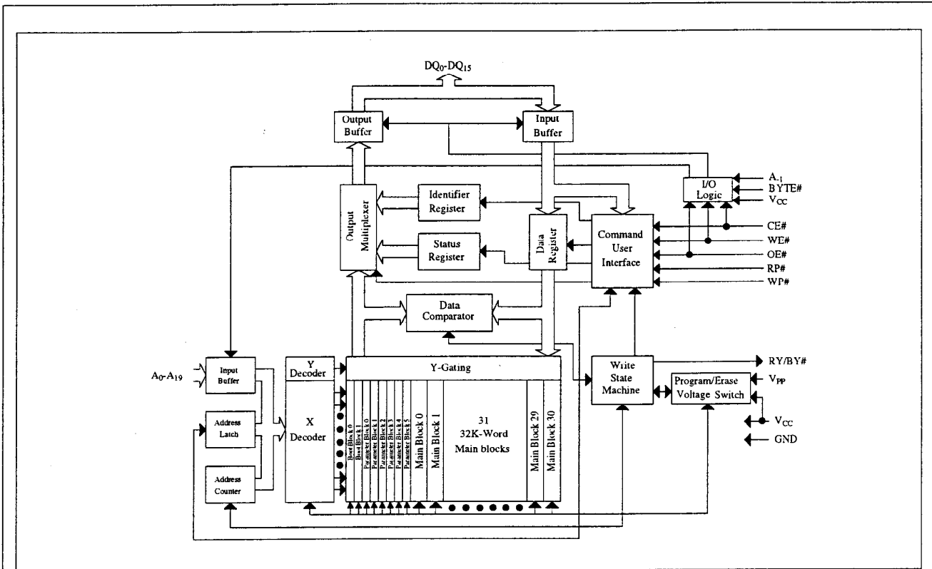
Figure 1. Block Diagram
