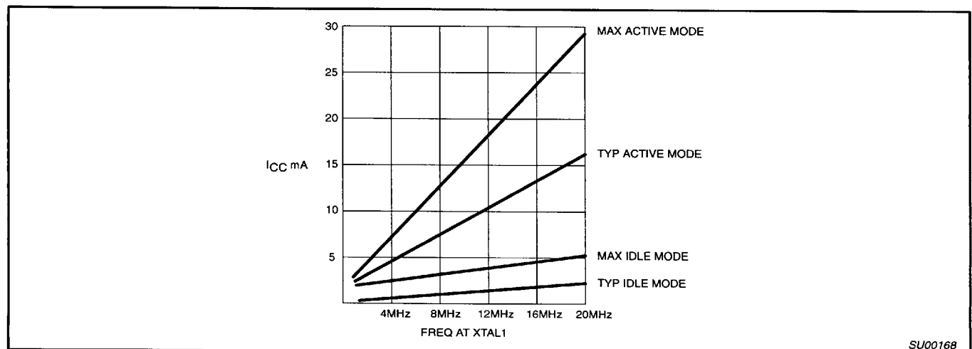
Figure 9. I_{CC} vs. FREQ.
