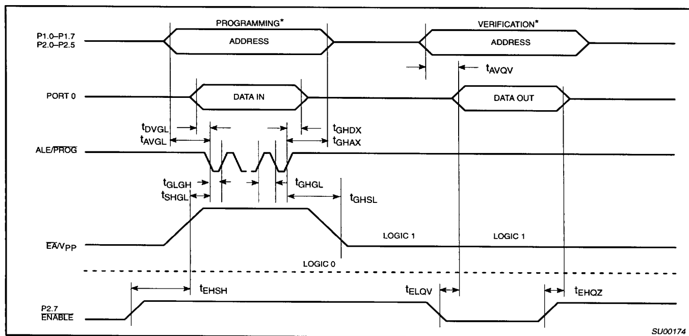
Figure 17. EPROM Programming and Verification
