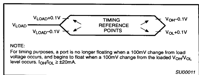
Figure 8. Float Waveform
