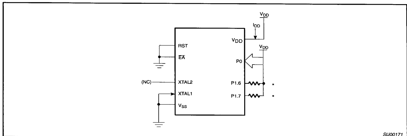
Figure 13. I_{DD} Test Condition, Power Down Mode All other pins are disconnected. V_{DD} = 2\text{V to } 5.5\text{V}
