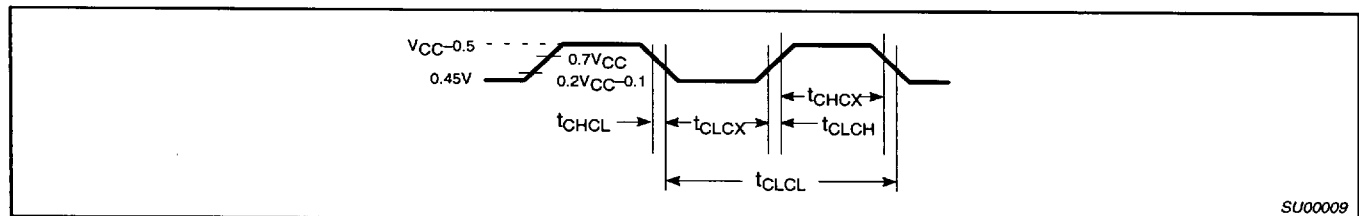
Figure 6. External Clock Drive
