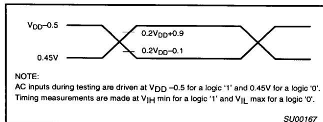
Figure 7. AC Testing Input/Output
