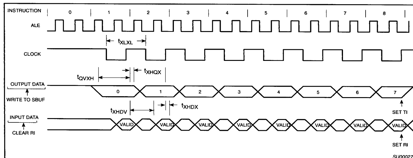
Figure 4. Shift Register Mode Timing
