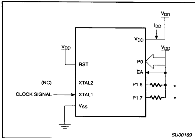
Figure 10. I_{DD} Test Condition, Active Mode All other pins are disconnected
