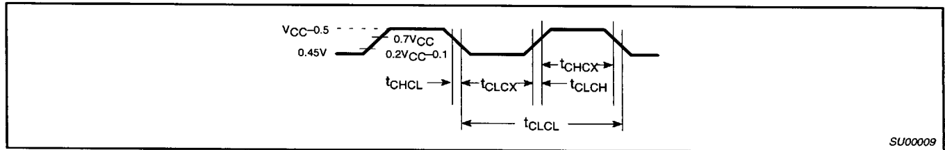
Figure 12. Clock Signal Waveform for I_{DD} Tests in Active and Idle Modes t_{CLCH} = t_{CHCL} = 5\text{ns}
