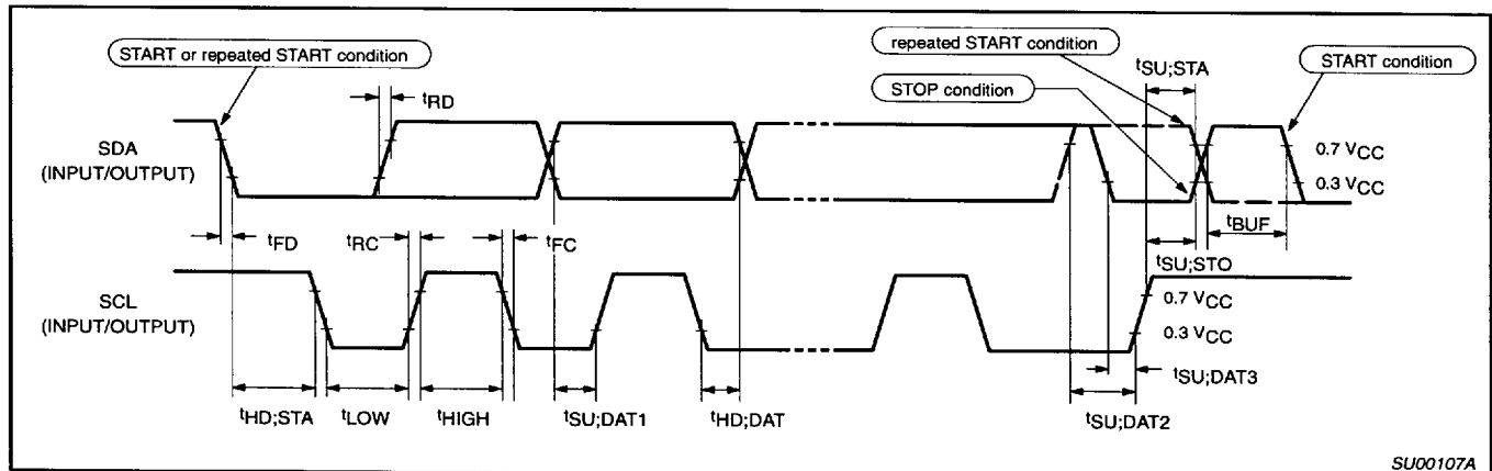
Figure 5. Timing SIO1 (I²C) Interface
