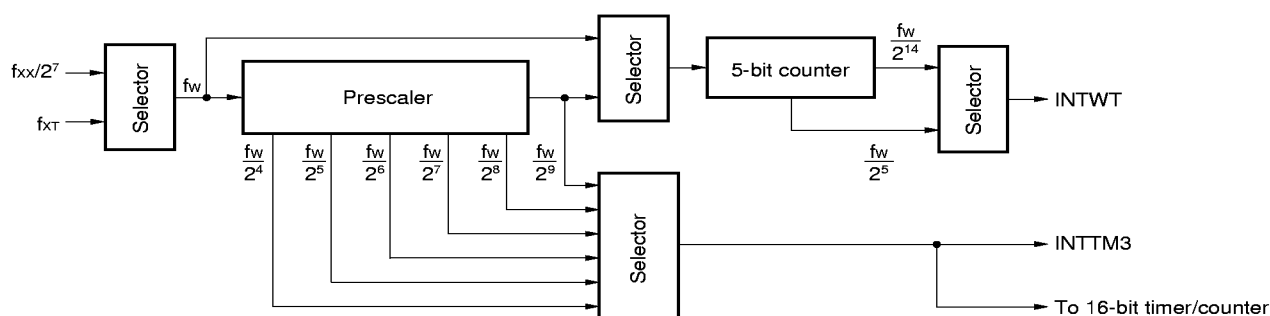
Figure 7-15. Block Diagram of Watch Timer
