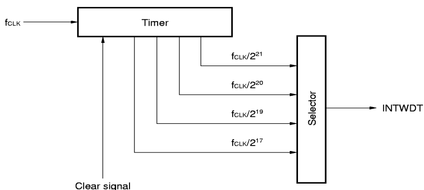
Figure 7-16. Block Diagram of Watchdog Timer
