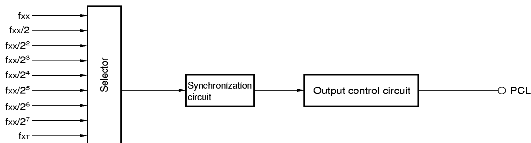
Figure 7-13. Block Diagram of Clock Output Function
