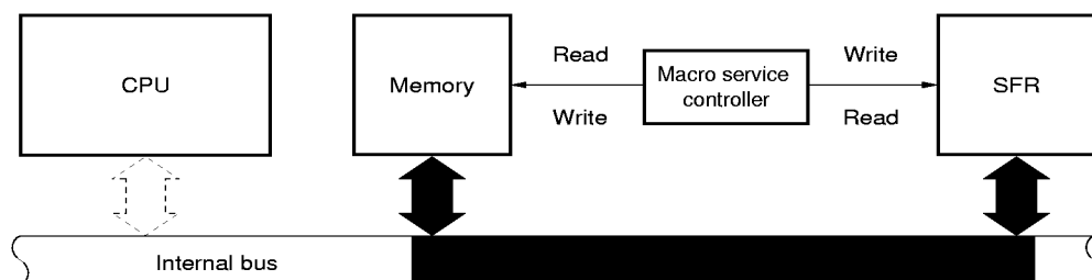
Figure 8-2. Macro Service
