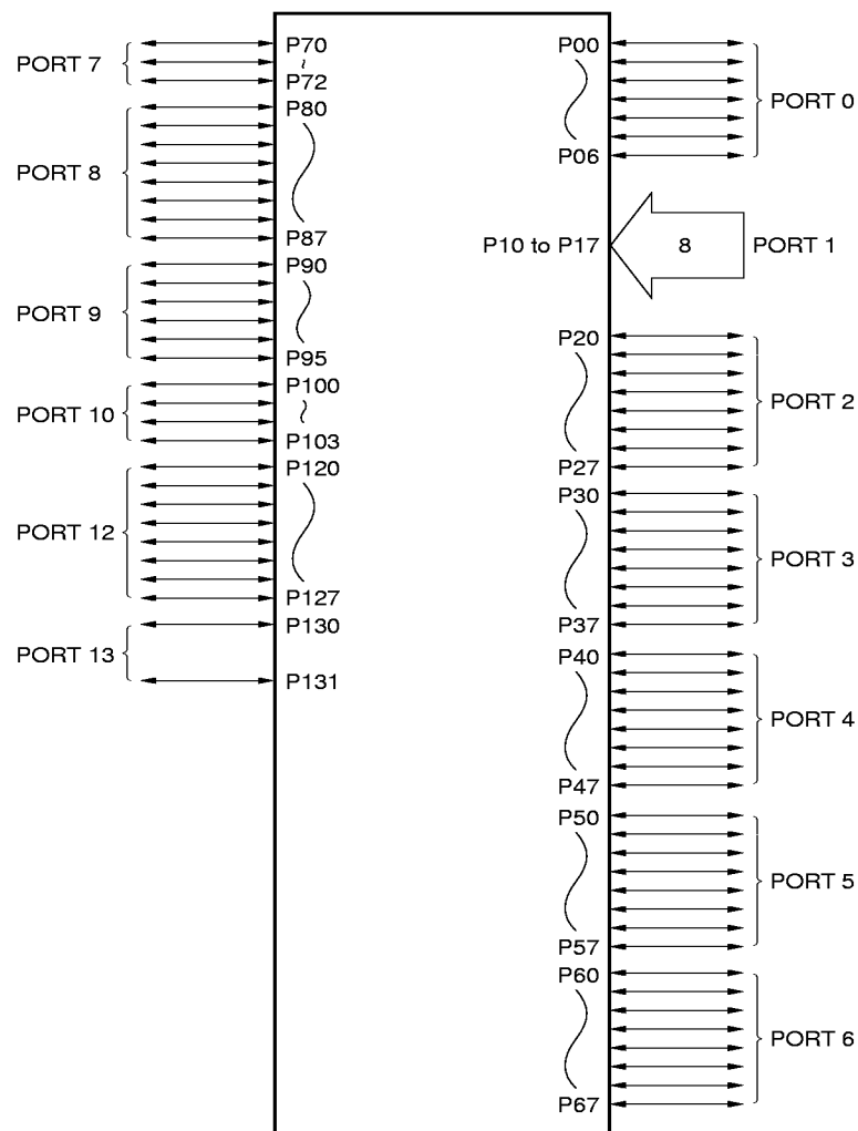
Figure 7-1. Port Configuration
