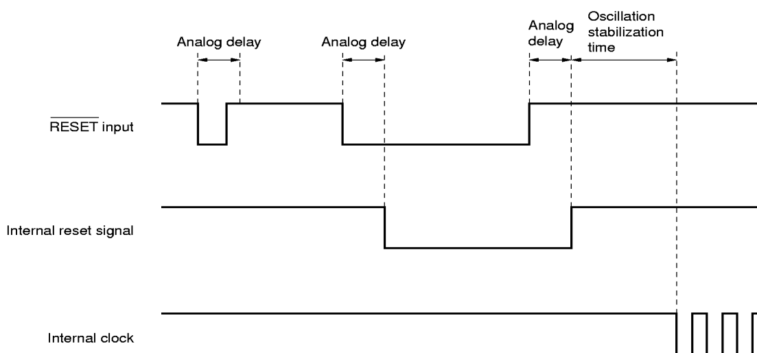
Figure 11-2. Acknowledgement of Reset Signal
