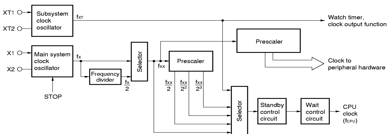
Figure 7-2. Block Diagram of Clock Generation Circuit
