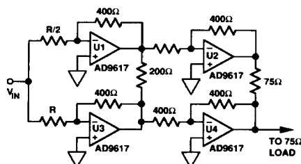
Input Impedance = R/3 Gain = +400\ \Omega / R ( V_{OUT} = 2\ \text{V p-p} ) Low-Distortion Drive Circuit for AD9014
