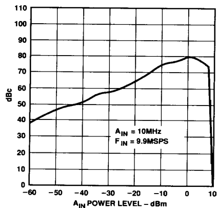
AD9014K TYPICAL PERFORMANCE SPURIOUS FREE DYNAMIC RANGE (SFDR) VS. INPUT POWER LEVEL
