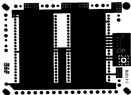
Layer 1 (Bottom)
