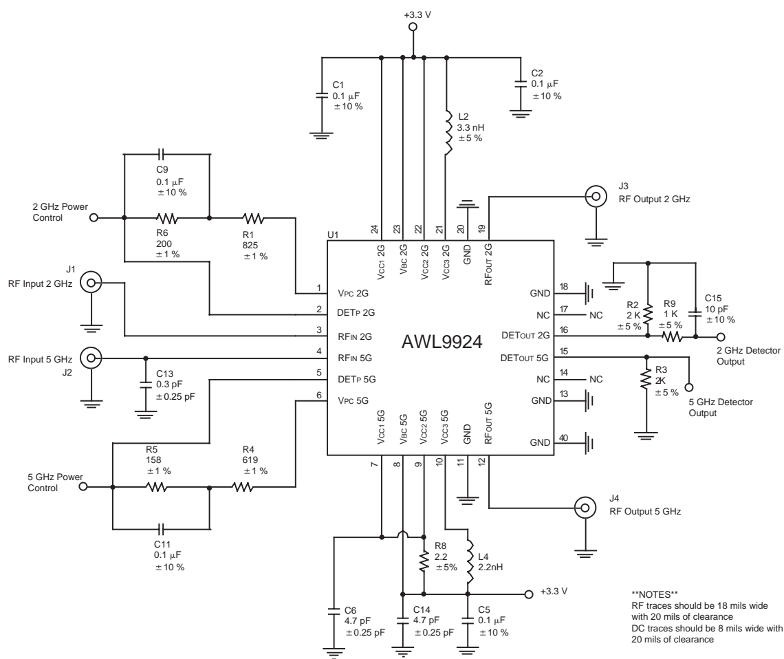
Figure 35: Application Circuit
