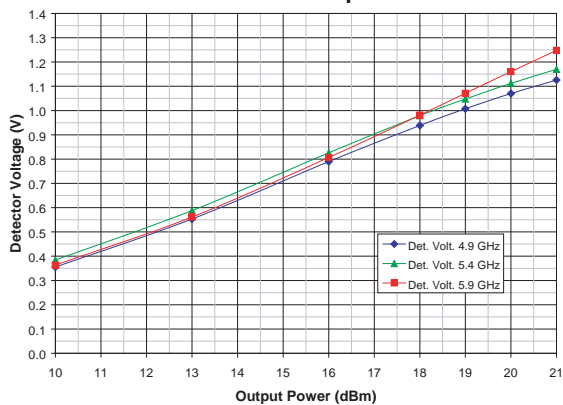
Figure 26: Detector Voltage vs. Output Power Across Freq ( V_{CC} = +3.3\text{ V} , T_c = 25^\circ\text{C} , 2\text{ K}\Omega Load) 5 GHz 802.11a 54 Mbps OFDM
