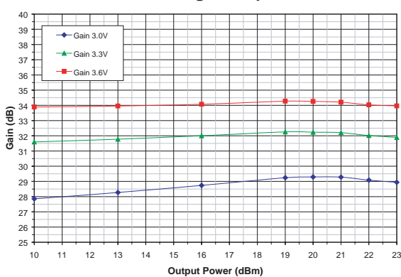
Figure 6: Gain vs. Output Power Across Power Supply Voltage (Frequency = 2.45 GHz, T_C = 25^\circ\text{C} ) 2.4 GHz 802.11g 54 Mbps OFDM
