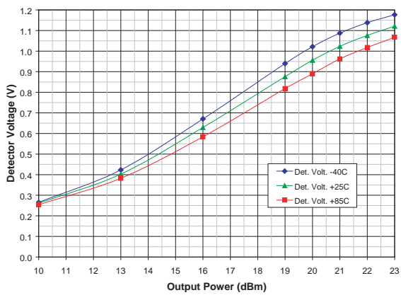
Figure 18: Detector Voltage vs. Output Power Across Temp (Freq = 2.45 GHz, V_{CC} = +3.3\text{ V} , 2\text{ K}\Omega Load) 2.4 GHz 802.11b Gaussian Filtering (BT = 0.45), 1 Mbps
