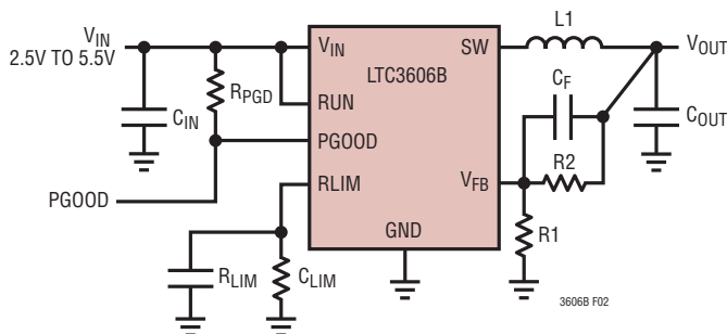
Figure 2. LTC3606B General Schematic
