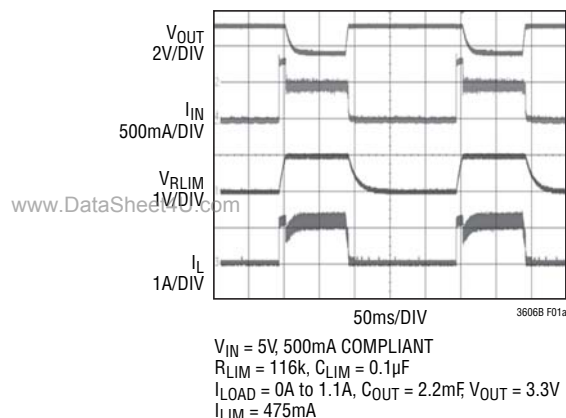
Figure 1a. Input Current Limit Within 100ms Load Pulses
