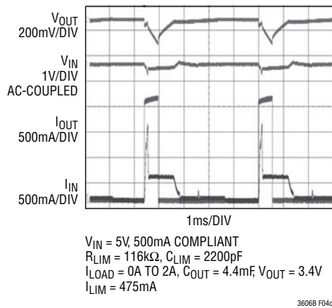
Figure 4c. Transient Response
