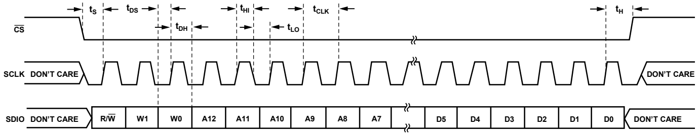
Figure 32. Serial Timing Details
