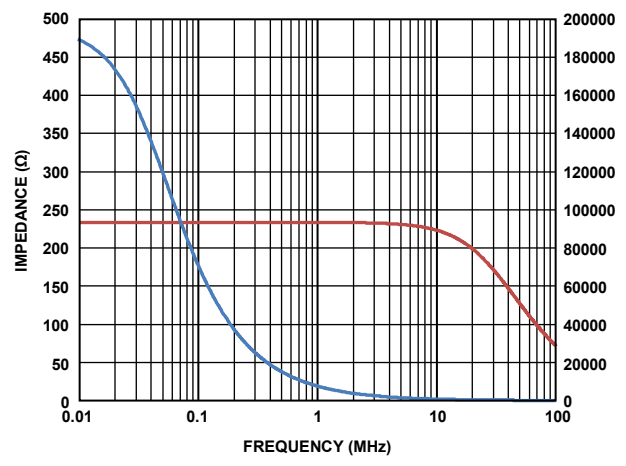
Figure 18. R_{IN} vs. Frequency
