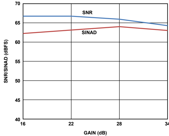
Figure 13. SNR vs. Gain
