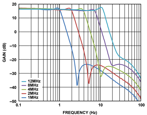
Figure 14. Filter Response
