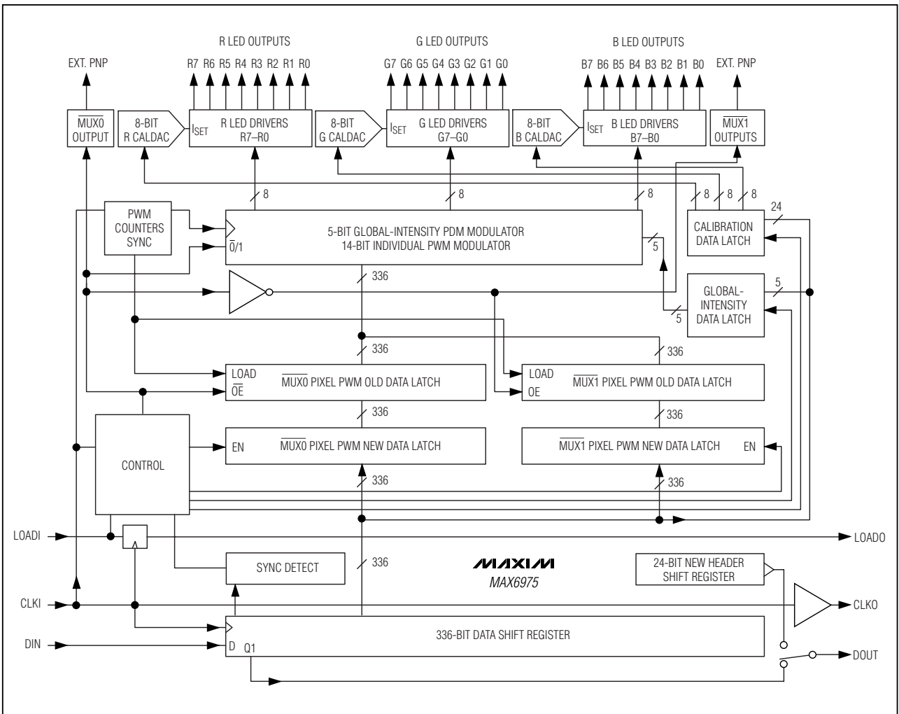
MAX6975 Block Diagram
