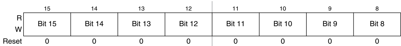
Figure 14-19. Timer Input Capture/Output Compare Register 0 High (TC0)
