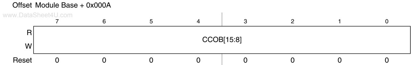
Figure 23-16. Flash Common Command Object High Register (FCCOBHI)
