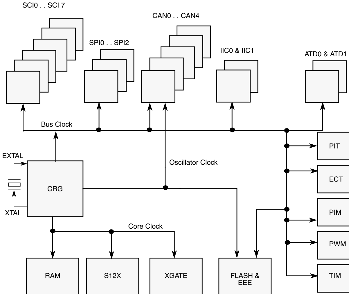
Figure 1-8. Clock Connections
