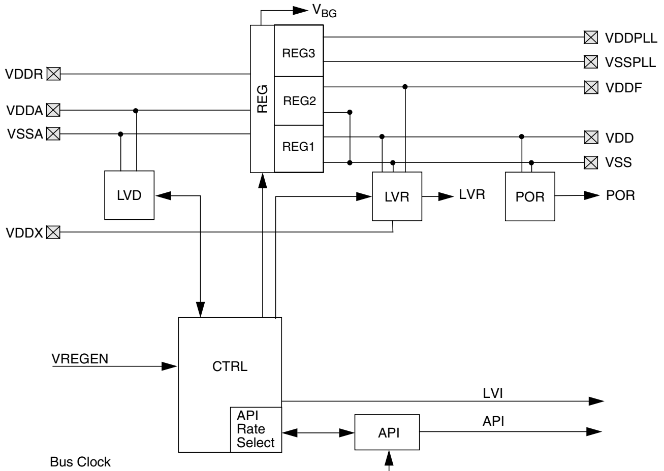
Figure 22-1. VREG_3V3 Block Diagram
