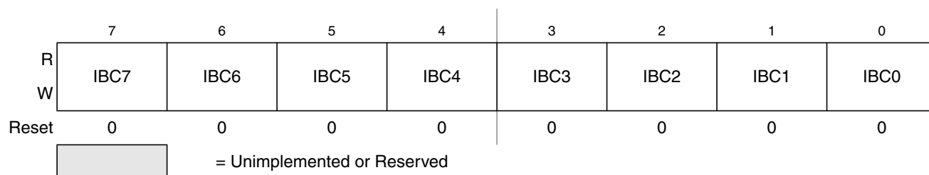
Figure 15-4. IIC Bus Frequency Divider Register (IBFD)
