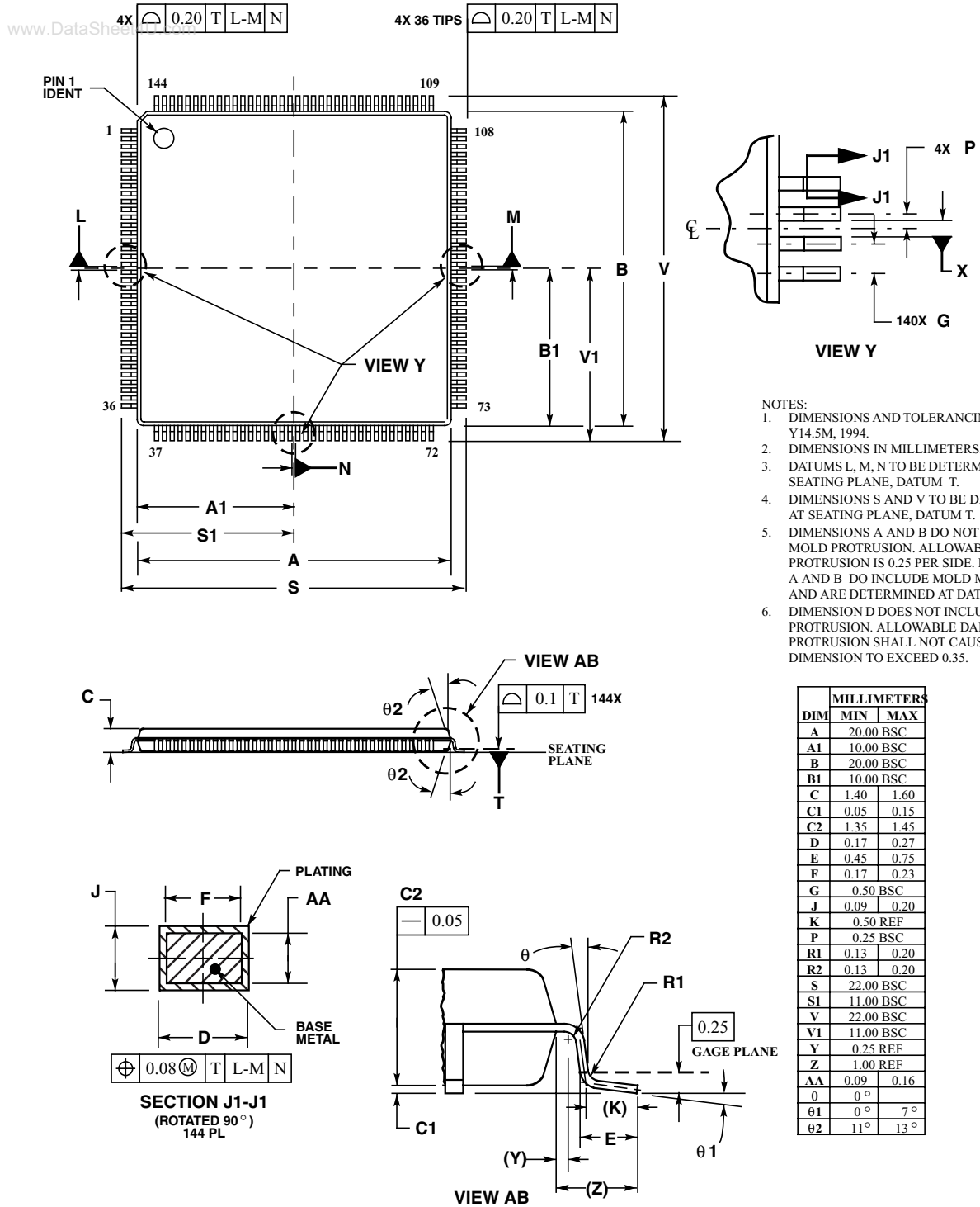
Figure B-2. 144-Pin LQFP Mechanical Dimensions (Case No. 918-03)
