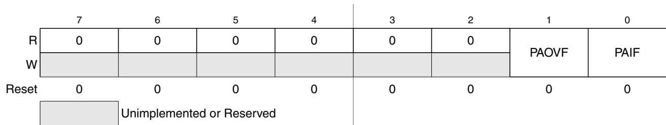
Figure 21-25. Pulse Accumulator Flag Register (PAFLG)
