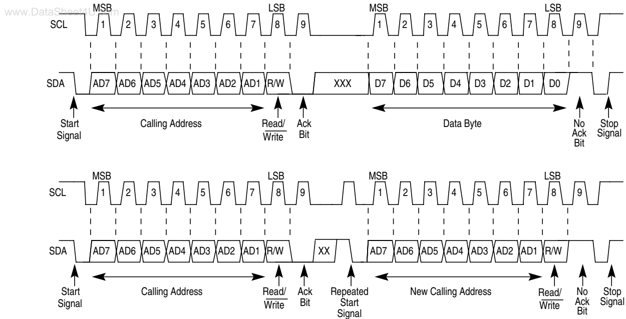
Figure 15-10. IIC-Bus Transmission Signals
