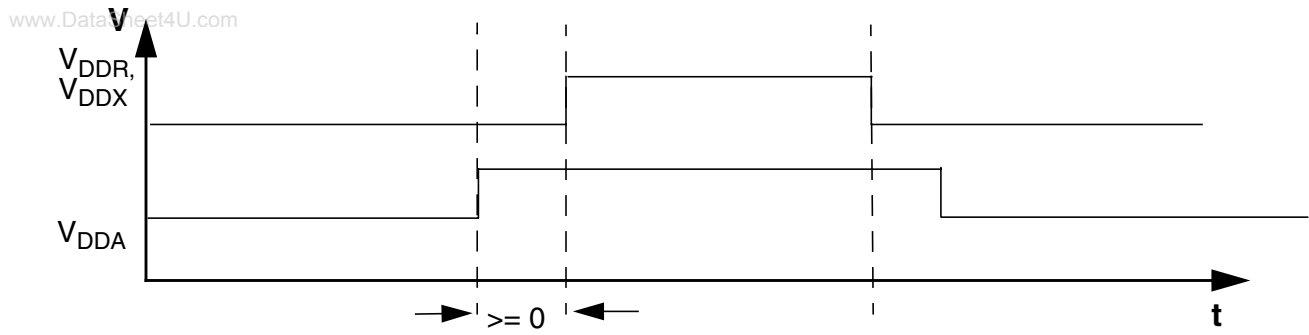
Figure A-4. MC9S12XE-Family Power Sequencing
