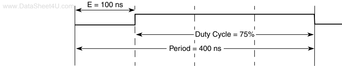
Figure 18-21. PWM Left Aligned Output Example Waveform
