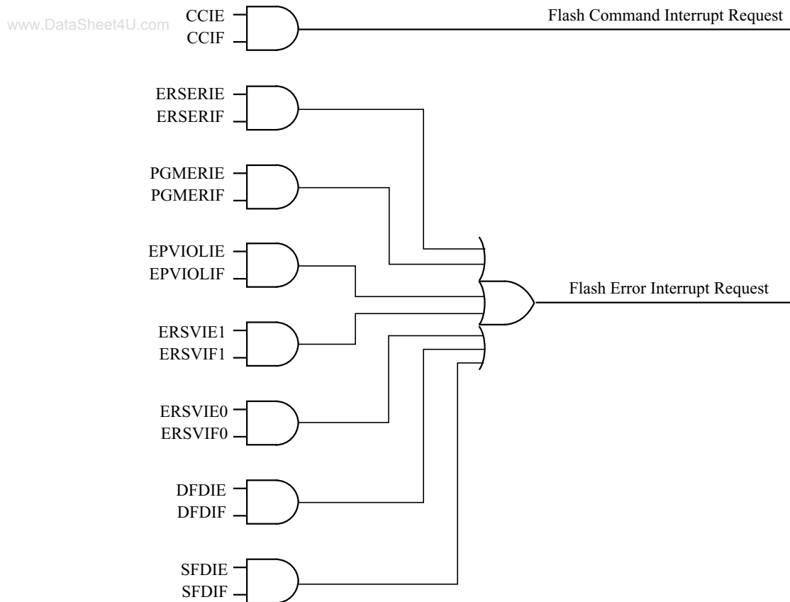
Figure 23-27. Flash Module Interrupts Implementation
