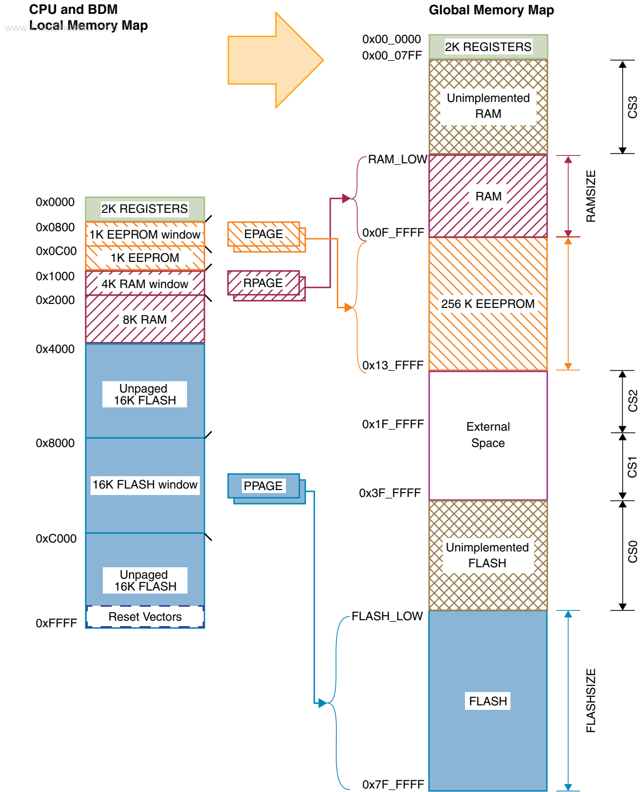
Figure 3-19. S12XE CPU & BDM Global Address Mapping
