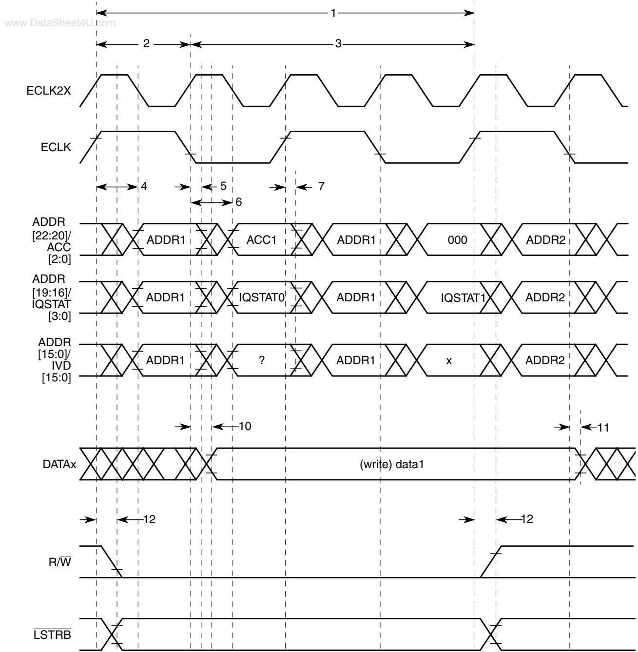
Figure A-17. Example 2b: Emulation Expanded Mode 0 Write with 1 Stretch Cycle
