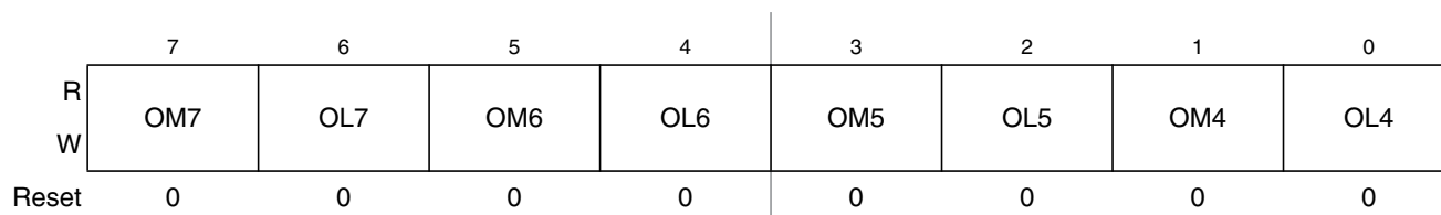
Figure 21-14. Timer Control Register 1 (TCTL1)
