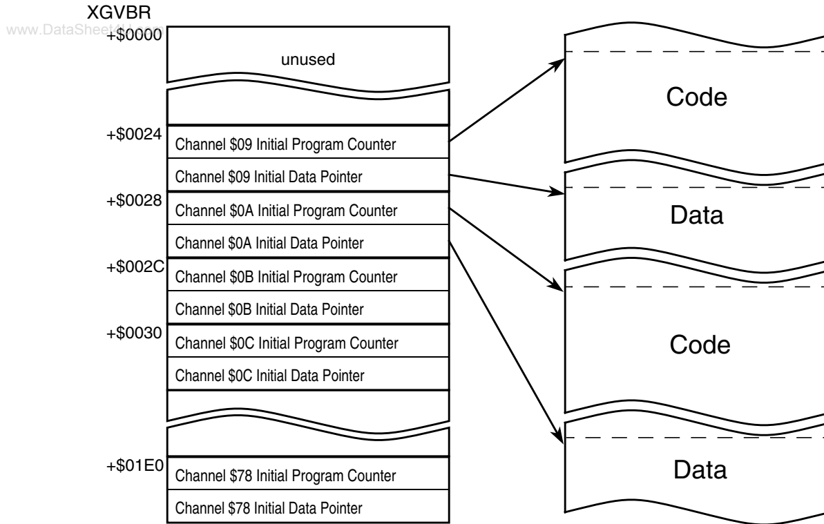
Figure 10-23. XGATE Vector Block
