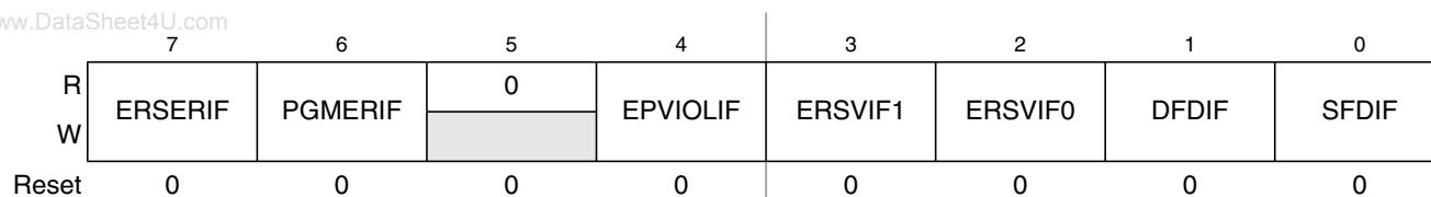
Figure 23-12. Flash Error Status Register (FERSTAT)
