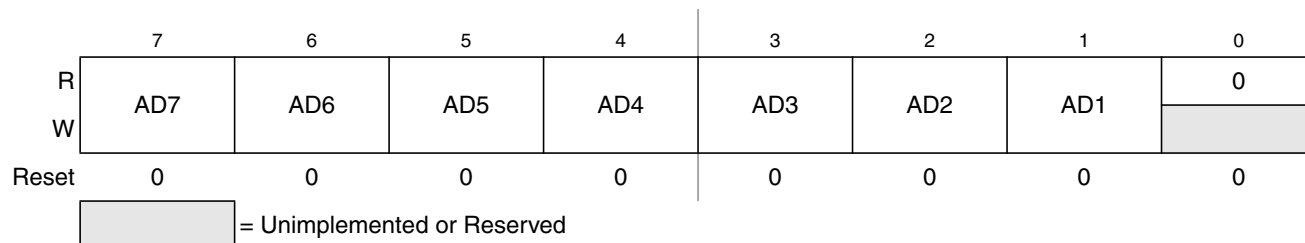
Figure 15-3. IIC Bus Address Register (IBAD)
