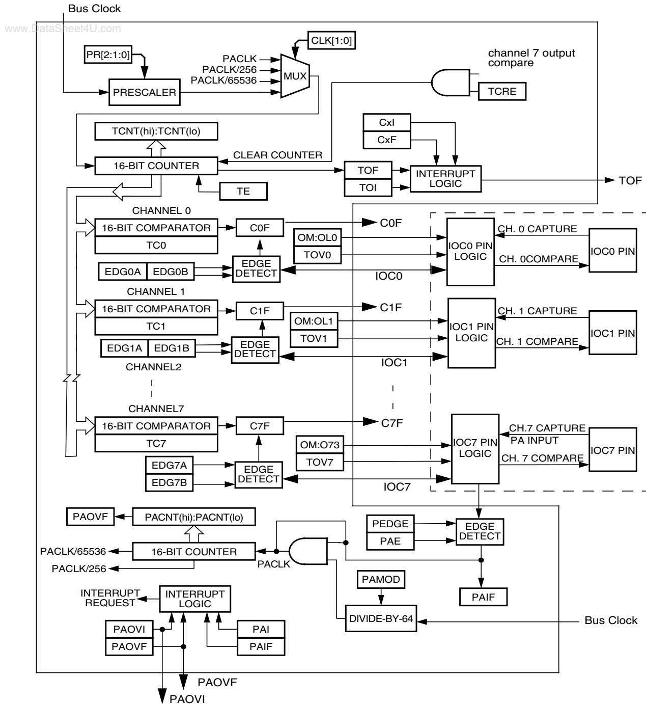
Figure 21-30. Detailed Timer Block Diagram
