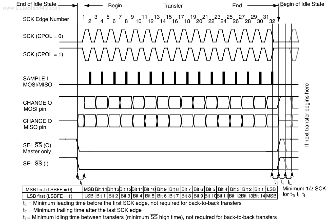
Figure 20-15. SPI Clock Format 1 (CPHA = 1), with 16-Bit Transfer Width selected (XFRW = 1)
