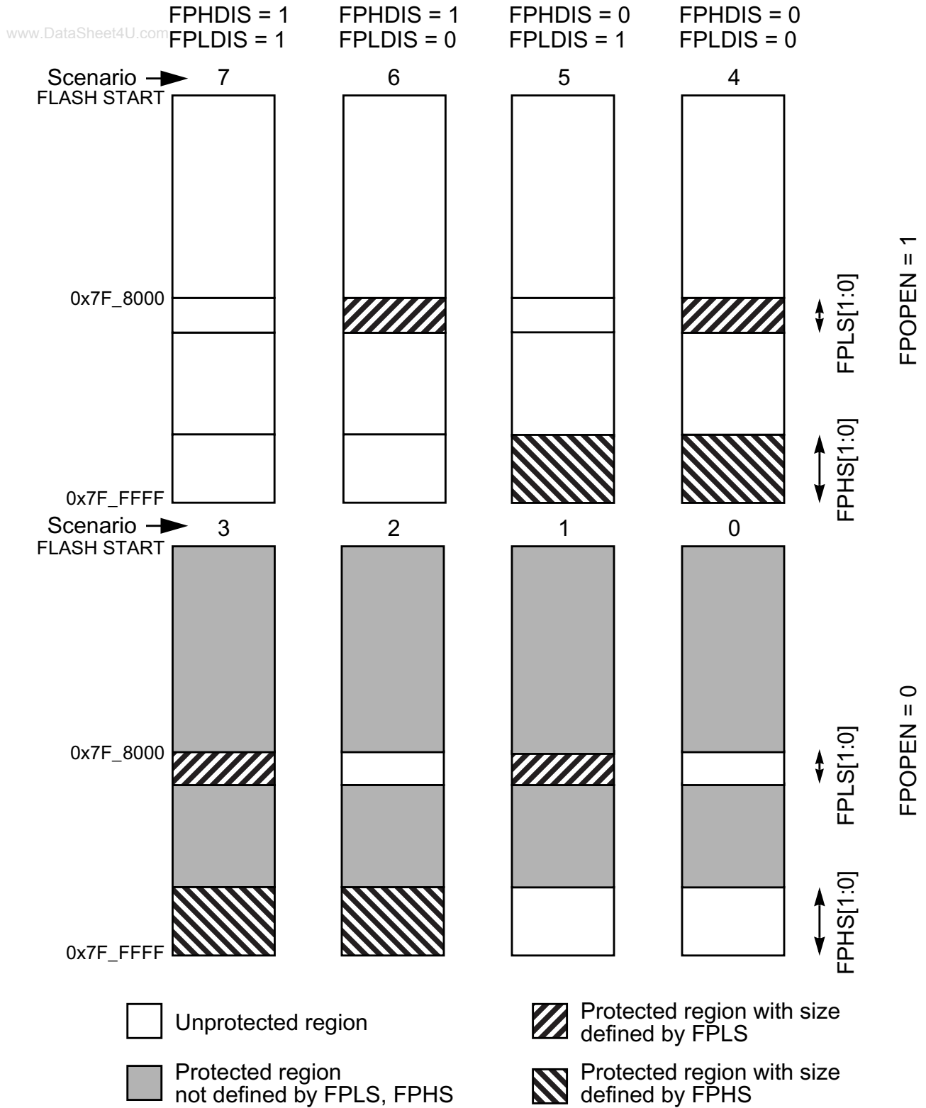
Figure 23-14. P-Flash Protection Scenarios
