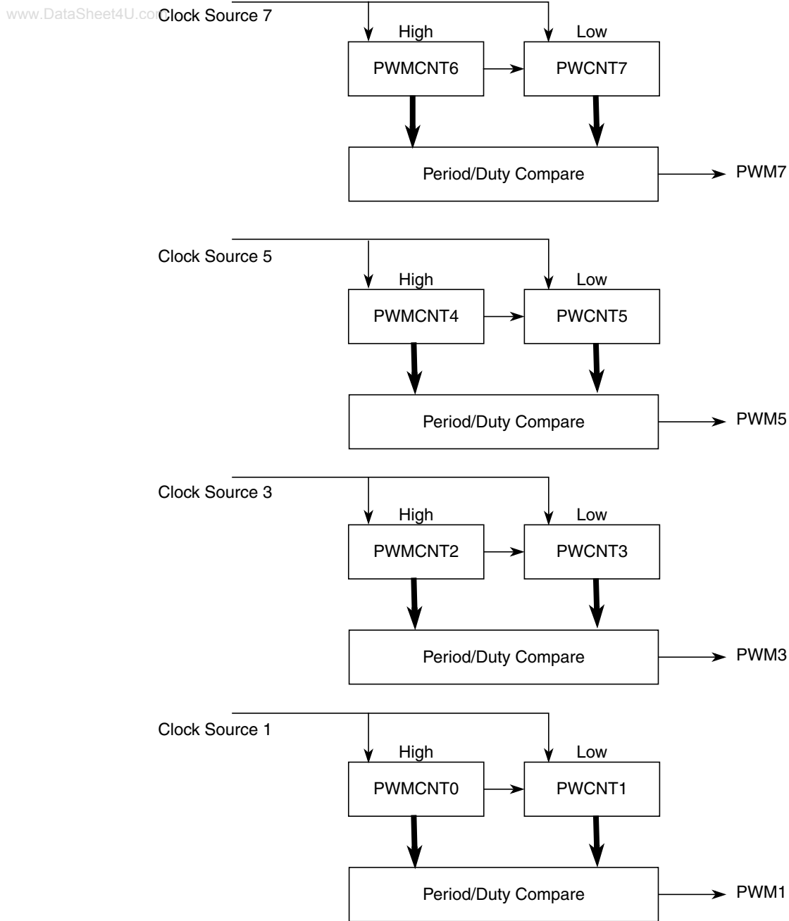
Figure 18-24. PWM 16-Bit Mode
