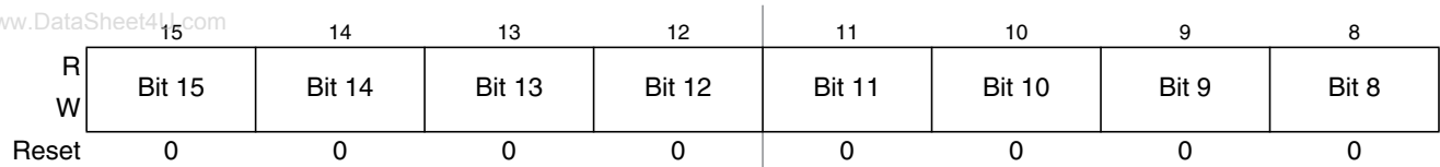
Figure 14-31. Timer Input Capture/Output Compare Register 6 High (TC6)
