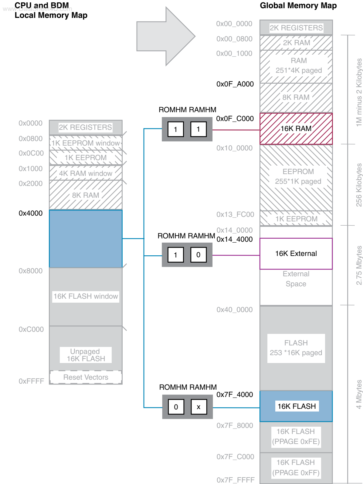
Figure 3-21. ROMHM, RAMHM Memory Configuration
