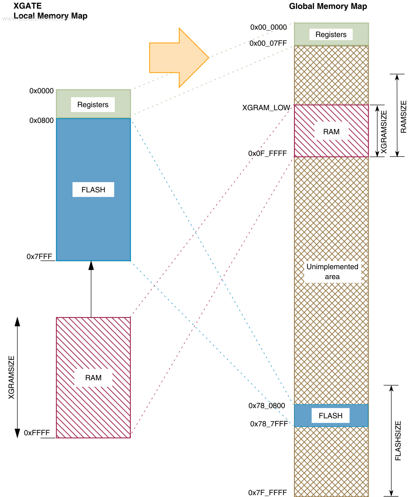
Figure 3-20. XGATE Global Address Mapping
