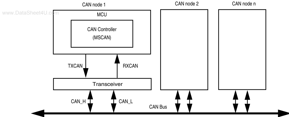
Figure 16-2. CAN System
