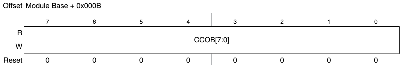
Figure 23-17. Flash Common Command Object Low Register (FCCOBLO)
