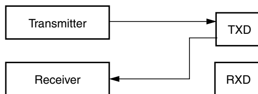
Figure 19-30. Single-Wire Operation (LOOPS = 1, RSRC = 1)
