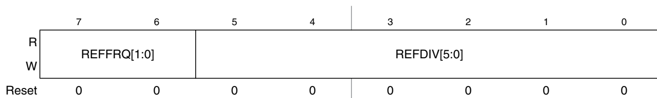
Figure 11-4. S12XECRG Reference Divider Register (REFDV)
