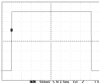
20ms Pulse, 150A, 40V Output 2.5ms/Div horizontal scale, 25A/Div vertical scale
