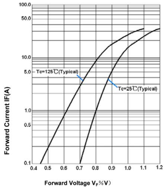
Fig.4 Forward Voltage
