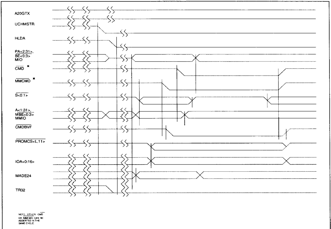
Figure 8. Address Mode: 80386/80486/DMA Channel Accesses
