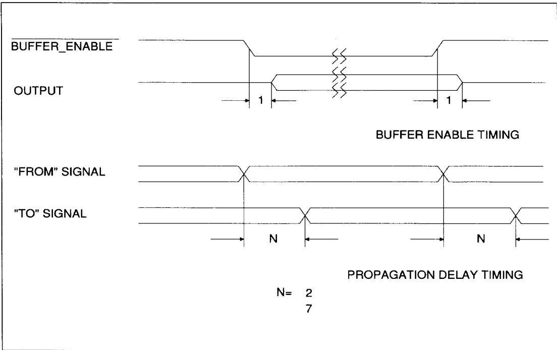
Figure 17. Data Buffer Mode: Propagation Delay Timings
