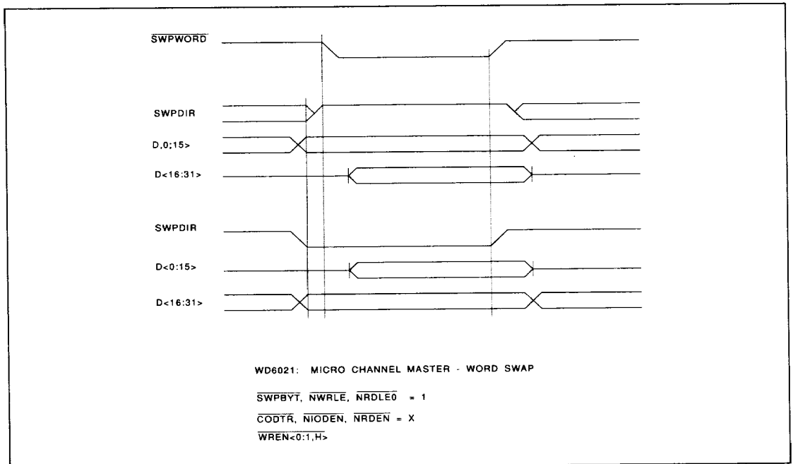
Figure 13. Data Mode: Channel Master Word Swap
