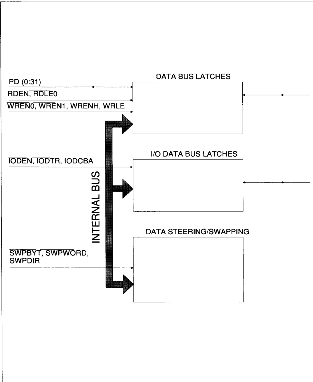
Figure 4. Data Buffer Mode Block Diagram
