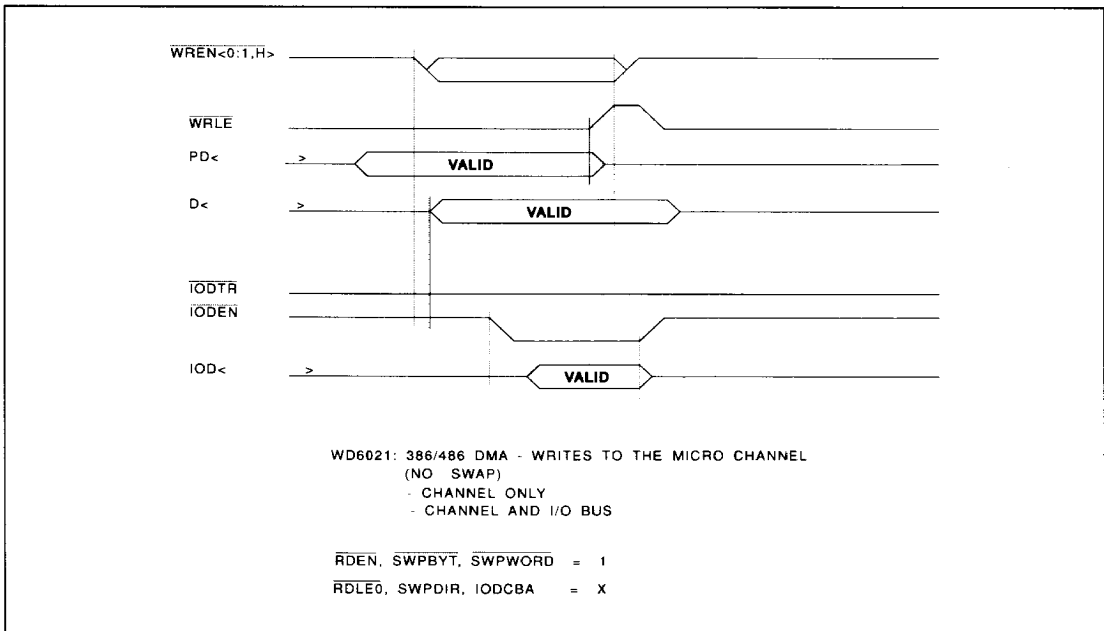
Figure 11. Data Mode: 80386/80486/DMA Writes to the Channel
