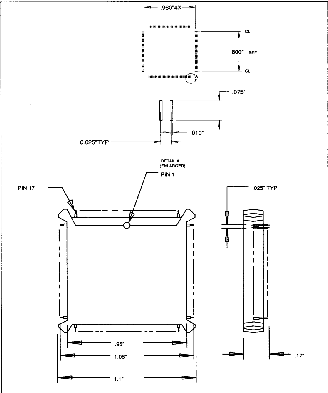
Figure 21. 132-Pin JEDEC Flat Pack Packaging Diagram
