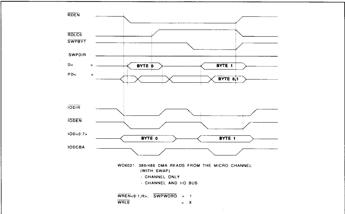
Figure 10. Data Mode: 80386/80486/DMA Reads from the Channel with Swap
