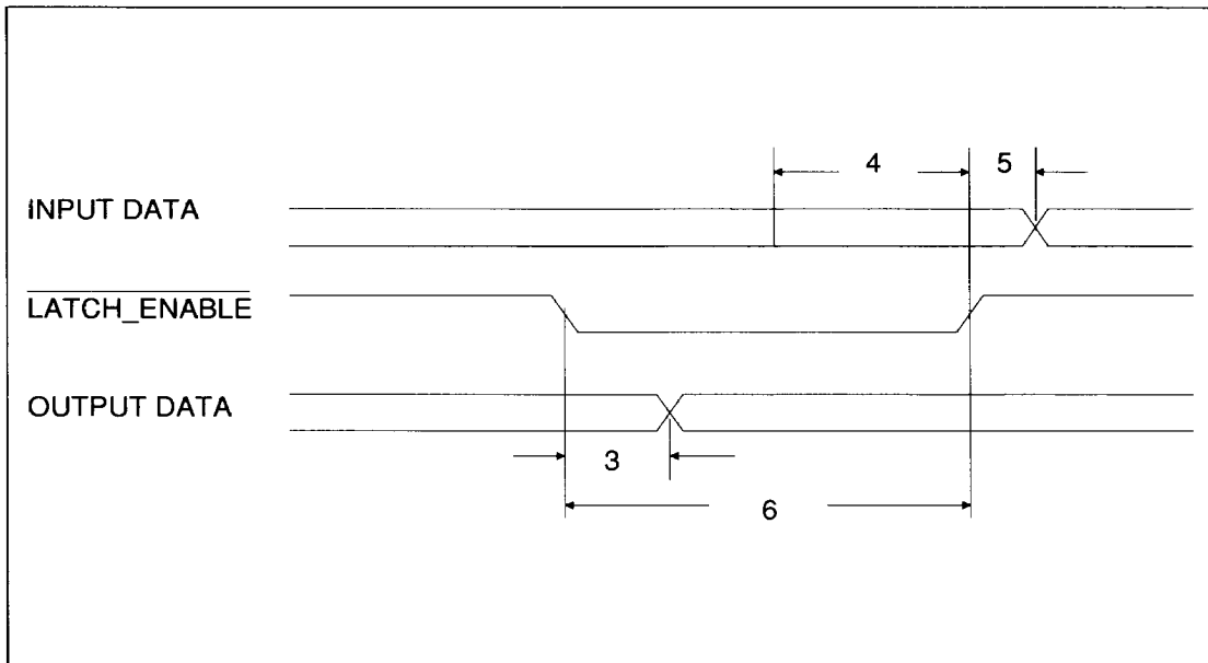
Figure 18. Data Buffer Mode: Latch Timings
