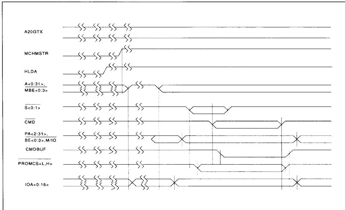
Figure 7. Address Mode: Channel Master Accesses
