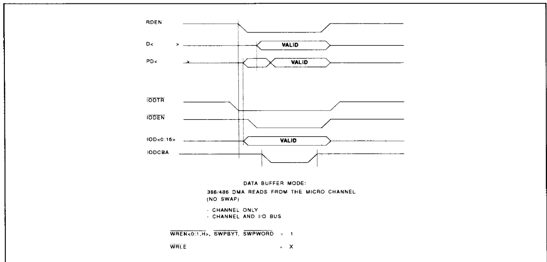
Figure 9. Data Mode: 80386/80486/DMA Reads from the Channel
