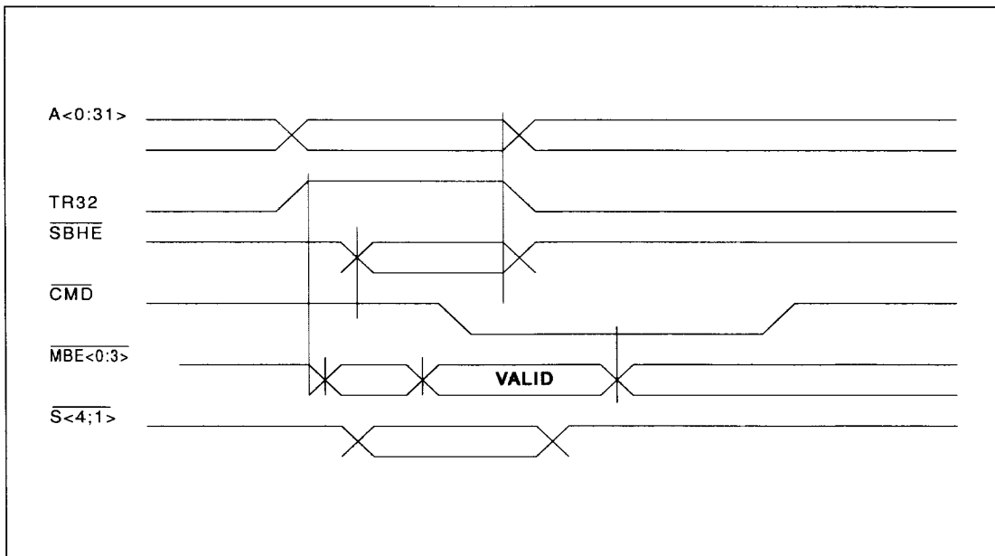
Figure 6. Address Mode: Channel Master Accesses Translate Function
