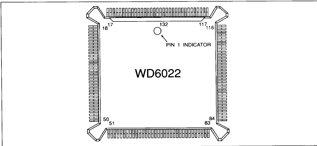
Figure 5. Data Buffer Mode Pin Diagram
