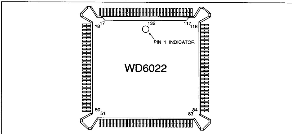
Figure 3. Address Buffer Mode Pin Diagram
