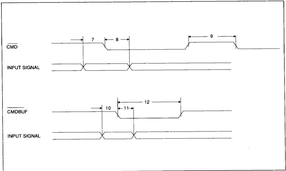
Figure 15. Address Buffer Mode: Latch Timings
