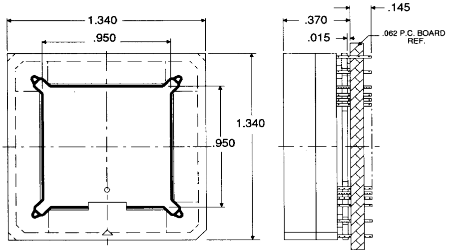
Figure 22. Socket Diagram
