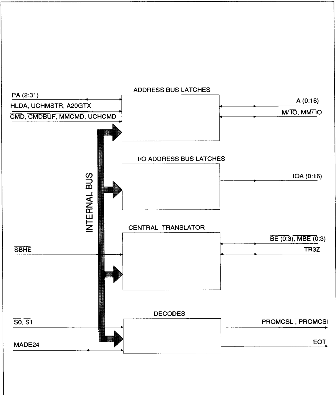
Figure 2. Address Buffer Mode Block Diagram
