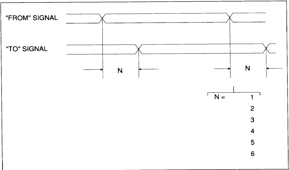
Figure 14. Address Buffer Mode: Propagation Delay Timings
