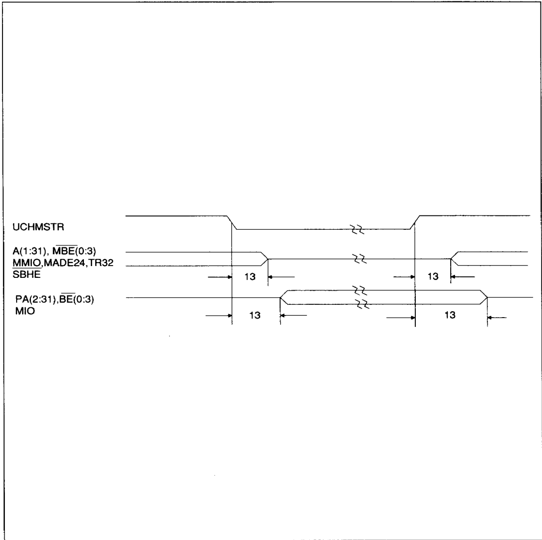
Figure 16. Address Buffer Mode: Float/Enable Timings
