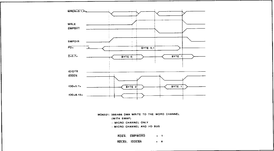
Figure 12. Data Mode: 80386/80486/DMA Writes to the Channel with Swap
