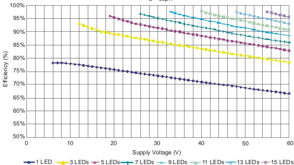
ZXLD1356 Efficiency L = 68μH
