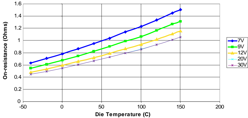
Lx on-resistance vs die temperature
