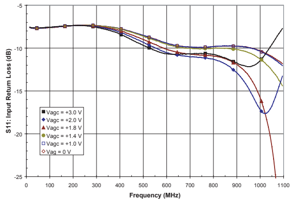
Figure 4: Input Return Loss vs. Frequency ( T_A = +25\text{ }^\circ\text{C} , V_{CC} = +5\text{ V} )
