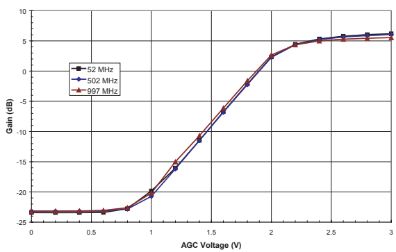
Figure 10: Gain vs. AGC Voltage (TA = +25 °C, VCC = + 5 V)
