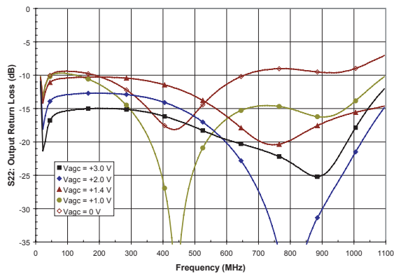
Figure 5: Output Return Loss vs. Frequency ( T_A = +25\text{ }^\circ\text{C} , V_{CC} = +5\text{ V} )
