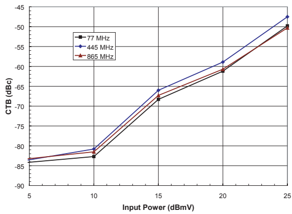
Figure 8: CTB vs. Input Power (TA = +25 °C, VCC = + 5 V, POUT = +6 dBmV, 135 channel flat input)
