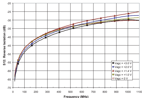
Figure 6: Reverse Isolation vs. Frequency ( T_A = +25\text{ }^\circ\text{C} , V_{CC} = +5\text{ V} )
