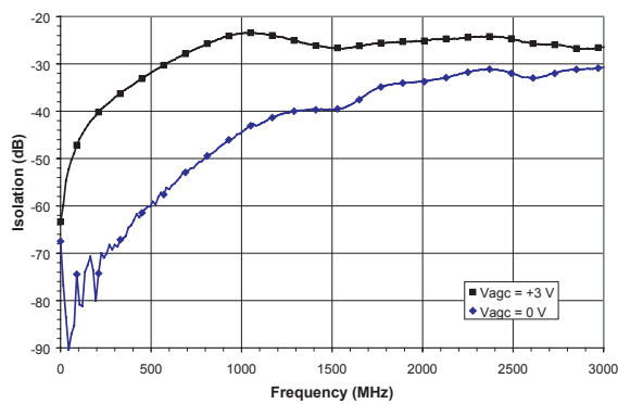
Figure 9: Output Port-to-Port Isolation vs. Frequency (TA = +25 °C, VCC = + 5 V, POUT = +6 dBmV)
