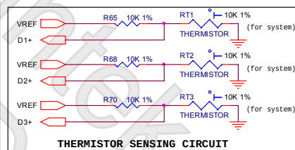
THERMISTOR SENSING CIRCUIT
