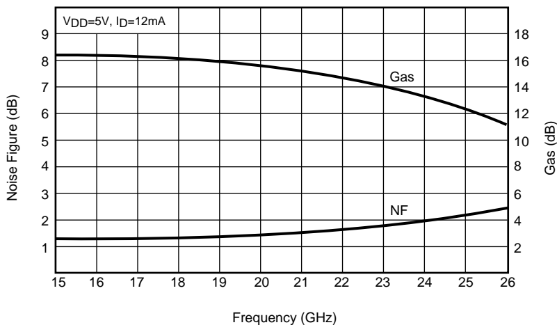
NF & Gas vs. FREQUENCY
