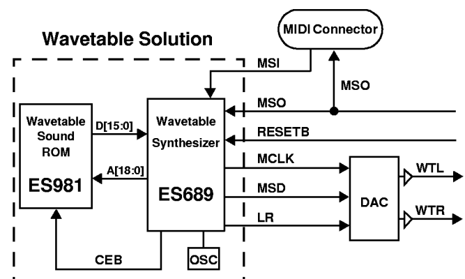
ES689 wavetable solution only
