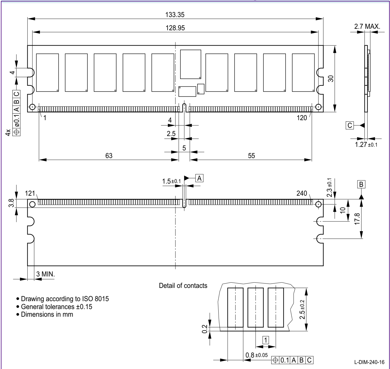
FIGURE 6 Package Outline Raw Card Z L-DIM-240-16
