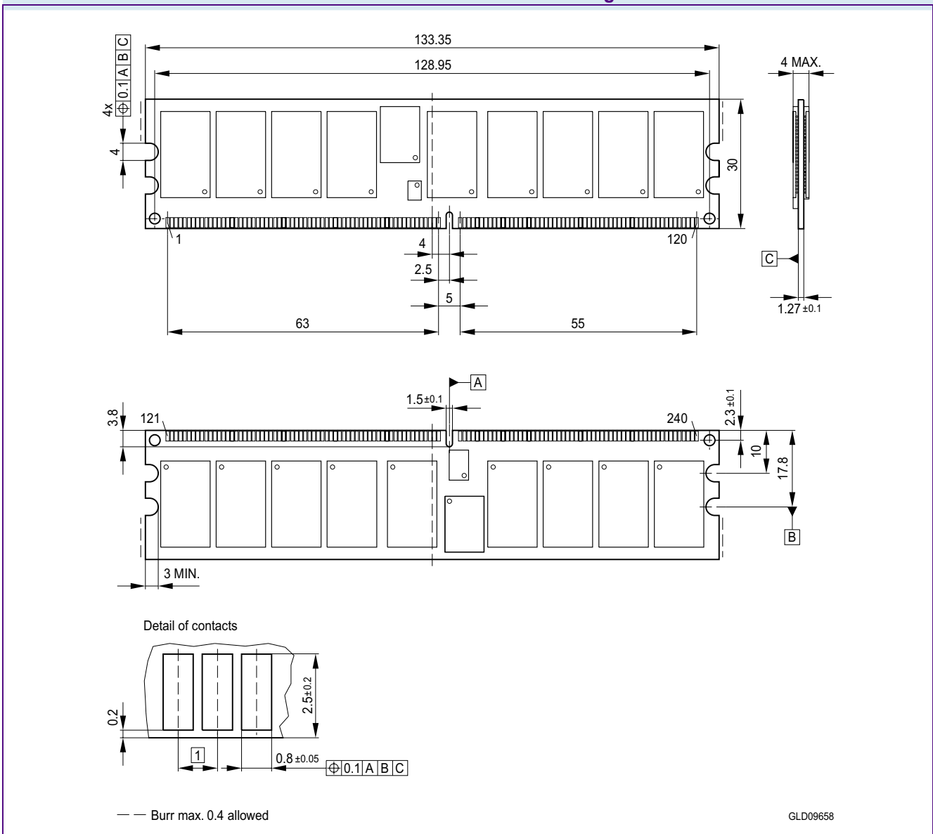
FIGURE 5 Package Outline Raw Card D L-DIM-240-15
