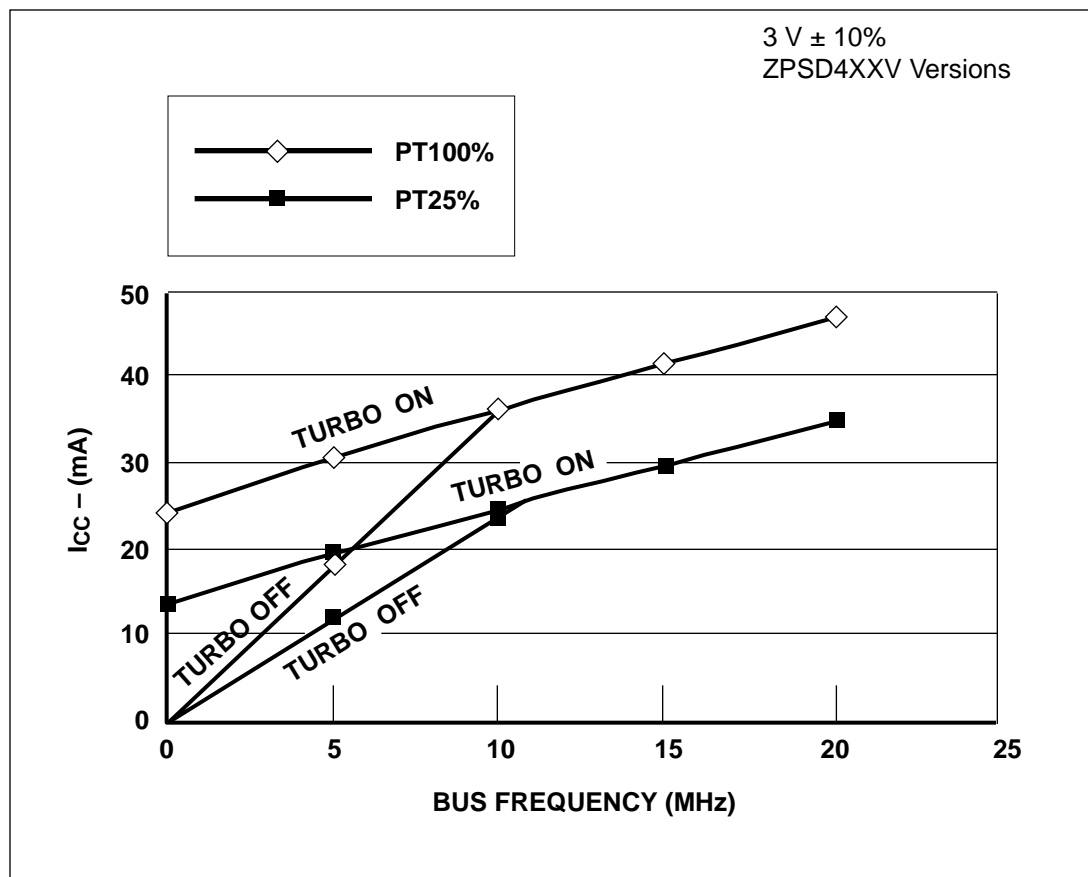
Figure 38c. ZPLD I_{CC} /Frequency Consumption
