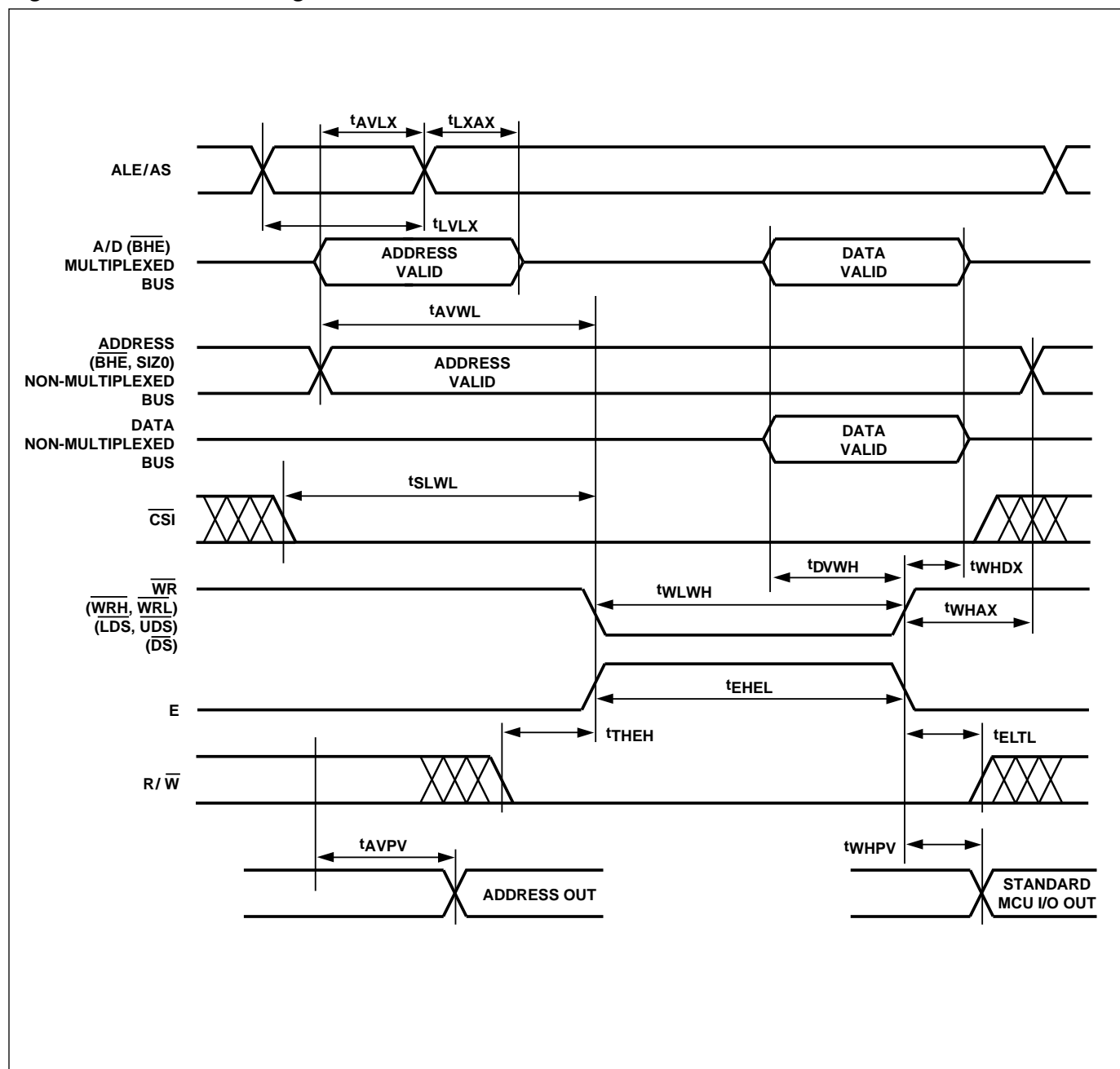
Figure 40. Write Timing
