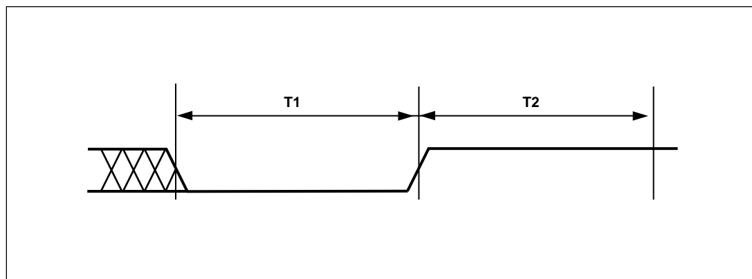
Figure 48. Reset Timing
