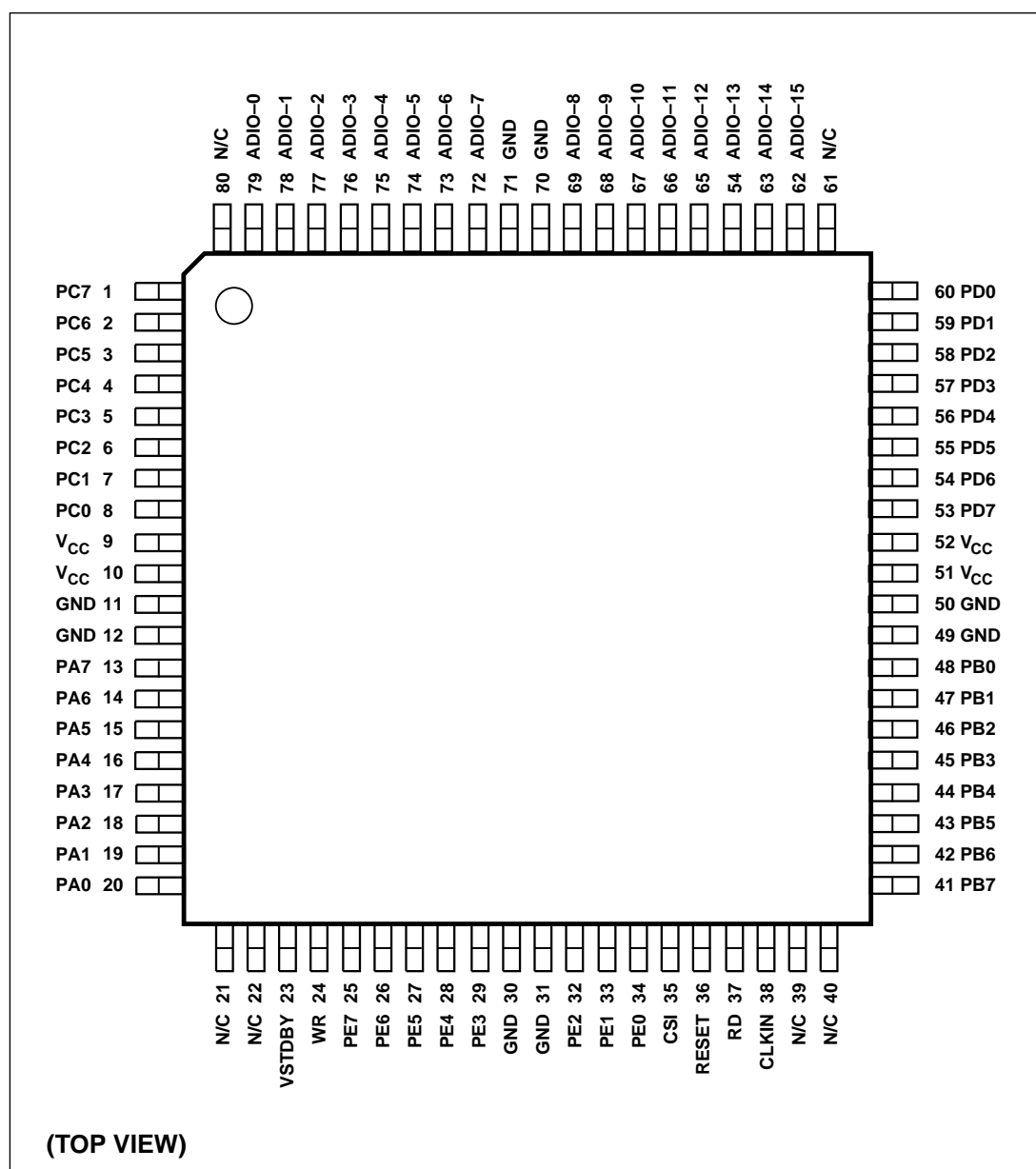
Figure 54. Drawing U2 D 80-Pin Plastic Thin Quad Flatpack (TQFP) (Package Type U)
