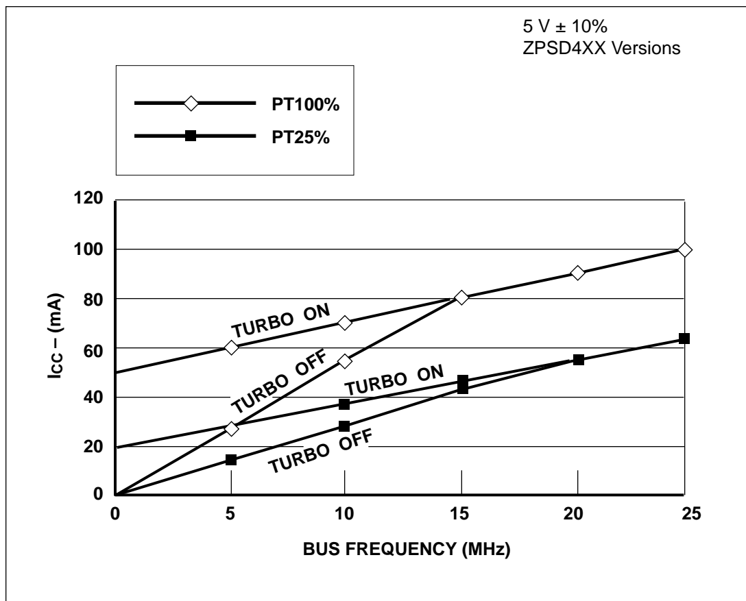
Figure 38b. ZPLD I_{CC} /Frequency Consumption
