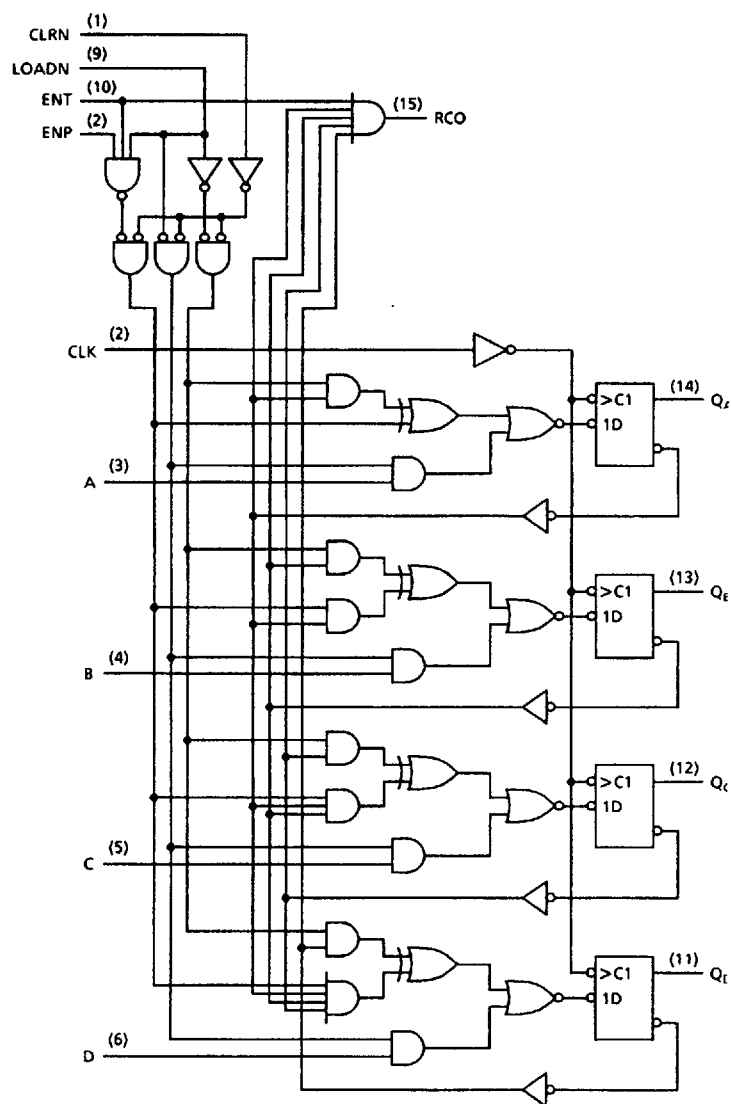
Figure 10: Logic Diagram
