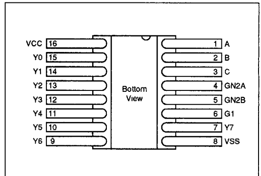
Figure 6: Flatpack Pin Out
