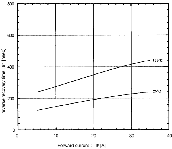
Reverse recovery time vs. Forward current -di/dt=75A / μsec
