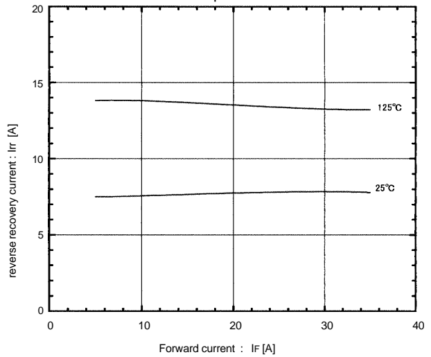
Reverse recovery current vs. Forward current -di/dt=75A / μsec
