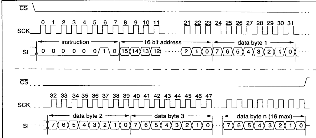
FIGURE 3-5: READ STATUS REGISTER SEQUENCE
