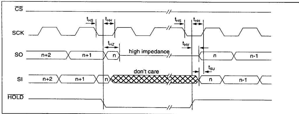
FIGURE 1-4: HOLD TIMING
