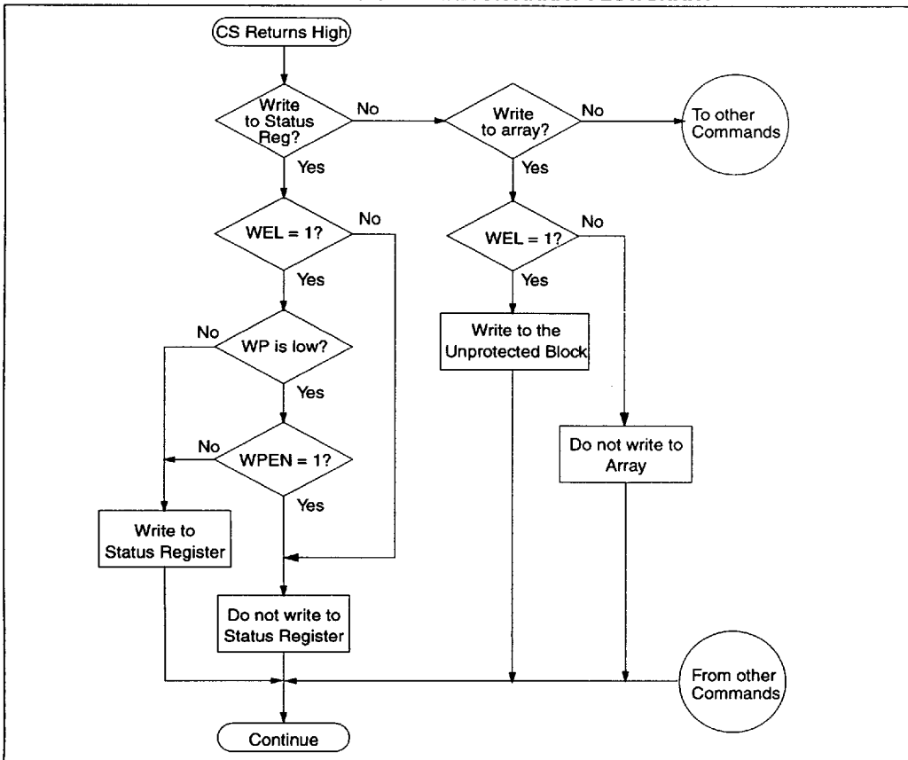
FIGURE 2-1: WRITE TO STATUS REGISTER AND/OR ARRAY FLOWCHART
