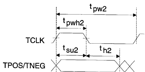
Figure 3a. Transmit Clock and Data Switching Characteristics
