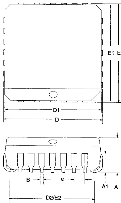
28-pin PLCC
