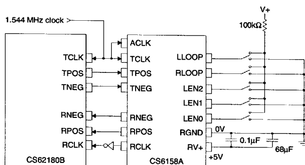
Figure A2. - Interfacing the CS6158A with a CS62180B
