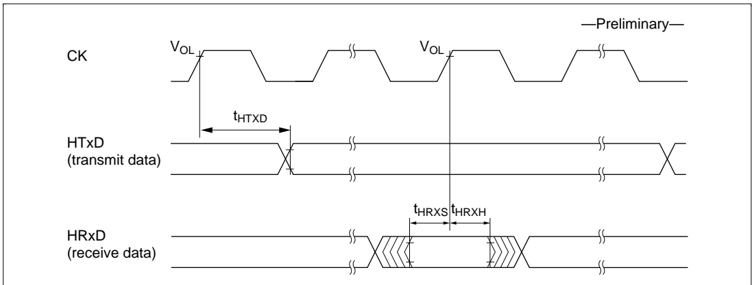
Figure 23-20 HCAN Input/Output Timing
