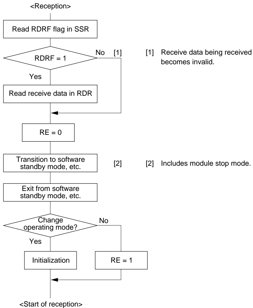
Figure 13-26 Sample Flowchart for Mode Transition during Reception
