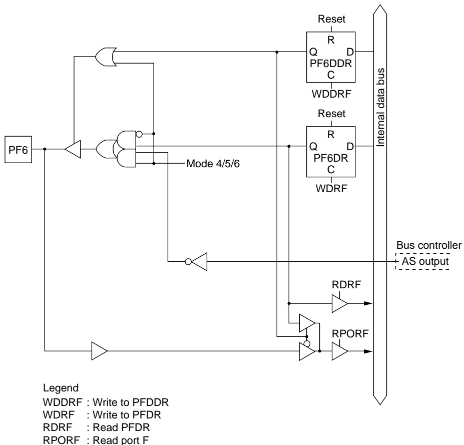
Figure C-12 (f) Port F Block Diagram (Pin PF6)
