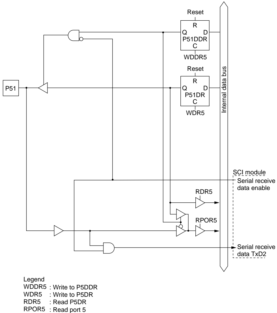
Figure C-5 (c) Port 5 Block Diagram (Pin P51) (H8S/2648, H8S/2648R, H8S/2647)
