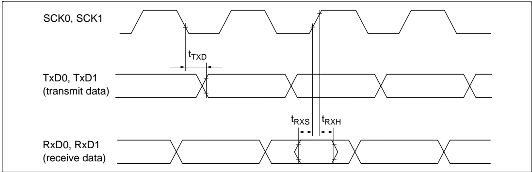
Figure 23-18 SCI Input/Output Timing (Clock Synchronous Mode)
