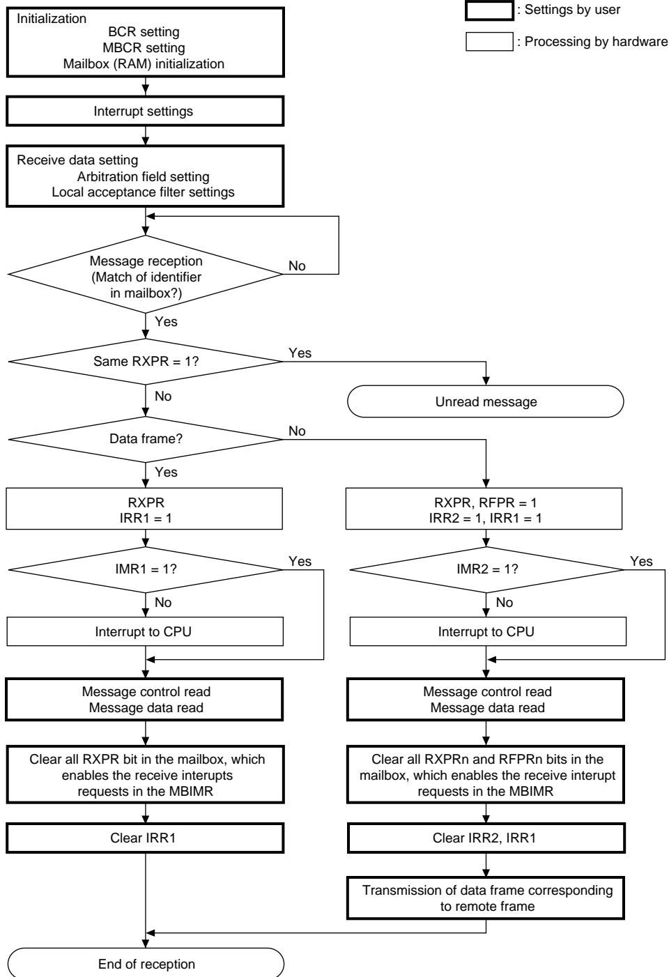
Figure 15-9 Reception Flowchart
