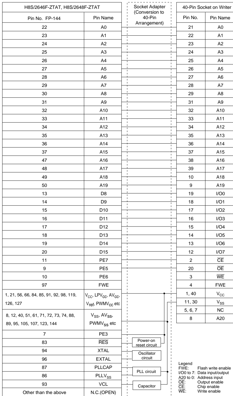
Figure 20-17 Socket Adapter Pin Correspondence Diagram
