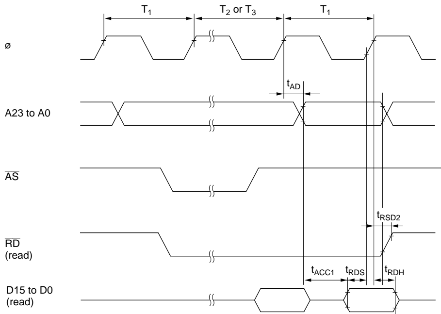
Figure 23-11 Burst ROM Access Timing (One-State Access)
