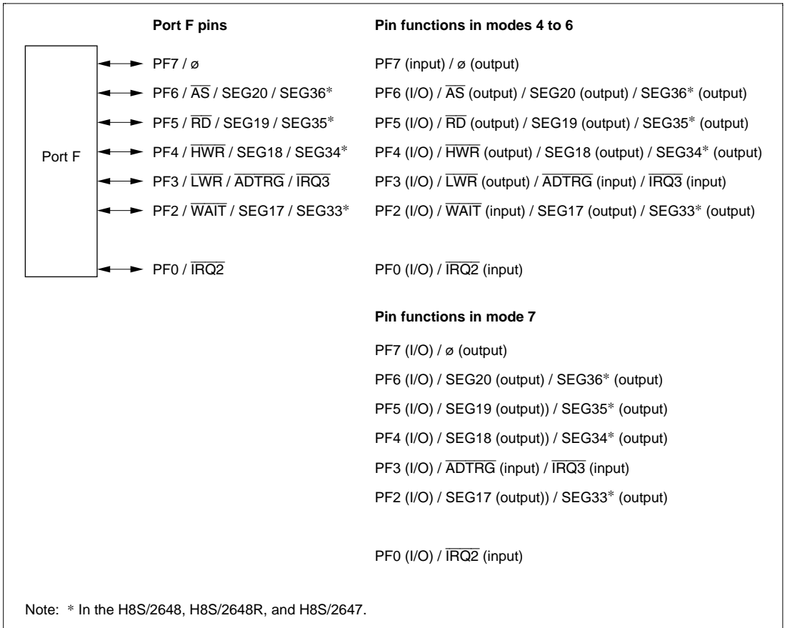
Figure 9-12 Port F Pin Functions
