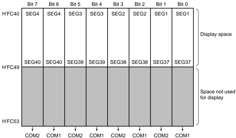
Figure 18-9 LCD RAM Map (1/2 Duty)
