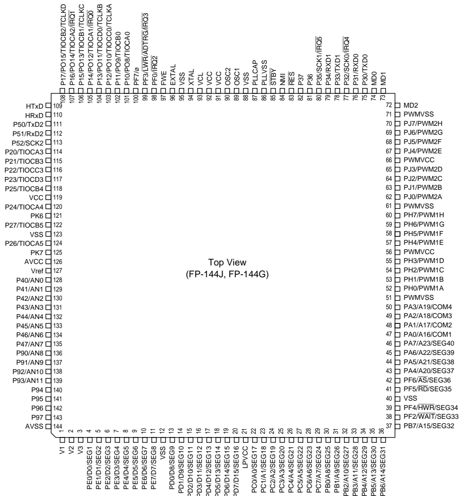
Figure 1-2 (2) H8S/2648, H8S/2648R, and H8S/2647 Pin Arrangement (FP-144J, FP-144G: Top View)
