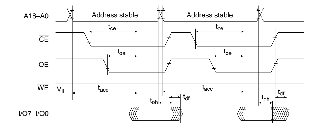
Figure 20-21 \overline{CE} and \overline{OE} Clock System Read Timing Waveforms
