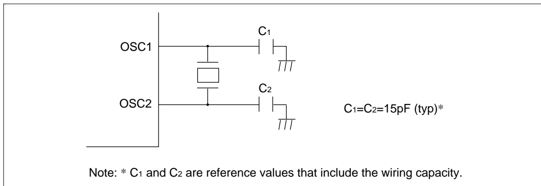
Figure 21-6 Example Connection of 32.768kHz Quartz Oscillator
