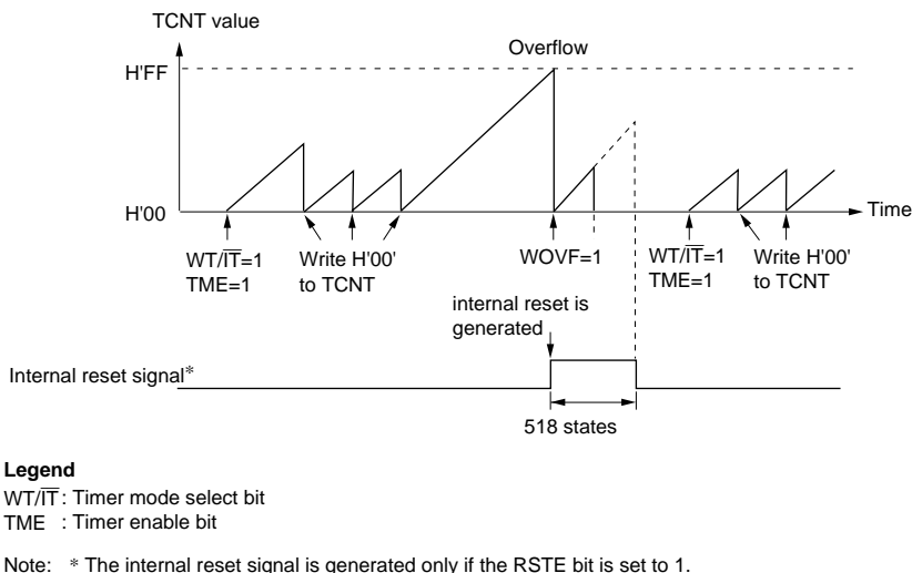
Figure 12-4 (a) WDT0 Watchdog Timer Operation
