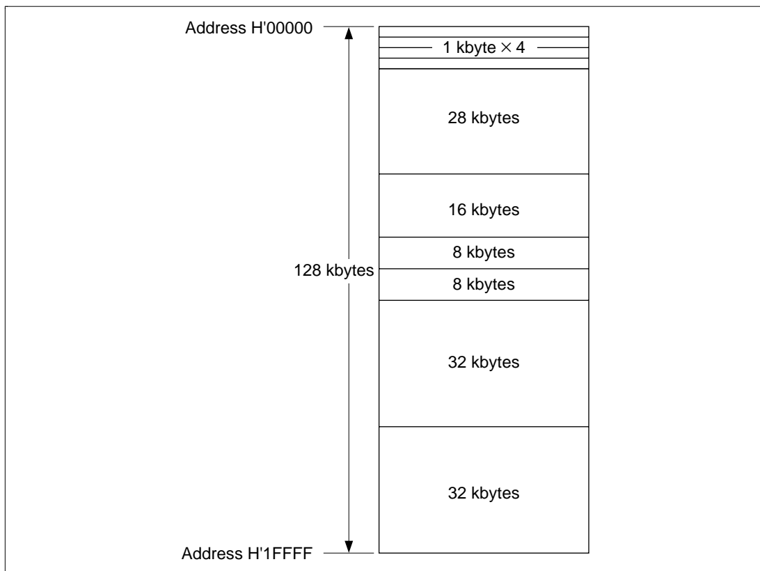
Figure 20-5 Block Configuration
