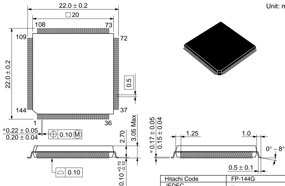
Figure F-2 FP-144G Package Dimension (H8S/2646, H8S/2645, H8S/2648, H8S/2647)
