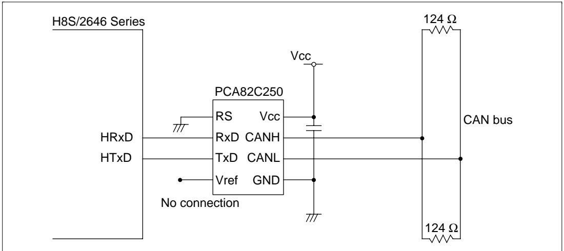
Figure 15-14 High-Speed Interface Using PCA82C250
