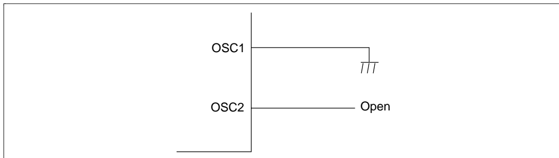
Figure 21-8 Pin Handling When Subclock Not Required
