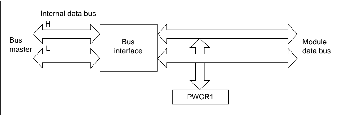
Figure 17-9 8-Bit Register Access Operation (Bus Master ↔ PWCR1 (Upper 8 Bits))
