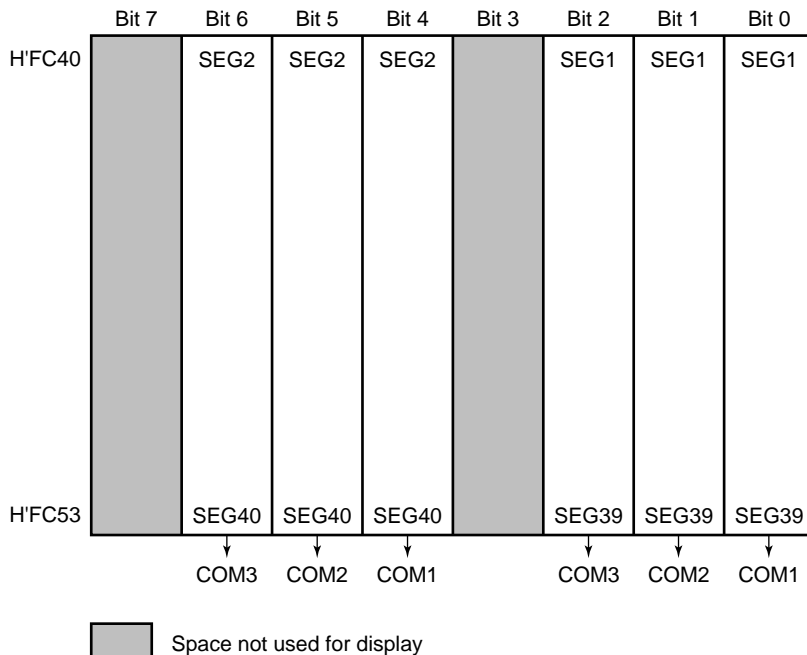
Figure 18-8 LCD RAM Map (1/3 Duty)
