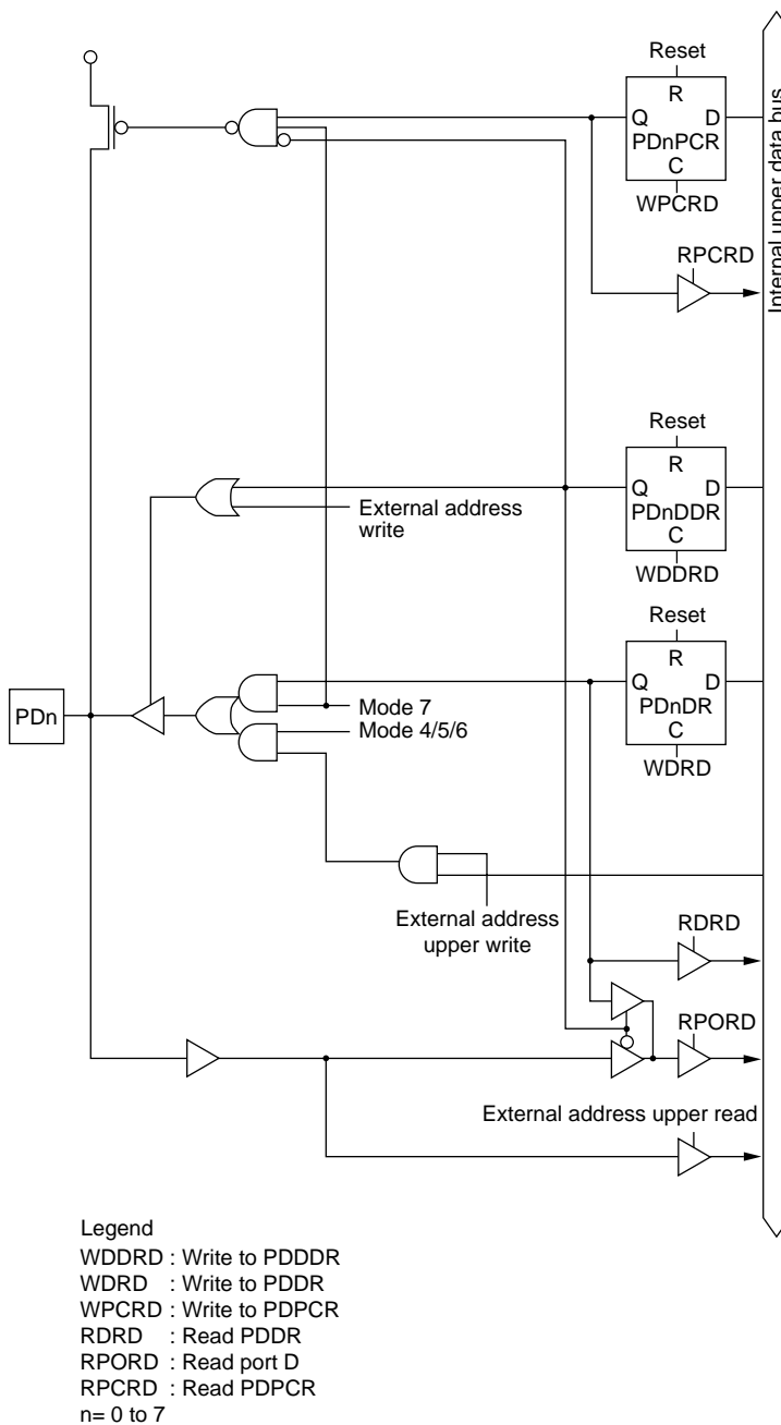
Figure C-10 Port D Block Diagram (Pins PD0 to PD7)
