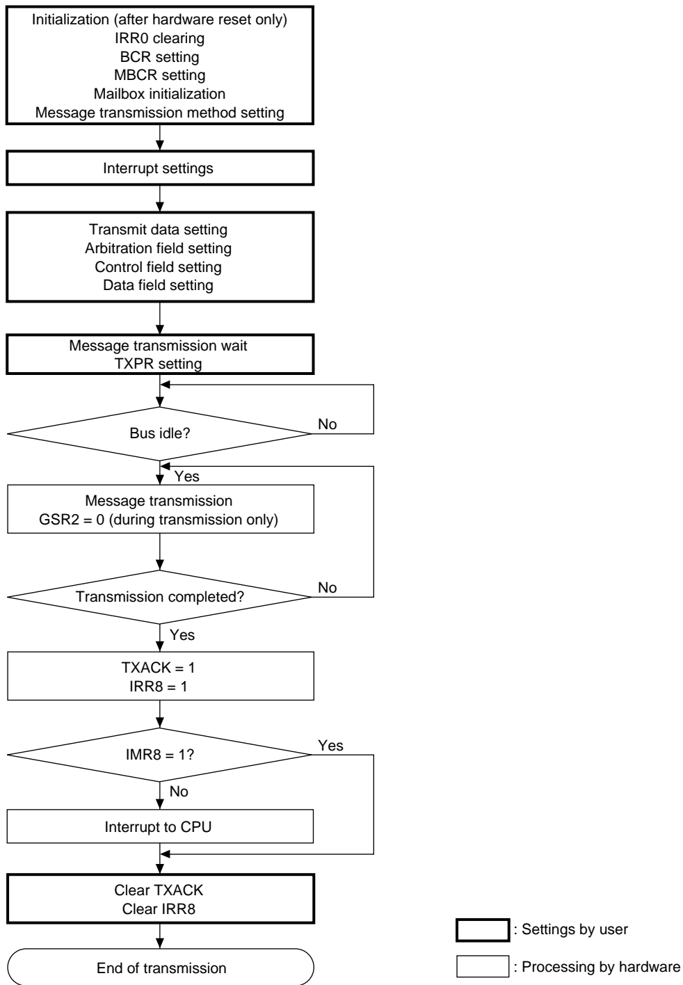
Figure 15-7 Transmission Flowchart
