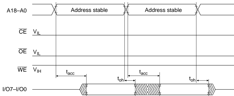
Figure 20-20 \overline{CE} and \overline{OE} Enable State Read Timing Waveforms
