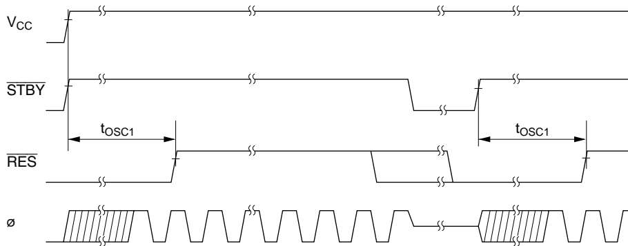
Figure 23-4 Oscillator Settling Timing
