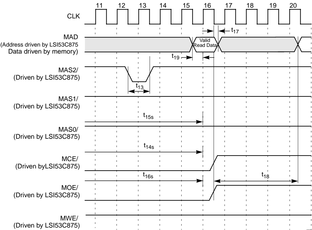
Figure 7.25 Read Cycle, Slow Memory ( \geq 64 Kbyte) (Cont.)
