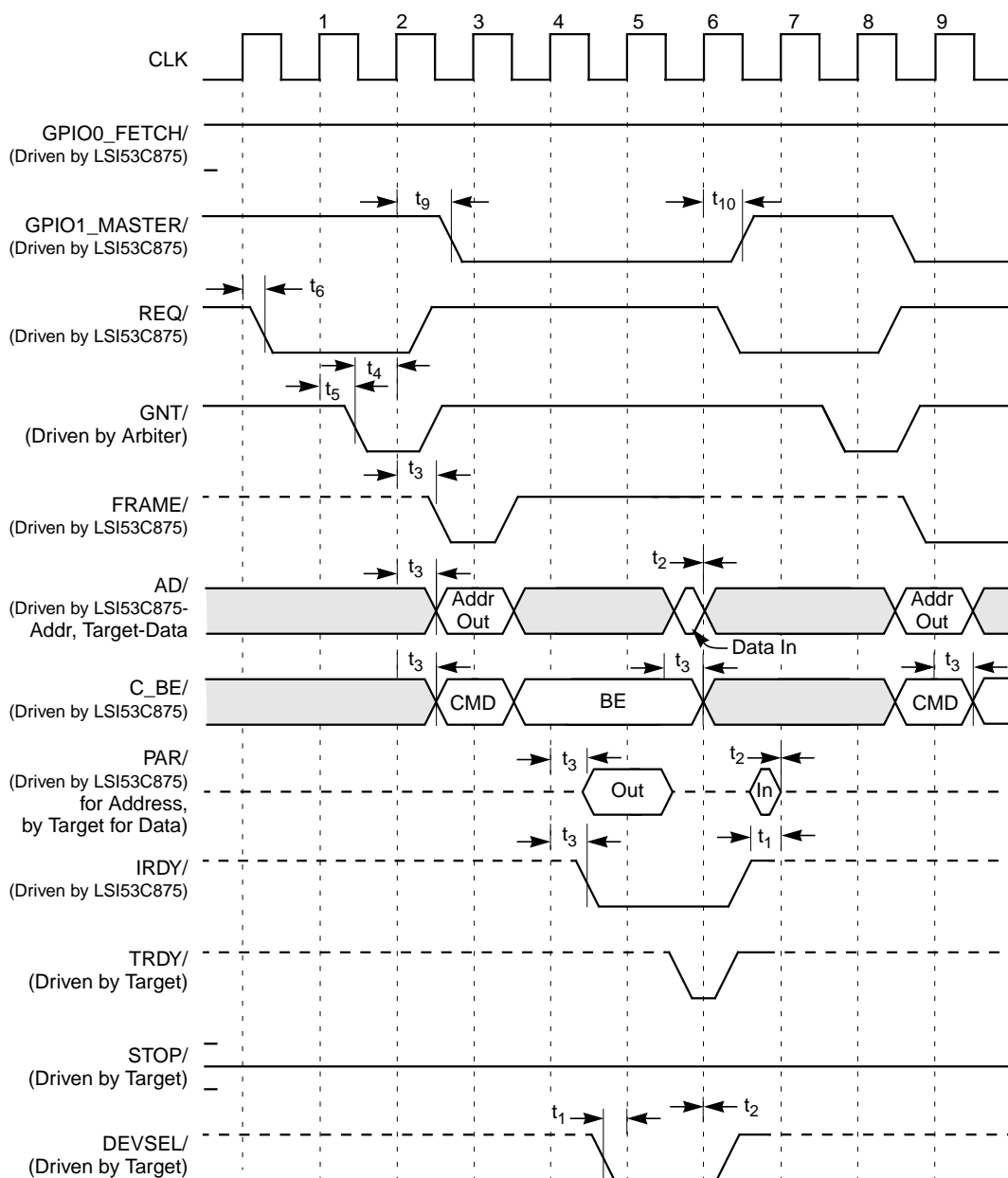
Figure 7.19 Burst Read
