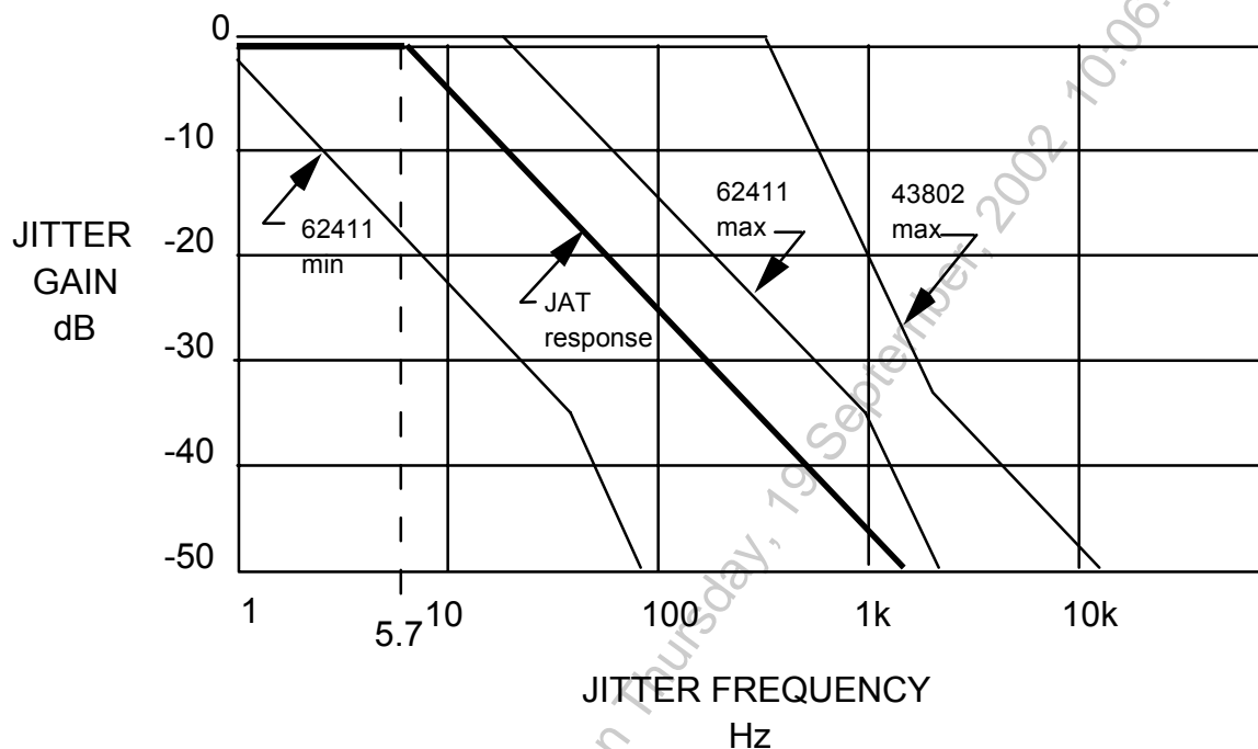
Figure 10 – TJAT Jitter Transfer
