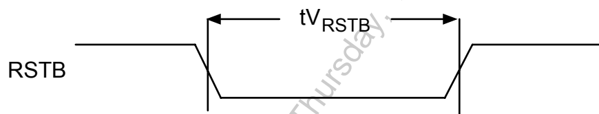
Figure 28 – RSTB Timing
