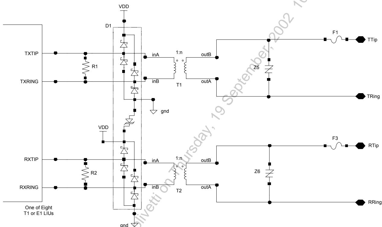
Figure 11 – External Analogue Interface Circuits
