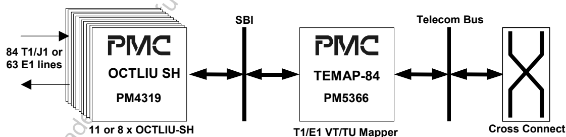
Figure 3 – Metro Optical Access Equipment
