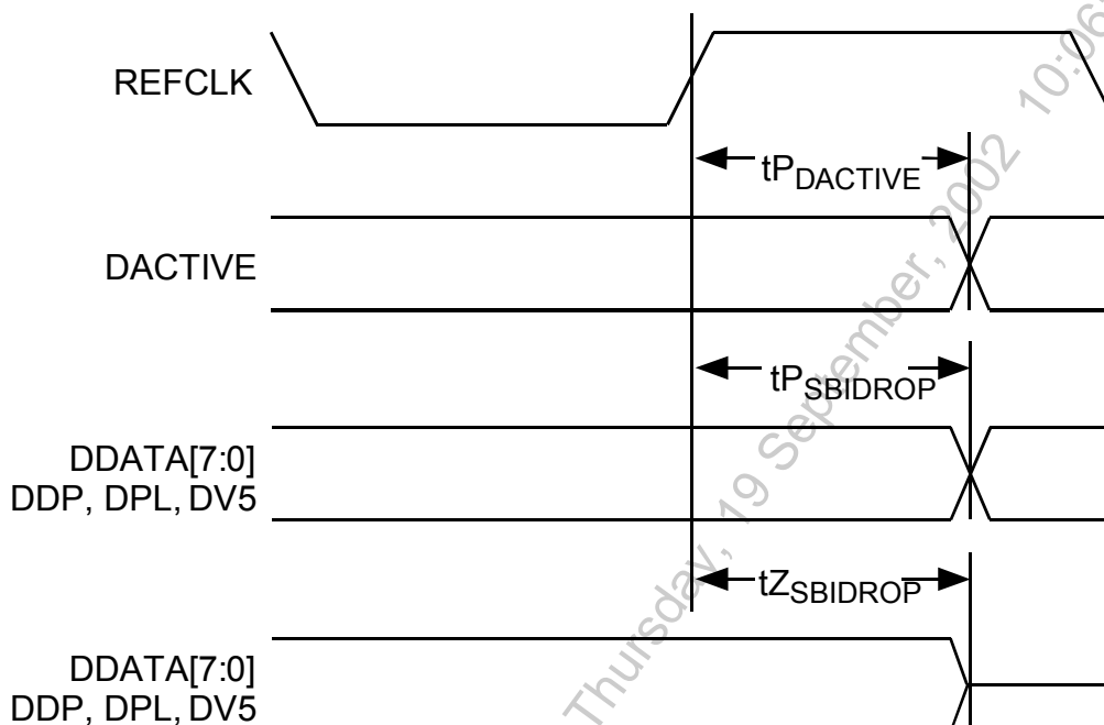
Figure 32 – SBI DROP BUS Timing
