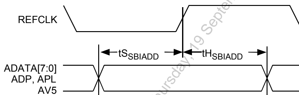
Figure 31 – SBI ADD BUS Timing
