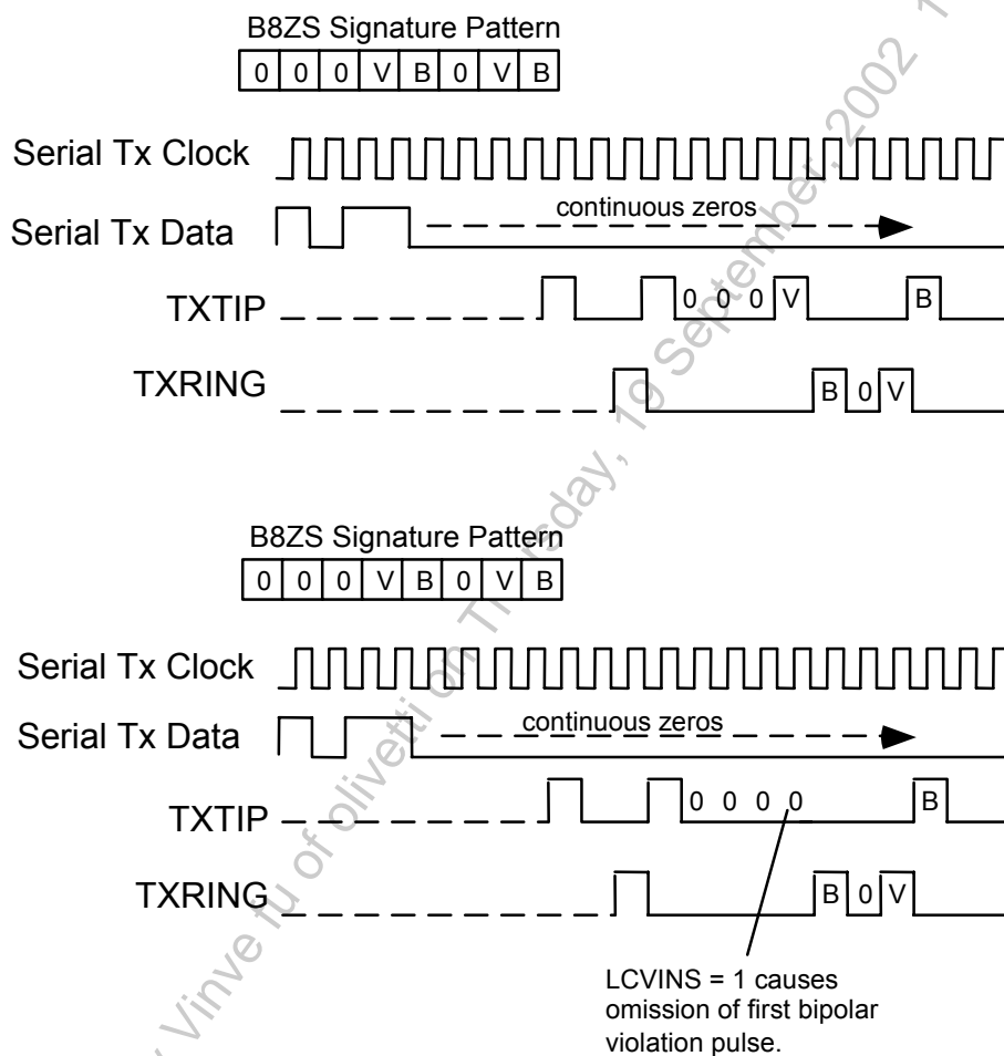
Figure 22 – B8ZS Line Code Violation Insertion
