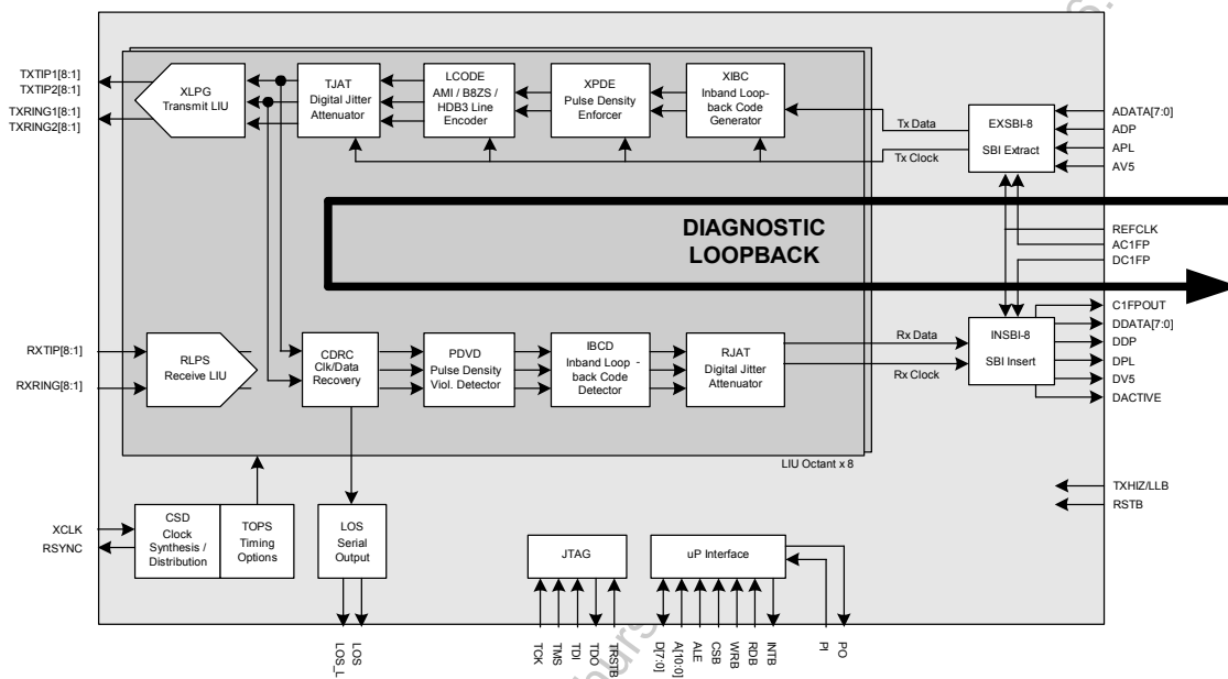
Figure 14 – Diagnostic Digital Loopback
