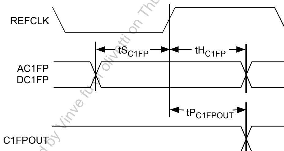
Figure 30 – SBI Frame Pulse Timing
