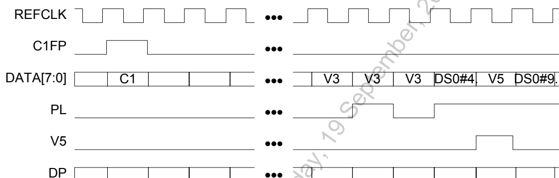
Figure 21 – SBI BUS Functional Timing
