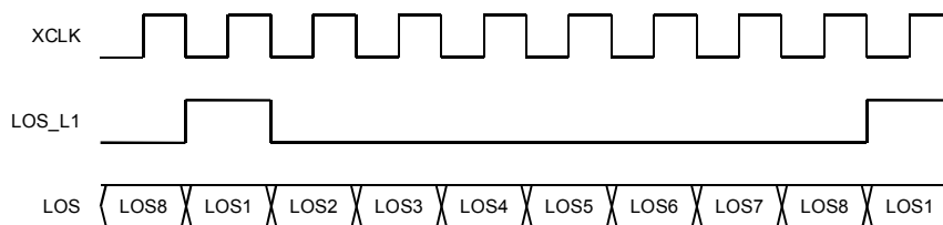
Figure 25 – LOS Alarm Serial Output
