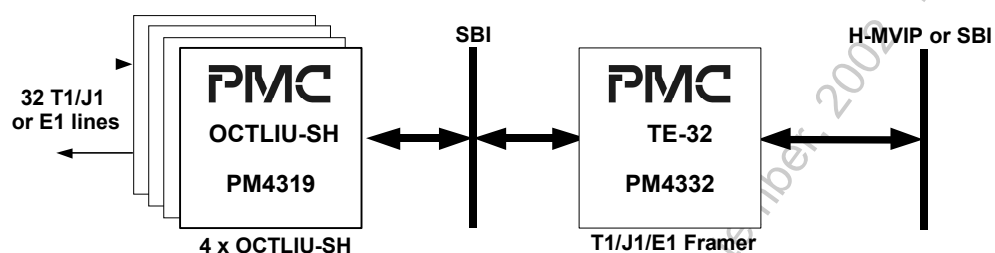
Figure 1 – High Density T1/E1 Framer/Transceiver Application
