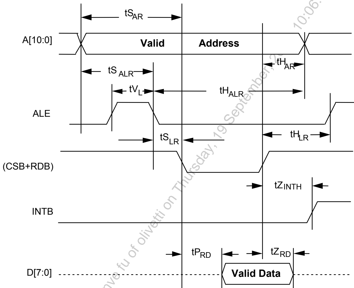
Figure 26 – Microprocessor Interface Read Timing
