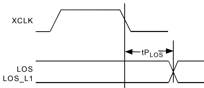
Figure 33 – Alarm Interface Timing
