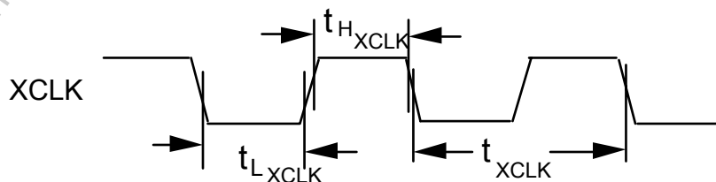
Figure 29 – XCLK Input Timing
