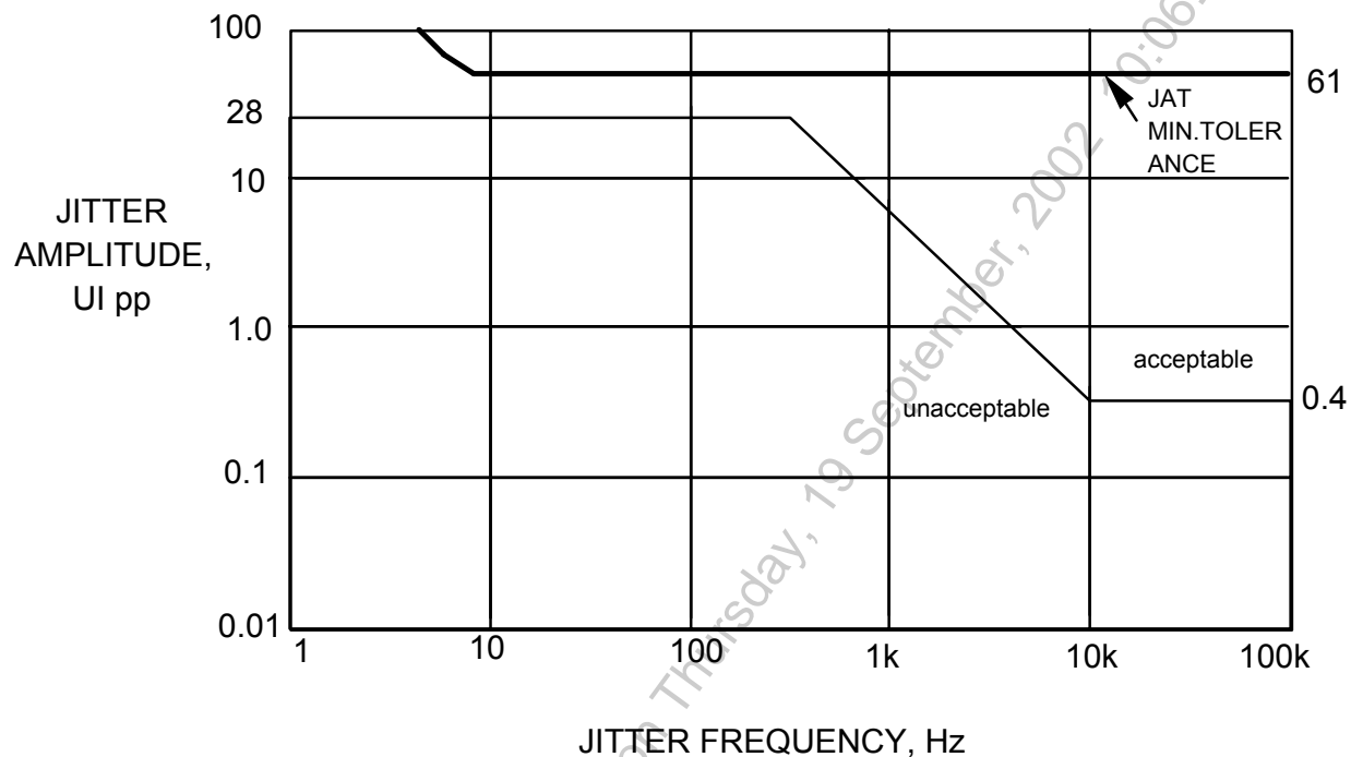
Figure 8 – TJAT Jitter Tolerance
