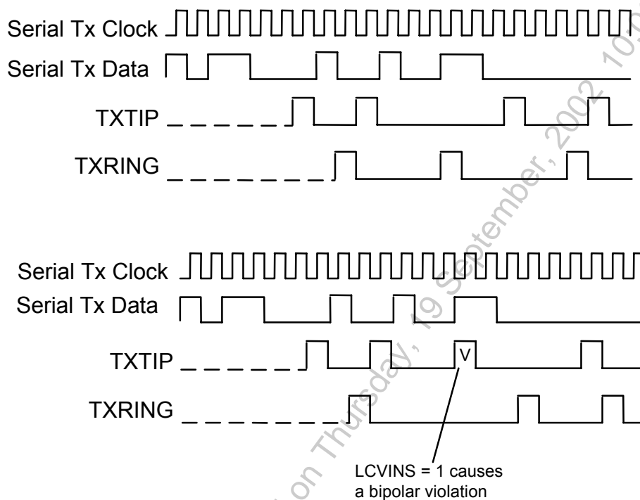
Figure 24 – AMI Line Code Violation Insertion
