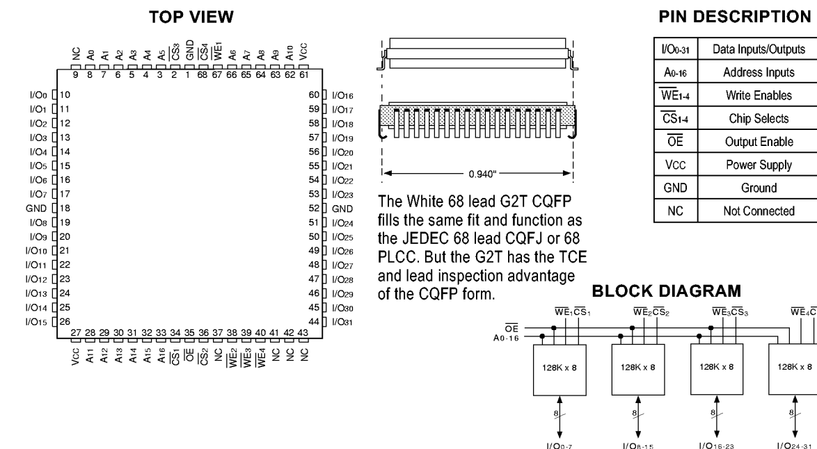
FIG. 3 PIN CONFIGURATION FOR WS128K32-XG2TX
