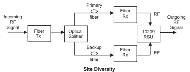
Figure 1. 10209-Type Redundancy Switch Unit Application Configurations
