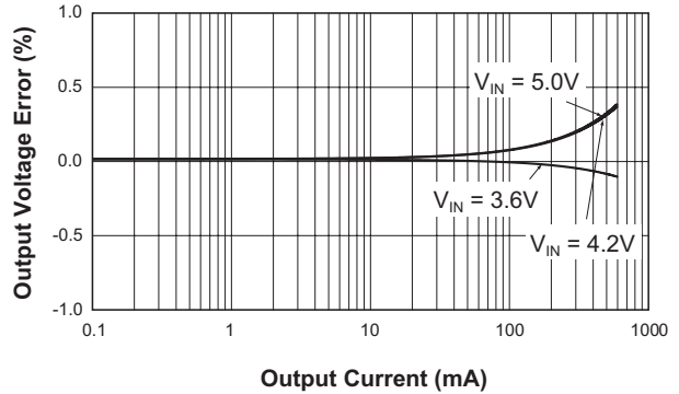
Load Regulation (PWM Mode; V_{OUT} = 3.3V )
