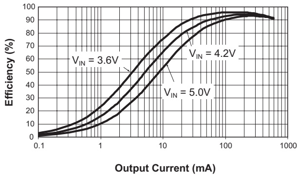
Efficiency vs. Output Current (PWM Mode; V_{OUT} = 3.3V )
