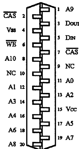
20 ZIP
