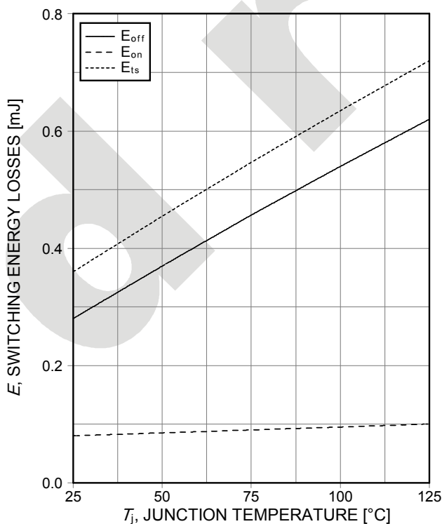
Figure 3. Typical switching energy losses as a function of junction temperature (ind load, V_{CE}=800\text{V} , V_{GE}=15/0\text{V} , I_C=10\text{A} , R_G=3\Omega , Diode IDH15S120)
