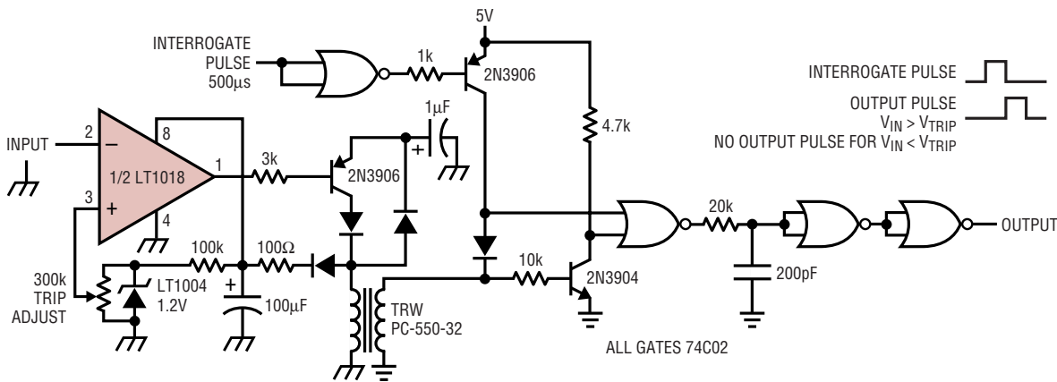
Fully Isolated Limit Comparator
