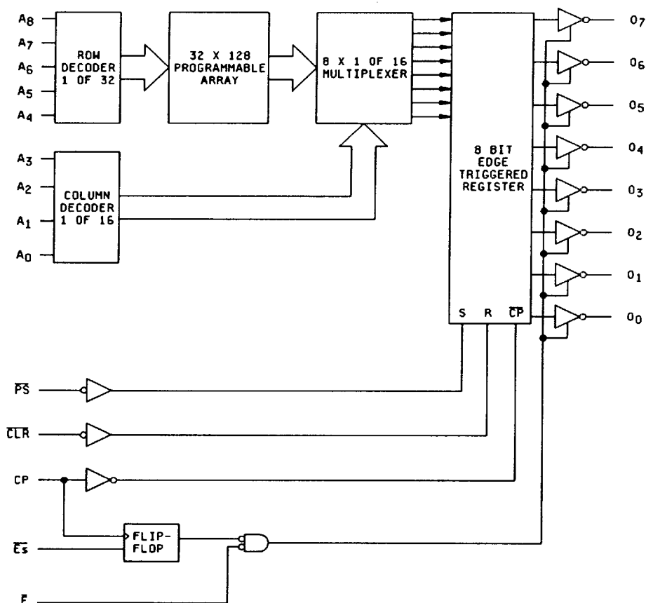
FIGURE 3. Logic diagram
