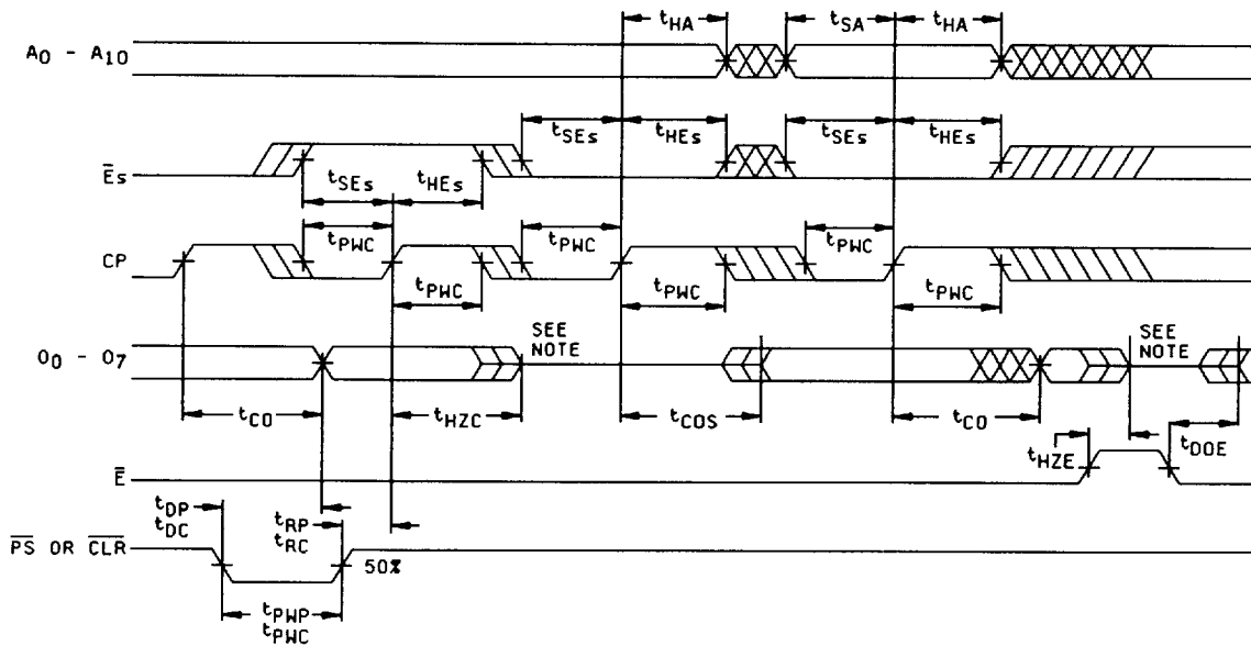
FIGURE 5. Switching waveforms.
