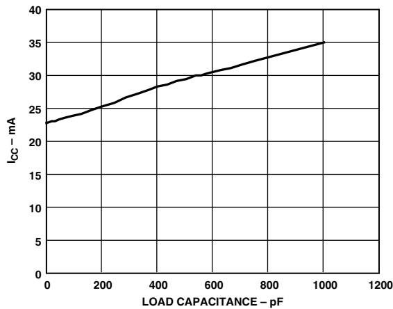
TPC 8. Supply Current vs. Load Capacitance ( R_L = 3\text{ k}\Omega )
