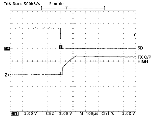
TPC 11. Transmitter Output (High) Exiting Shutdown
