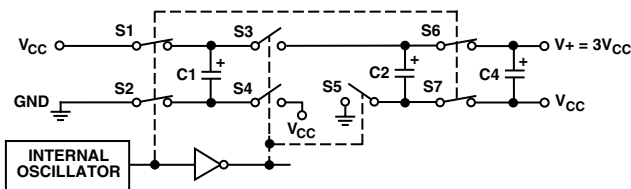
Figure 13. Charge Pump Voltage Tripler
