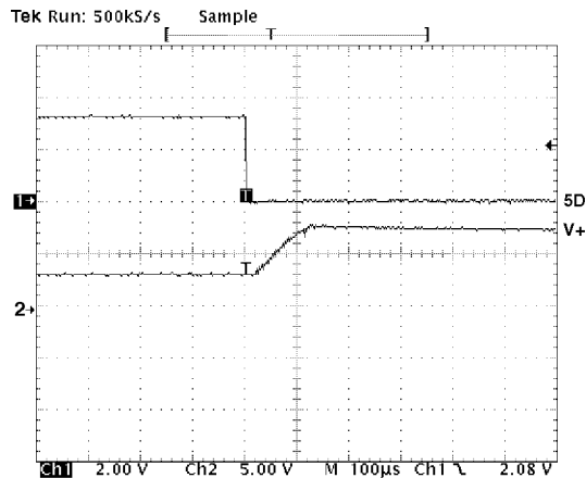
TPC 14. Charge Pump V+ Exiting Shutdown
