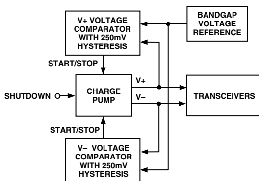
Figure 3. Block Diagram of Green Idle Circuit
