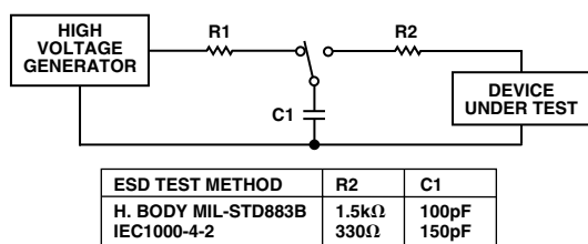
Figure 8. ESD Test Standards
