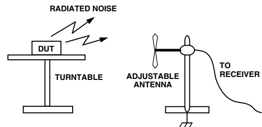
Figure 16. Radiated Emissions Test Setup
