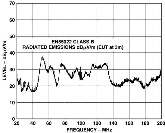
Figure 17. Radiated Emissions Plot
