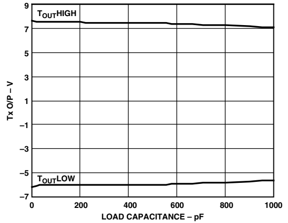
TPC 4. Tx Output vs. Load Capacitance
