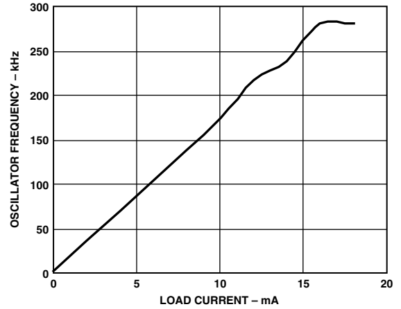
TPC 10. Oscillator Frequency vs. Load Current
