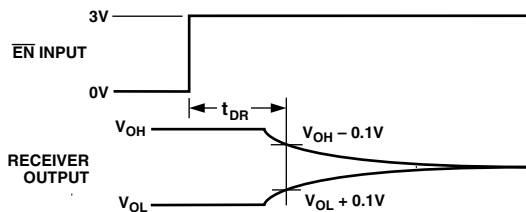
Figure 5. Receiver Disable Timing
