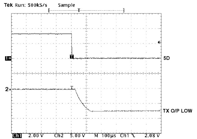
TPC 12. Transmitter Output (Low) Exiting Shutdown
