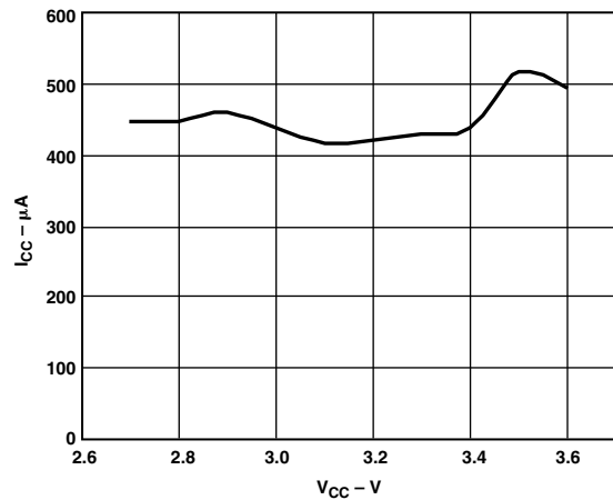
TPC 5. I_{CC} vs. V_{CC} (Unloaded)
