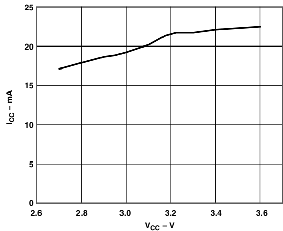
TPC 6. I_{CC} vs. V_{CC} ( R_L = 3\text{ k}\Omega )
