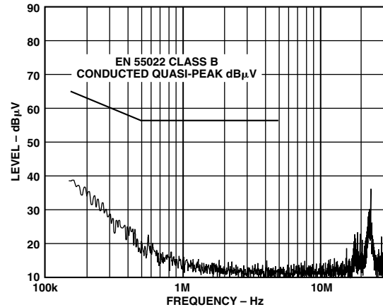
Figure 15. Conducted Emissions Plot
