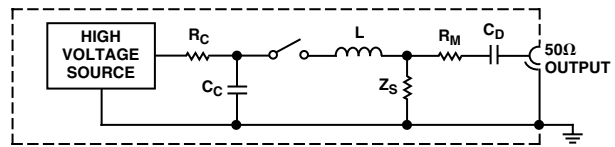
Figure 12. IEC1000-4-4 Fast Transient Generator
