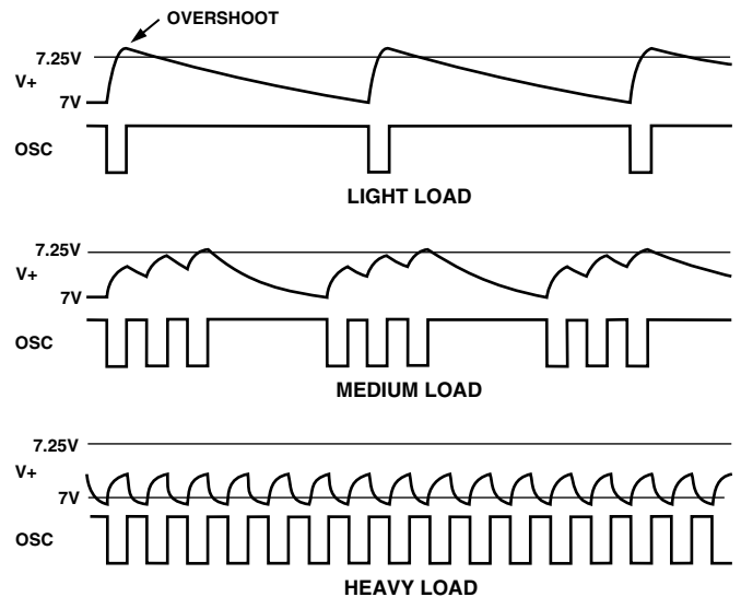
Figure 4. Operation of Green Idle Under Various Load Conditions
