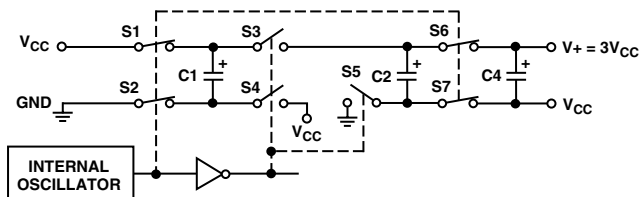
Figure 1. Charge Pump Voltage Tripler
