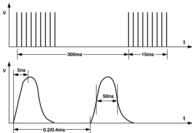
Figure 11. IEC1000-4-4 Fast Transient Waveform
