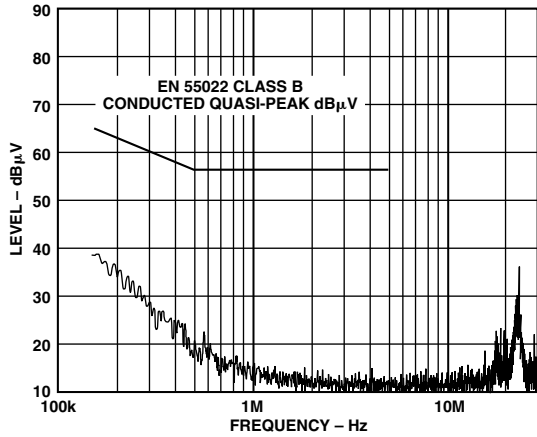
TPC 1. EMC Conducted Emissions
