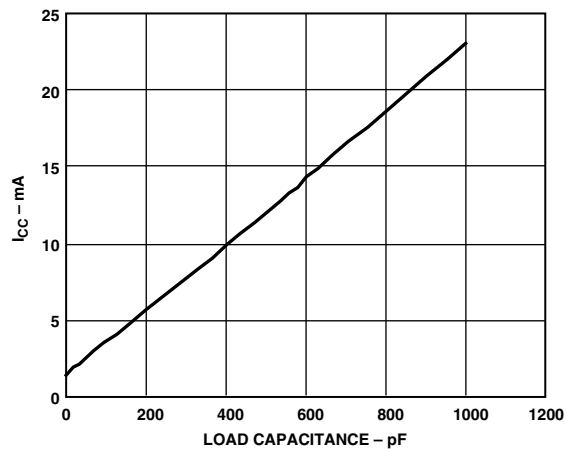
TPC 9. Supply Current vs. Load Capacitance ( R_L = \infty )
