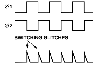
Figure 14. Switching Glitches
