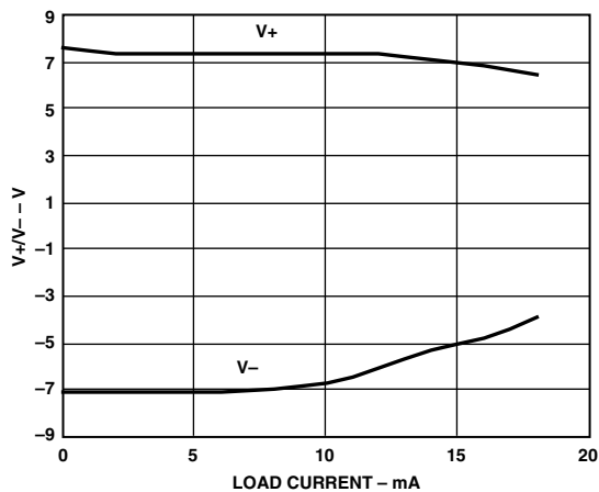
TPC 3. Charge Pump V_+ , V_- vs. Load Current
