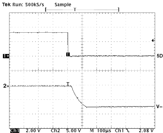
TPC 13. Charge Pump V- Exiting Shutdown
