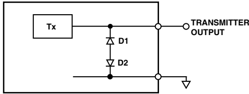
Figure 7b. Transmitter Output Protection Scheme
