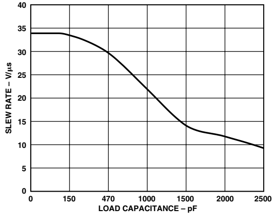
TPC 7. Slew Rate vs. Load Capacitance
