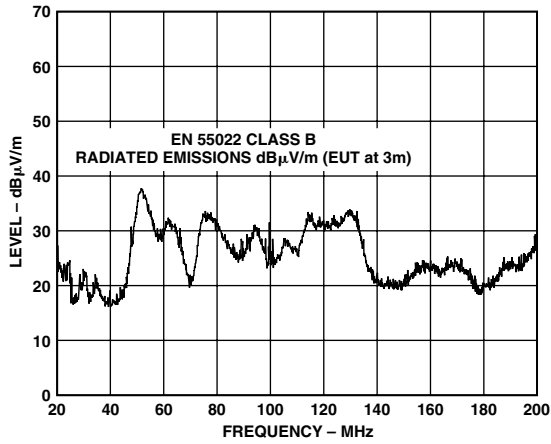
TPC 2. EMC Radiated Emissions
