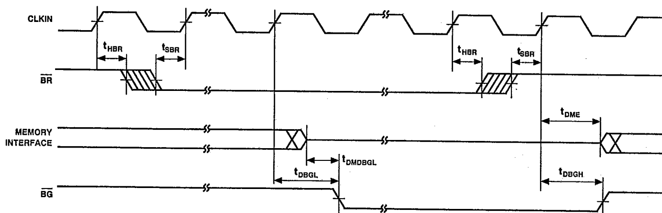
Figure 8. Bus Request/Bus Grant
