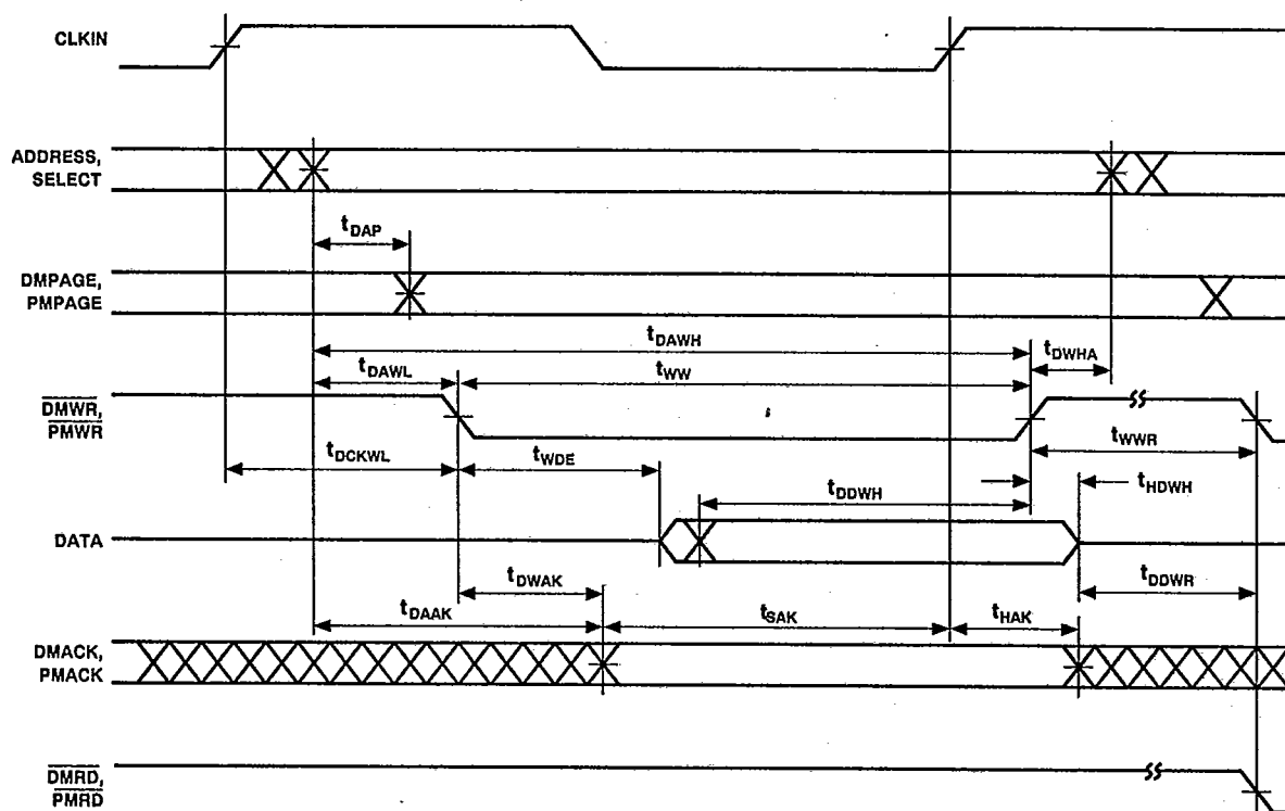
Figure 11. Memory Write
