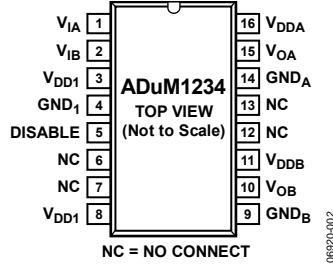
Figure 2. Pin Configuration
