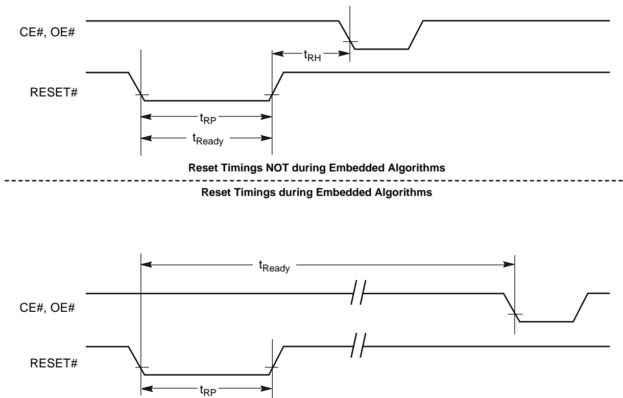
Figure 17. Reset Timings
