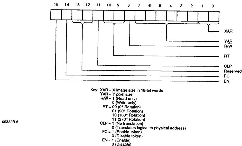
Figure 1. Control Status Register Format
