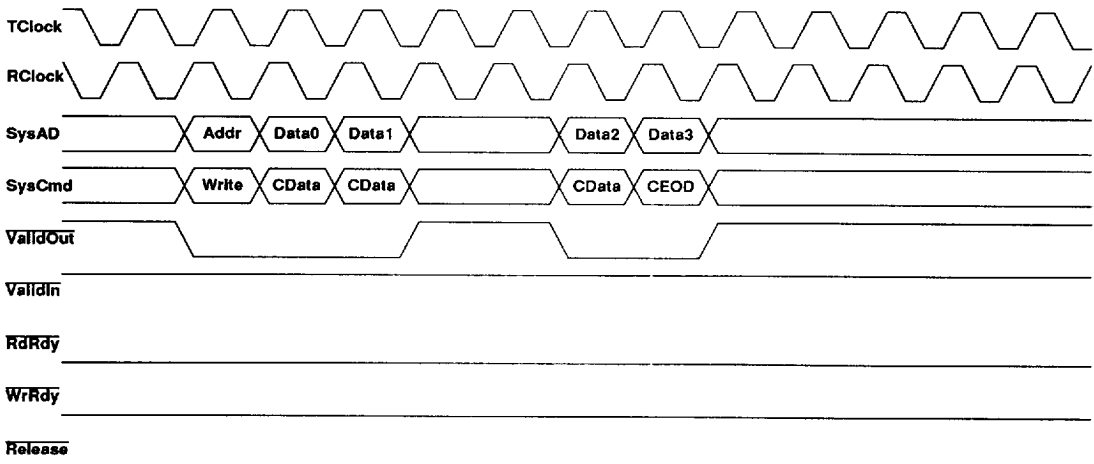
Figure 7. Processor Block Write
