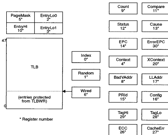
Figure 3. The R4600 CP0 Registers
