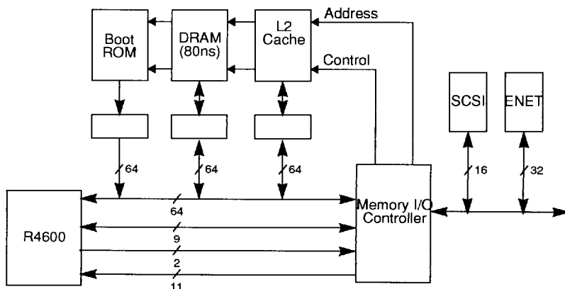
Figure 5. Typical Desktop System Block Diagram
