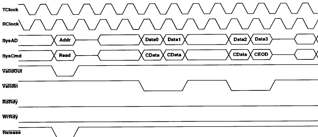
Figure 6. Processor Block Read
