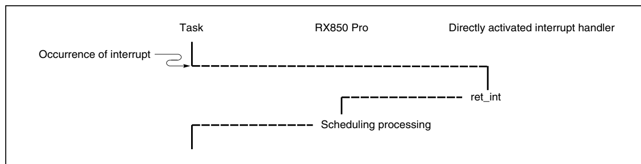
Figure 5-1. Flow of Processing Performed by Directly Activated Interrupt Handler
