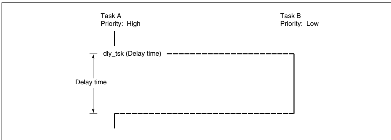
Figure 7-1. Flow of Processing After Issuance of dly_tsk
