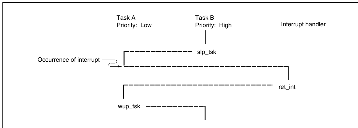
Figure 8-5. Flow of Control if Scheduling Processing Is Not Delayed (Normal)
