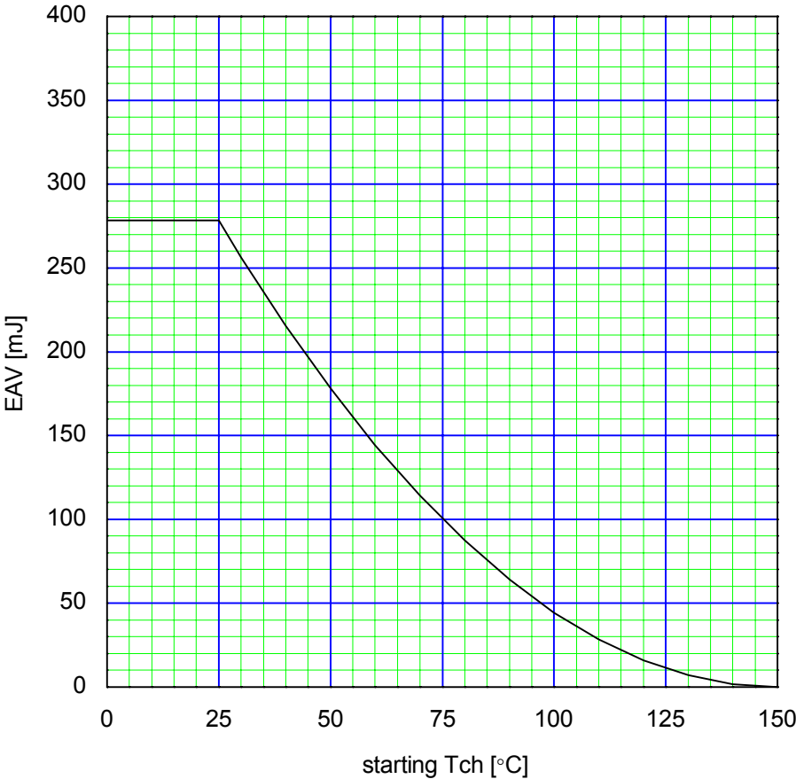
Maximum Avalanche Energy vs. starting Tch E(AV)=f(\text{starting Tch}):V_{CC}=48V, I(AV)\leq 30A
