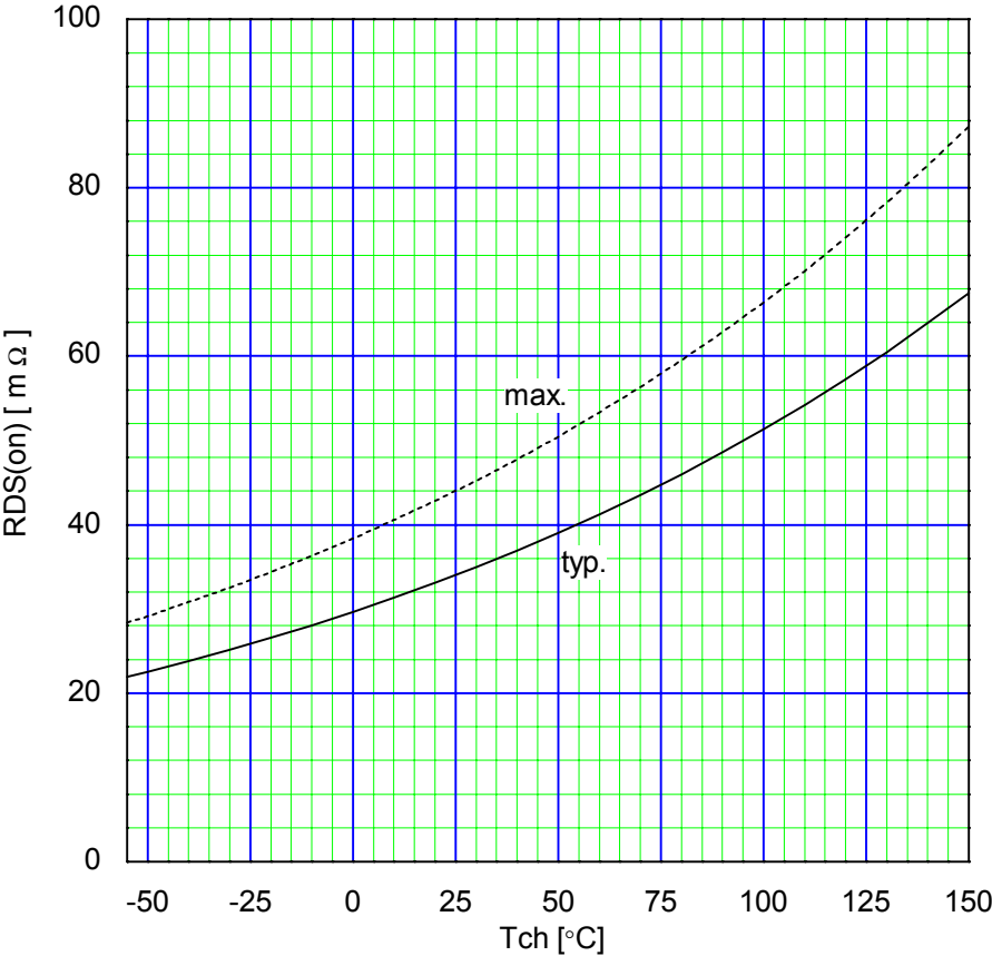
Drain-Source On-state Resistance R_{DS(on)}=f(T_{ch}):I_D=15\text{A}, V_{GS}=10\text{V}
