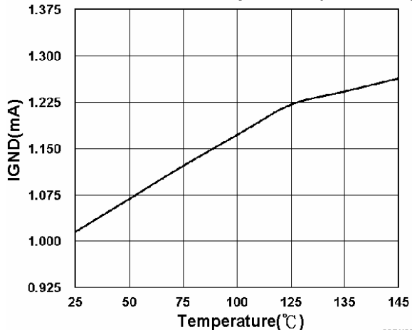
Ground Current Vs Temperature (VSD=VIN)
