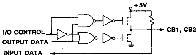
c. Port B Control Line Output Circuit
