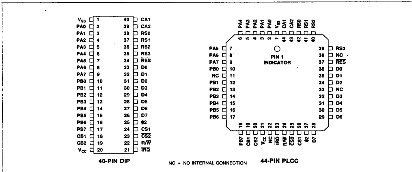
Figure 1. R65NC22 Pin Assignments
