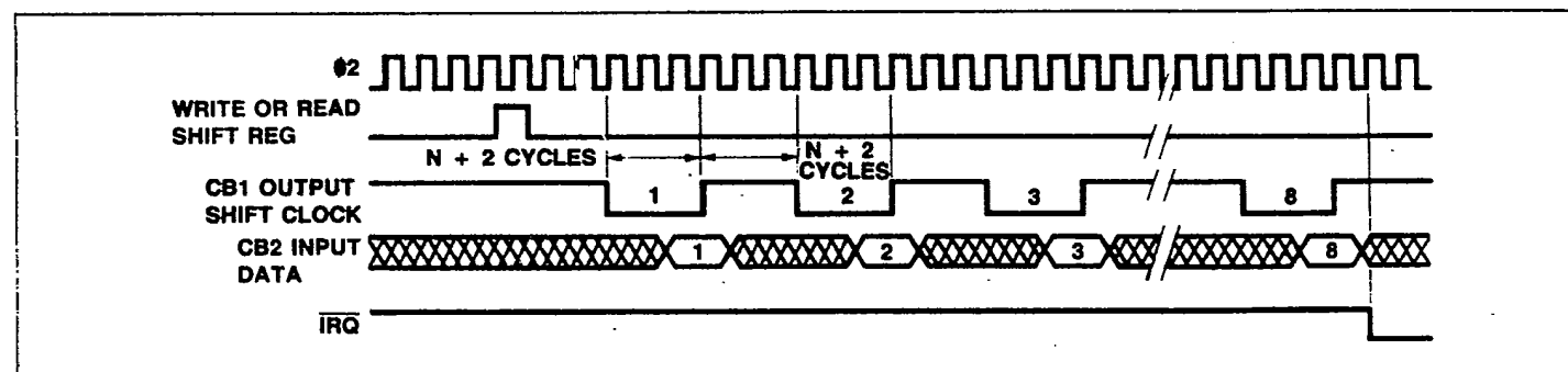
Figure 22. SR Mode 1 — Shift In Under T2 Control
