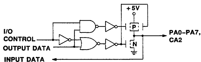
a. Port A Data and Control Line Output Circuit
