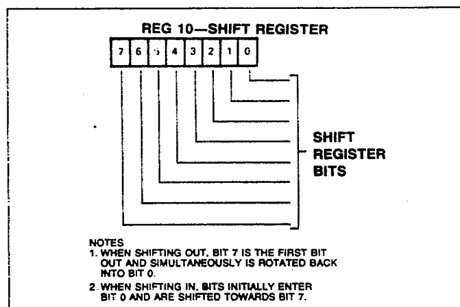
Figure 20. Shift Register
