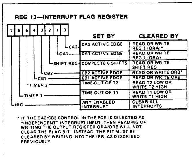
Figure 29. Interrupt Flag Register (IFR)
