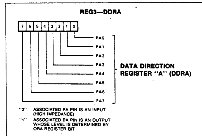
Figure 8. Data Direction Register A (DDRA)
