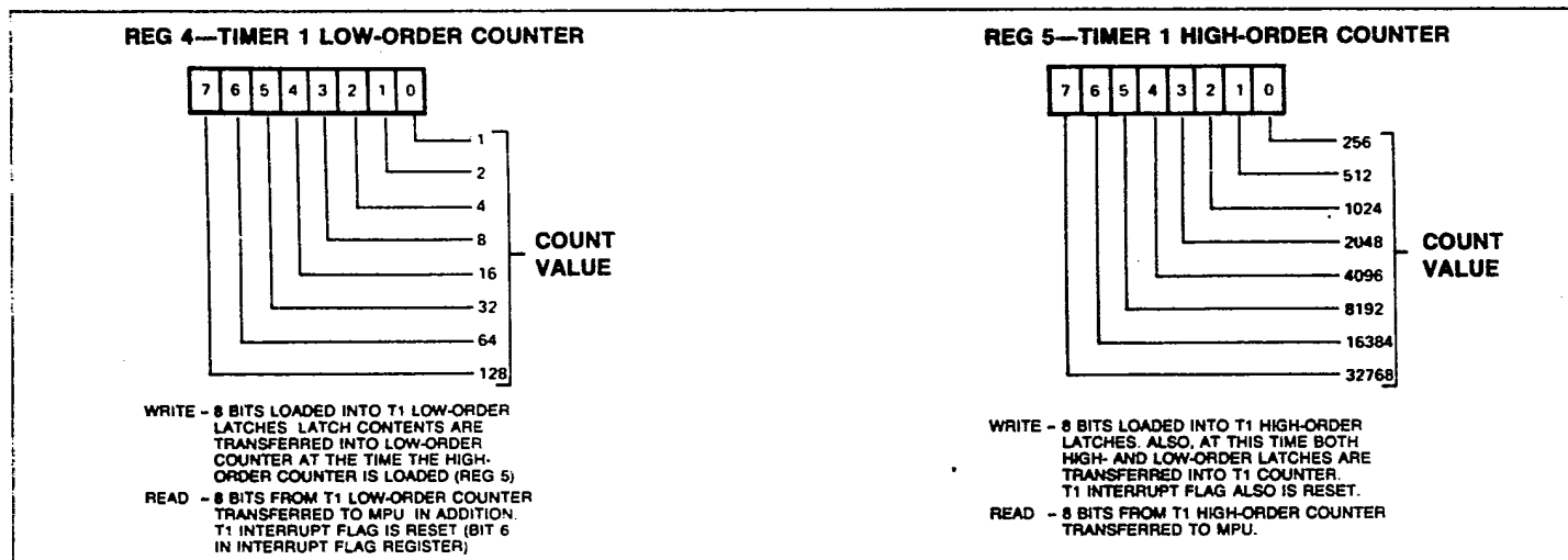
Figure 13: Timer 1 (T1) Counter Registers
