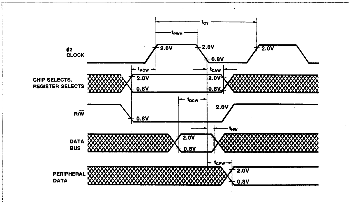
Figure 32b. Write Timing Waveforms
