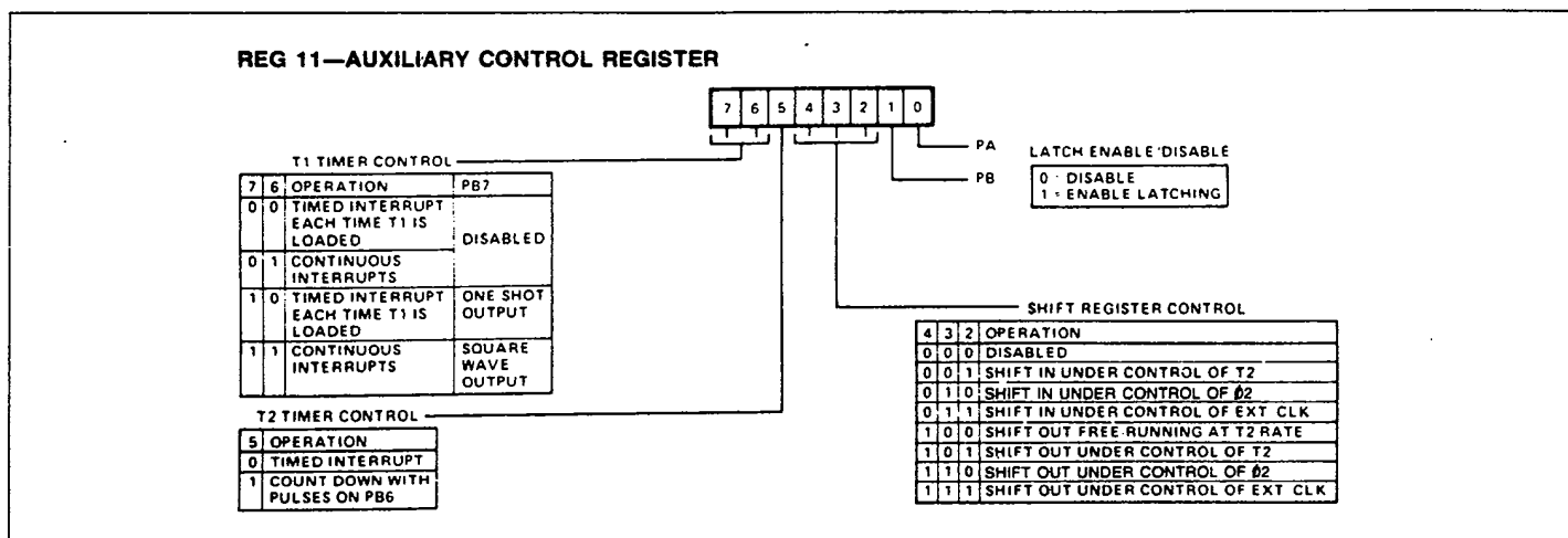
Figure 14. Auxiliary Control Register (ACR)
