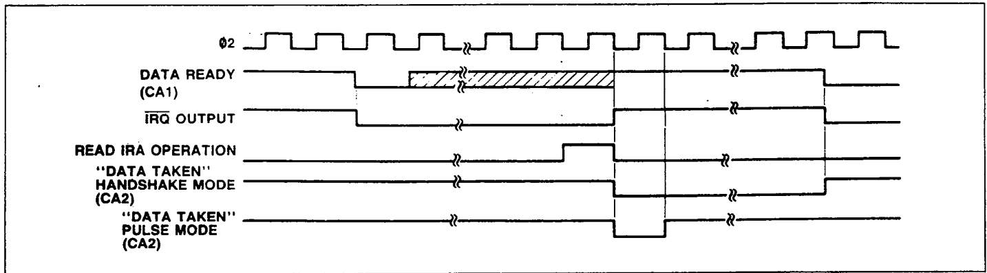
Figure 9. Read Handshake Timing (Port A Only)
