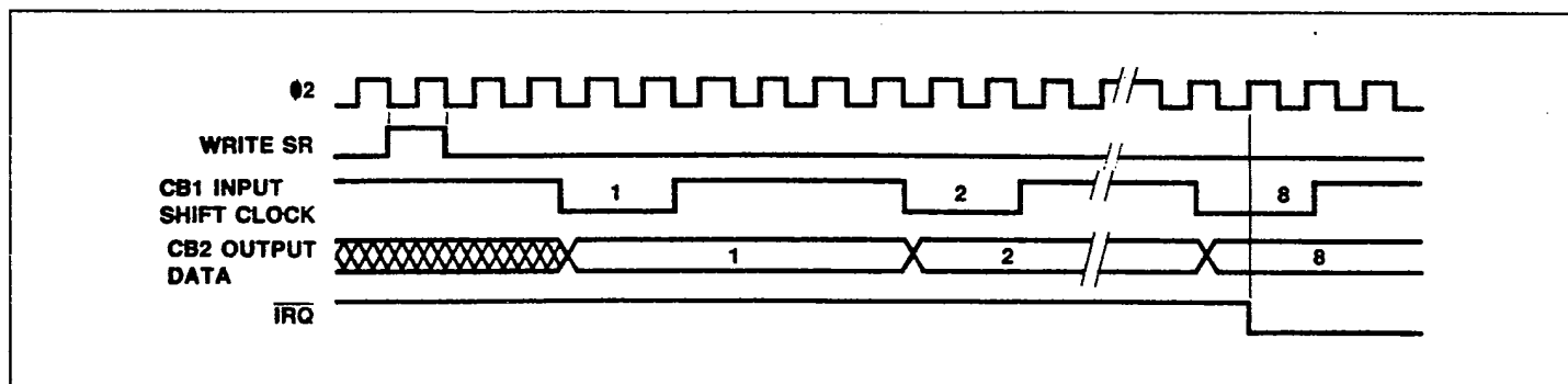
Figure 28. SR Mode 7 — Shift Out Under CB1 Control
