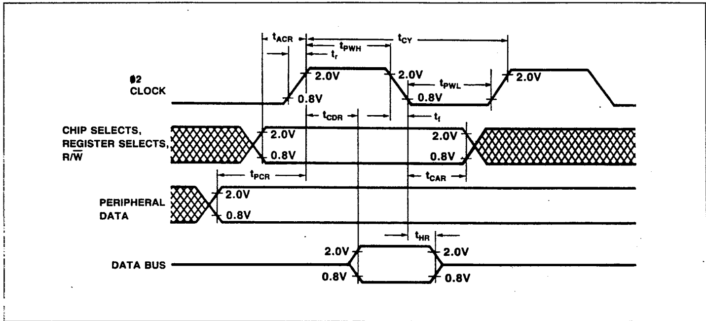
Figure 32a. Read Timing Waveforms
