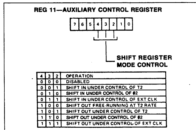
Figure 21. Shift Register Modes
