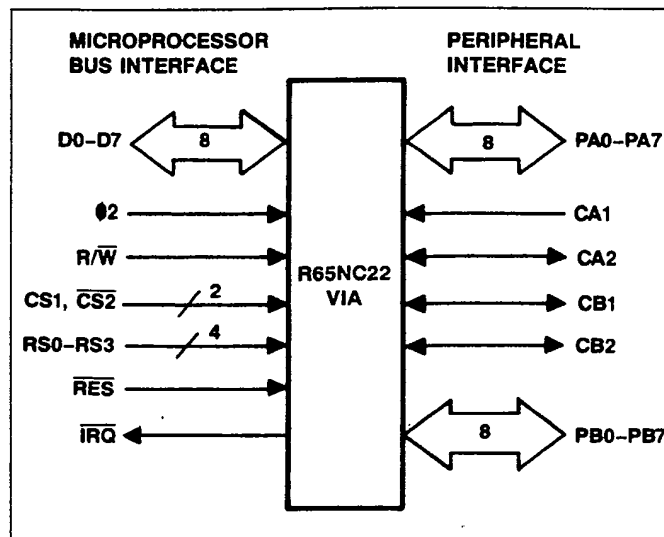
Figure 2. R65NC22 VIA Interface Signals
