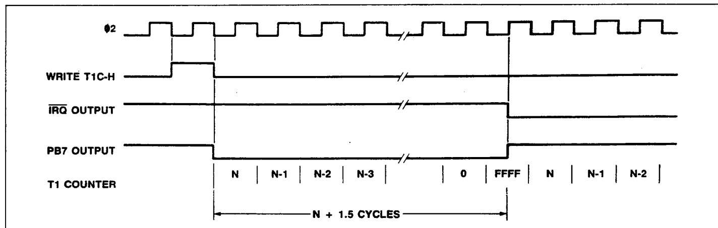
Figure 15. Timer 1 One-Shot Mode Timing
