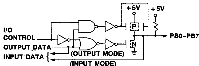
b. Port B Data Line Output Circuit
