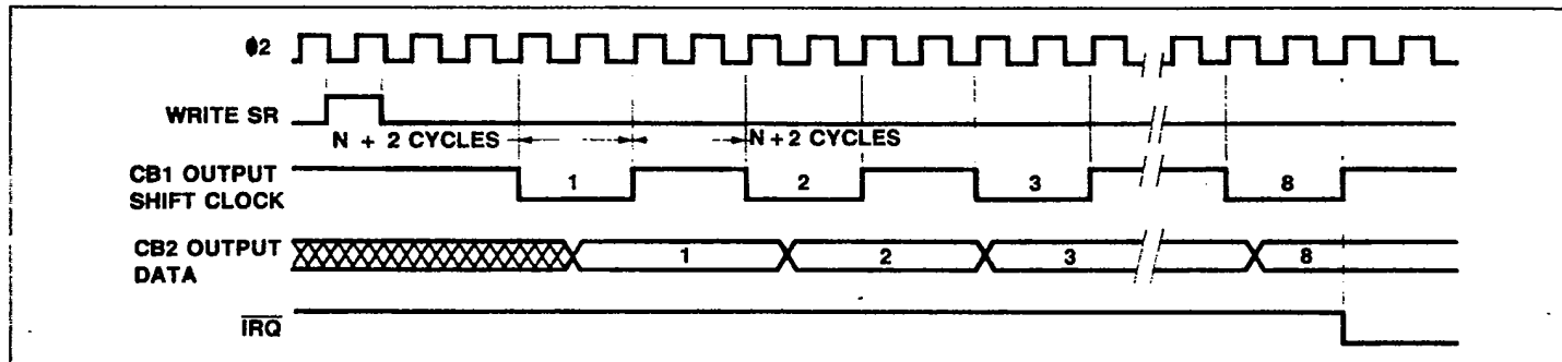
Figure 26. SR Mode 5 — Shift Out Under T2 Control
