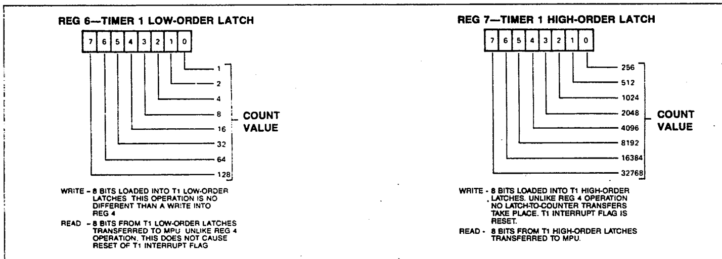
Figure 12: Timer 1 (T1) Latch Registers
