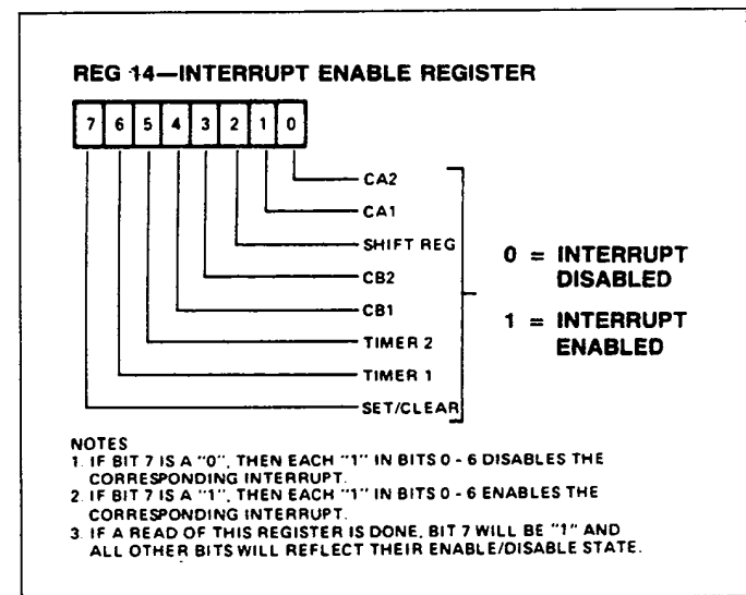
Figure 30. Interrupt Enable Register (IER)
