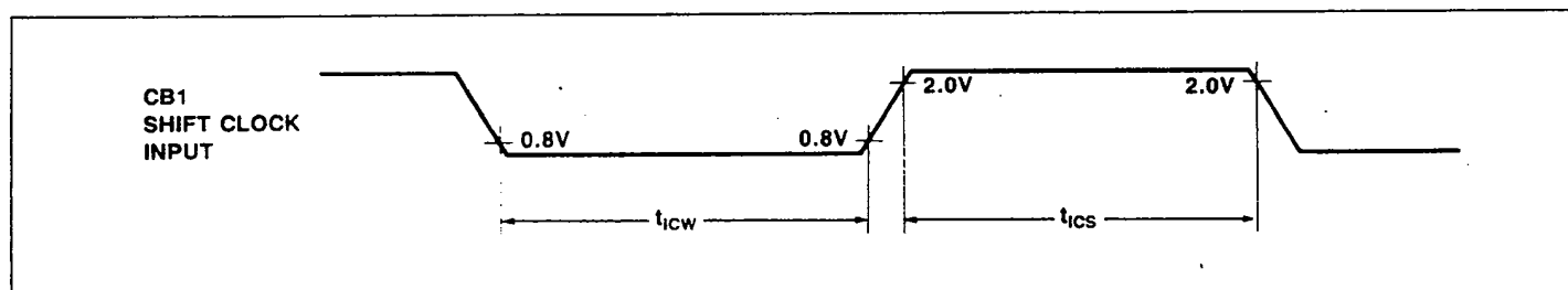
Figure 31h. External Shift Clock Timing
