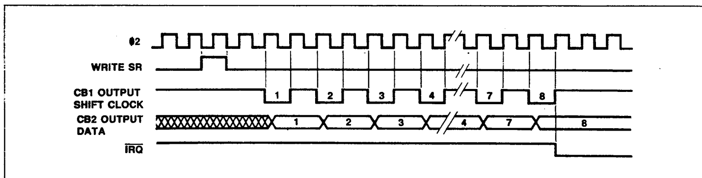
Figure 27. SR Mode 6 — Shift Out Under \phi 2 Control
