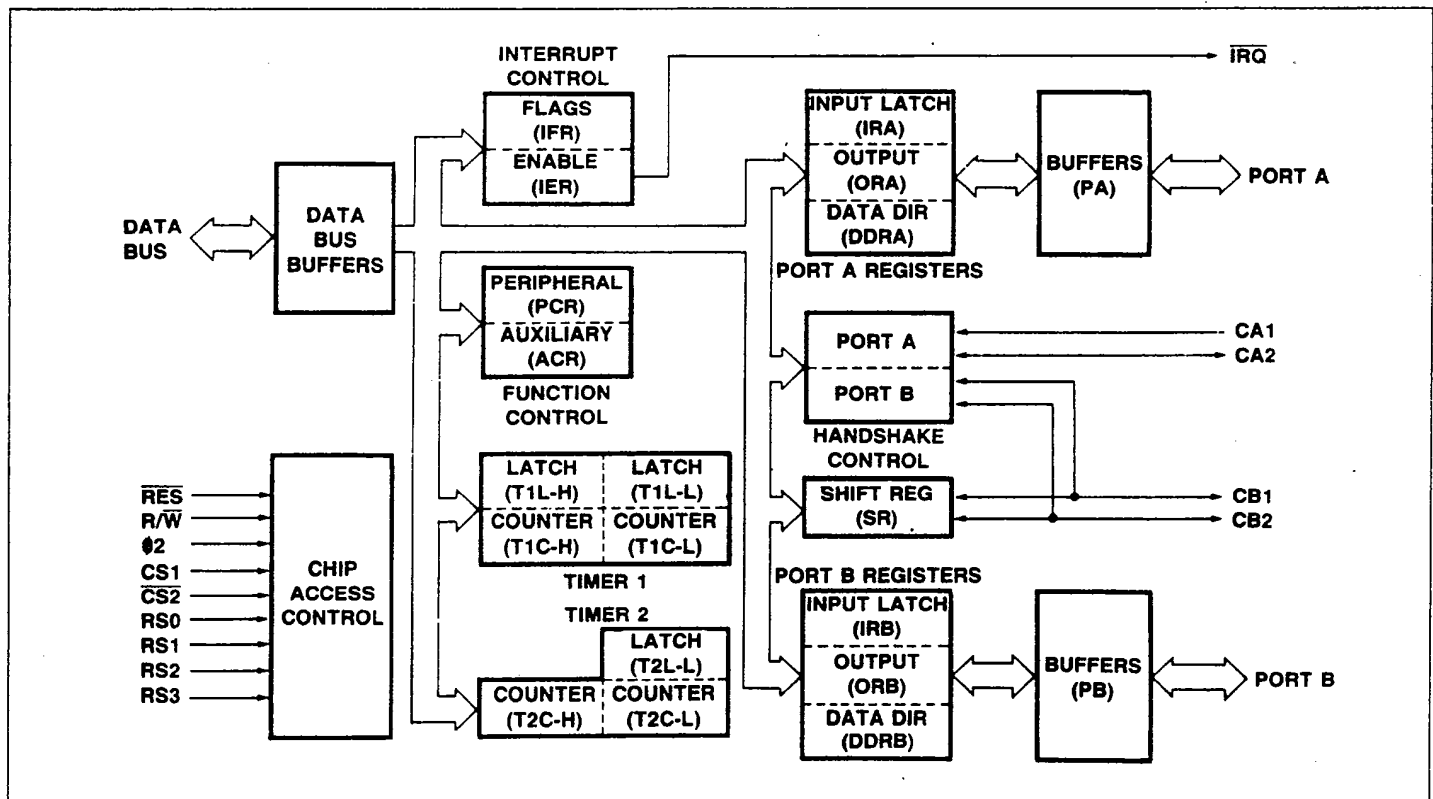
Figure 4. R65NC22 VIA Block Diagram
