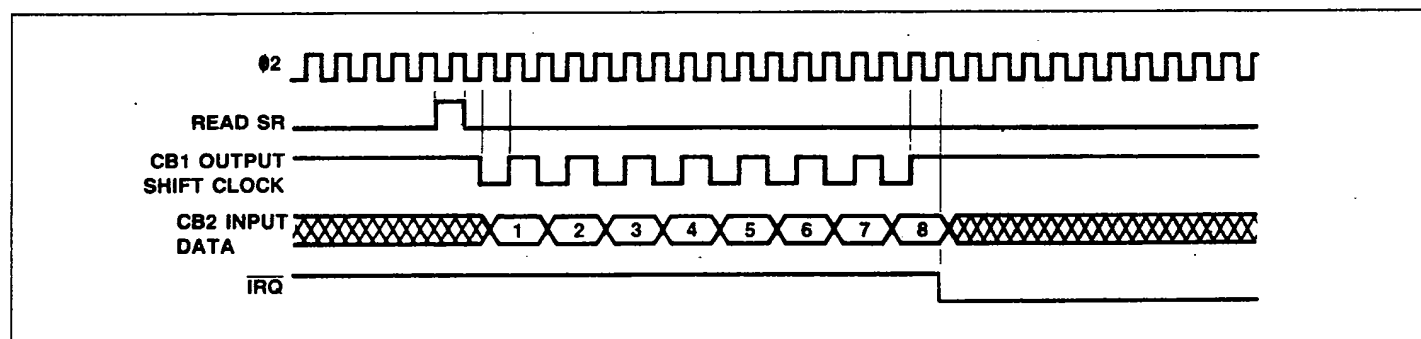
Figure 23. SR Mode 2 — Shift In Under #2 Control
