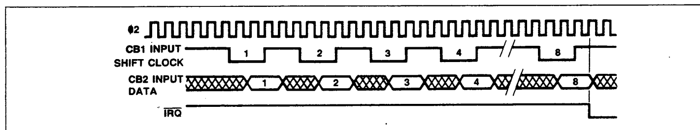
Figure 24. SR Mode 3 — Shift In Under CB1 Control
