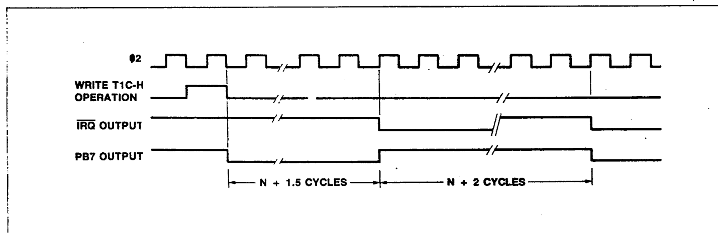
Figure 16. Timer 1 Free-Run Mode Timing
