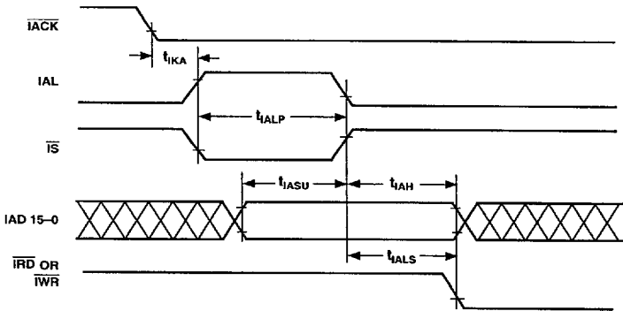
Figure 21. IDMA Address Latch
