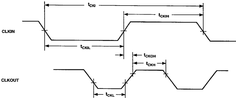
Figure 15. Clock Signals
