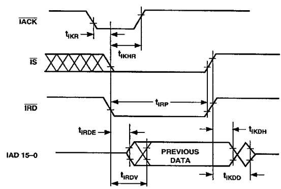
Figure 25. IDMA Read, Short Read Cycle
