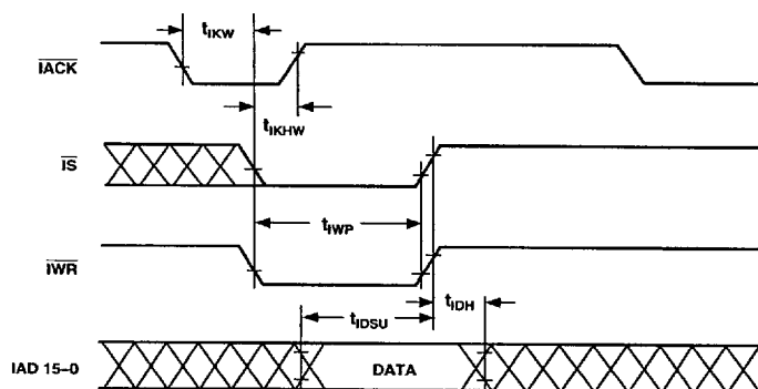
Figure 22. IDMA Write, Short Write Cycle
