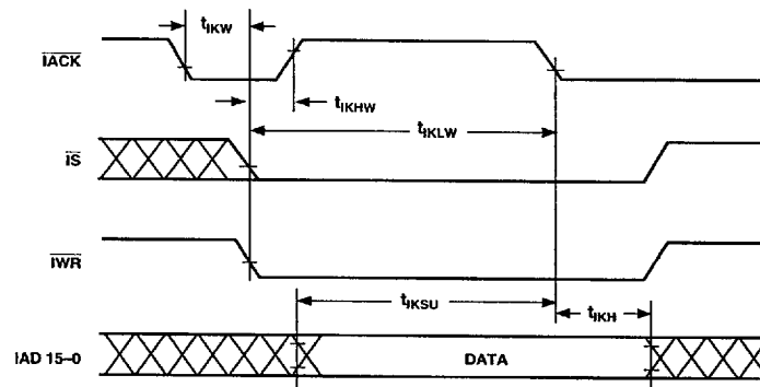
Figure 23. IDMA Write, Long Write Cycle
