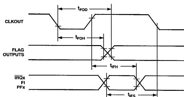
Figure 16. Interrupts and Flags
