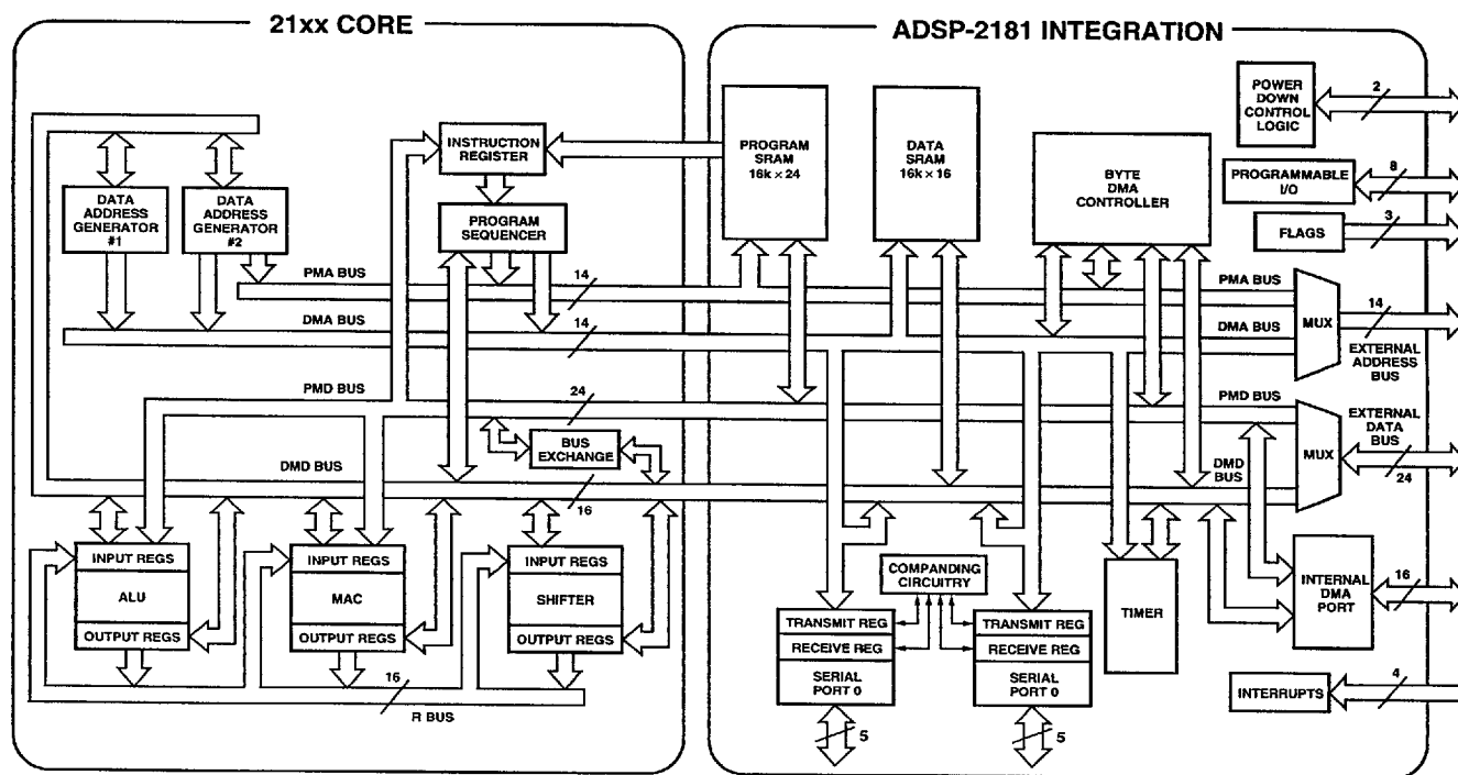
Figure 1. ADSP-2181 Block Diagram
