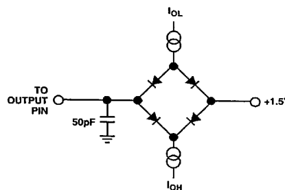
Figure 14. Equivalent Device Loading for AC Measurements (Including All Fixtures)
