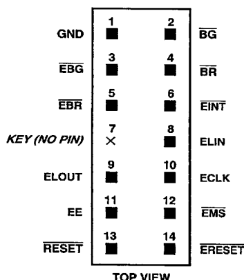
Figure 7. Target Board Connector for EZ-ICE ®
