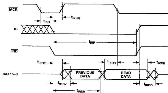
Figure 24. IDMA Read, Long Read Cycle
