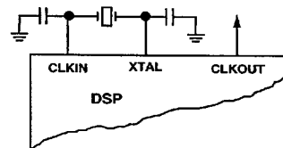
Figure 3. External Crystal Connections
