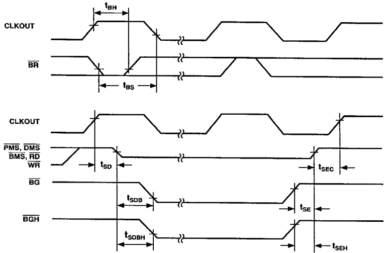
Figure 17. Bus Request-Bus Grant
