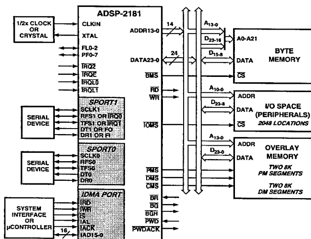
Figure 2. ADSP-2181 Basic System Configuration
