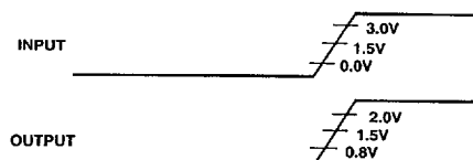
Figure 12. Voltage Reference Levels for AC Measurements (Except Output Enable/Disable)
