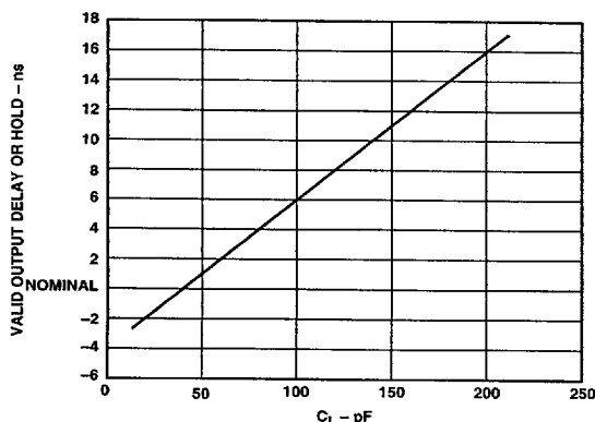
Figure 11. Typical Output Valid Delay or Hold vs. Load Capacitance, C_L (at Maximum Ambient Operating Temperature)
