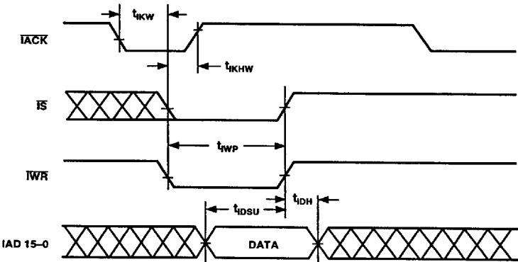
Figure 21. IDMA Write, Short Write Cycle
