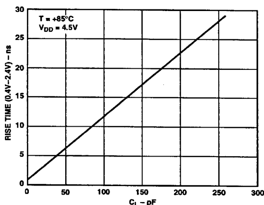
Figure 9. Typical Output Rise Time vs. Load Capacitance, C_L (at Maximum Ambient Operating Temperature)
