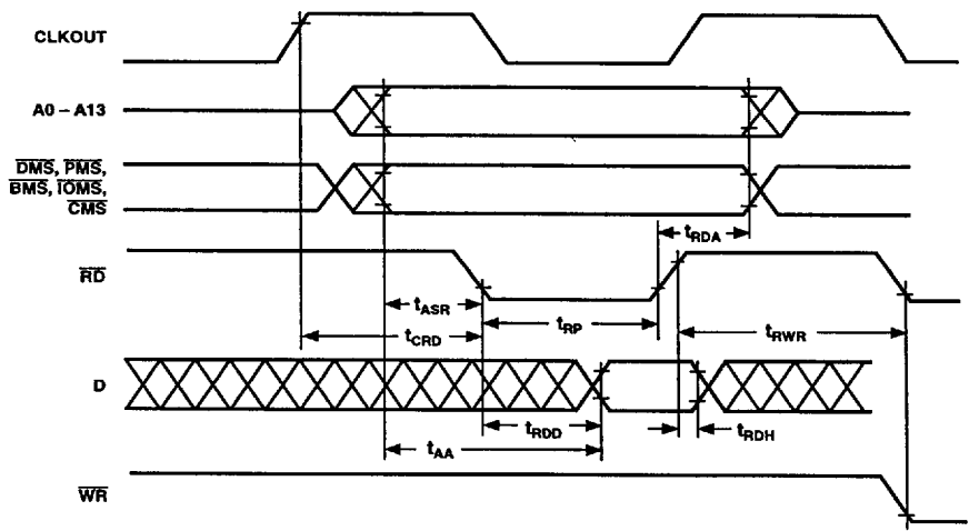
Figure 17. Memory Read
