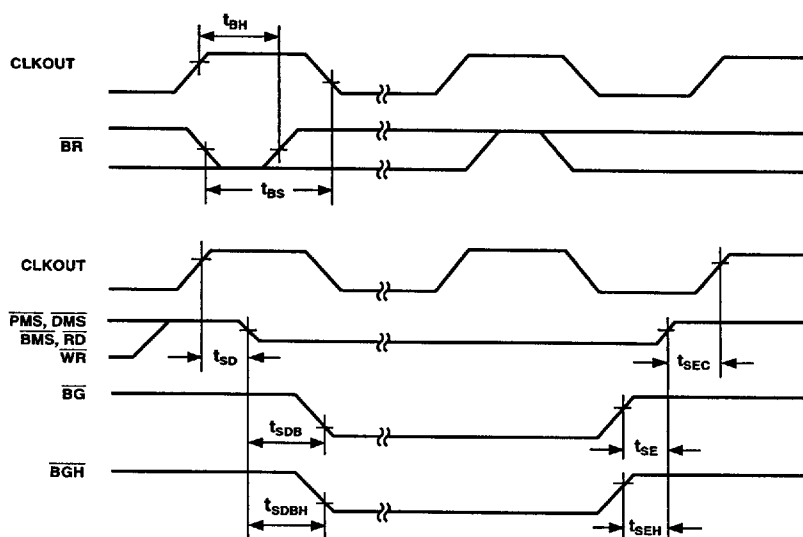
Figure 16. Bus Request-Bus Grant
