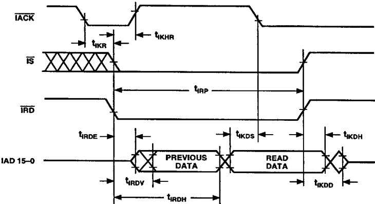
Figure 23. IDMA Read, Long Read Cycle
