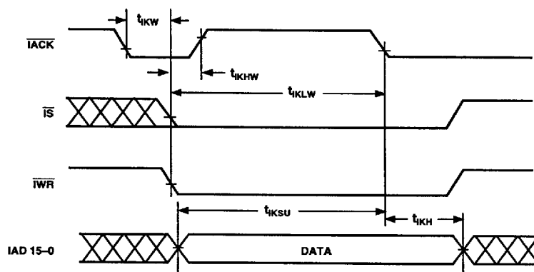
Figure 22. IDMA Write, Long Write Cycle
