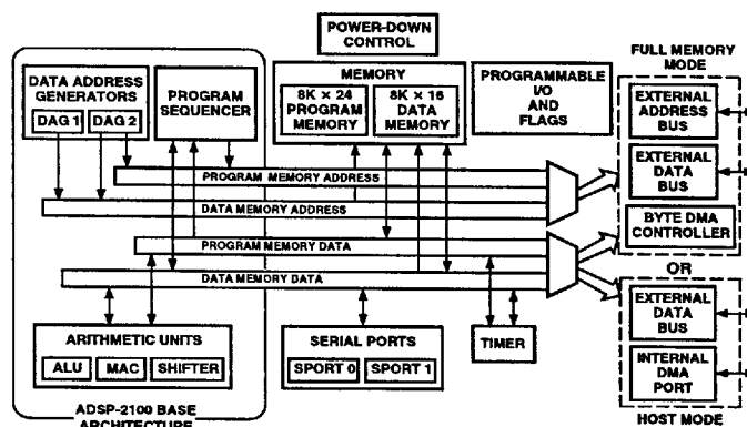
Figure 1. Block Diagram
