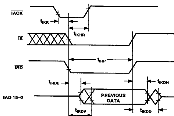
Figure 24. IDMA Read, Short Read Cycle
