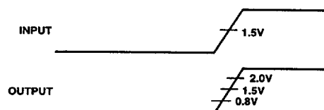
Figure 11. Voltage Reference Levels for AC Measurements (Except Output Enable/Disable)
