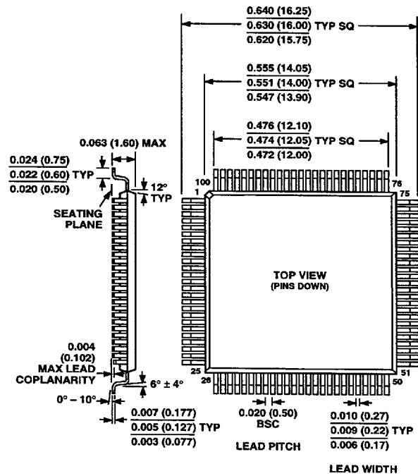
100-Lead Metric Thin Plastic Quad Flatpack (TQFP) (ST-100)
