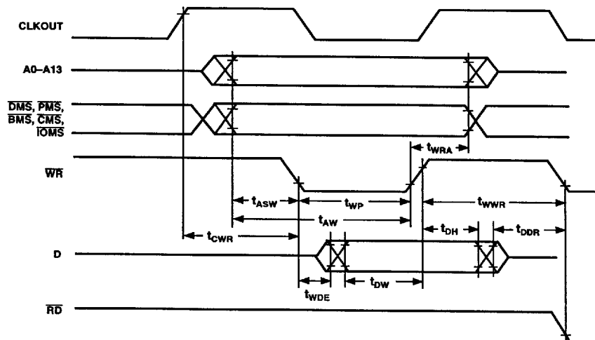
Figure 18. Memory Write
