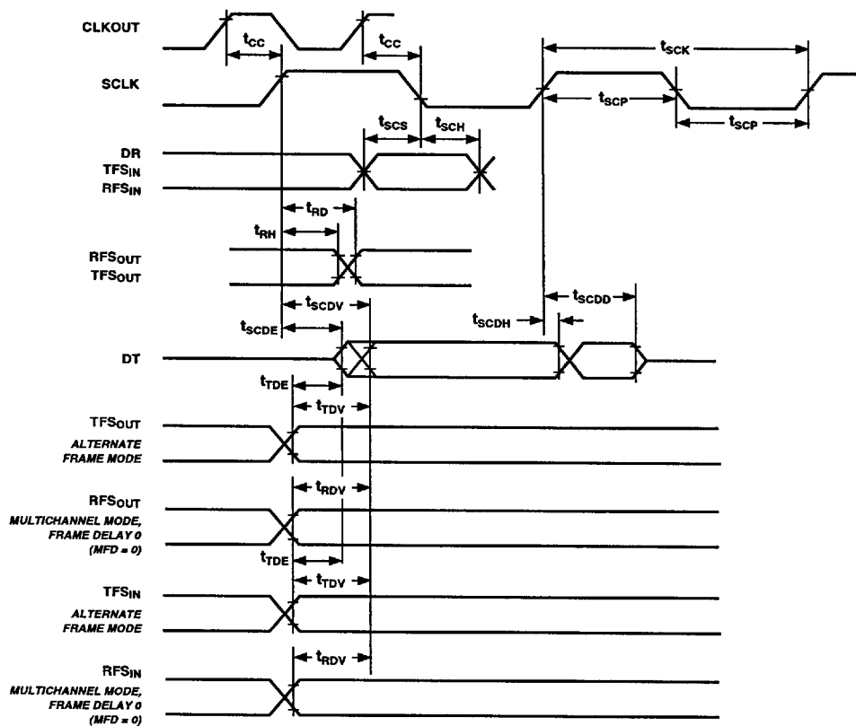
Figure 19. Serial Ports
