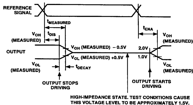
Figure 12. Output Enable/Disable
