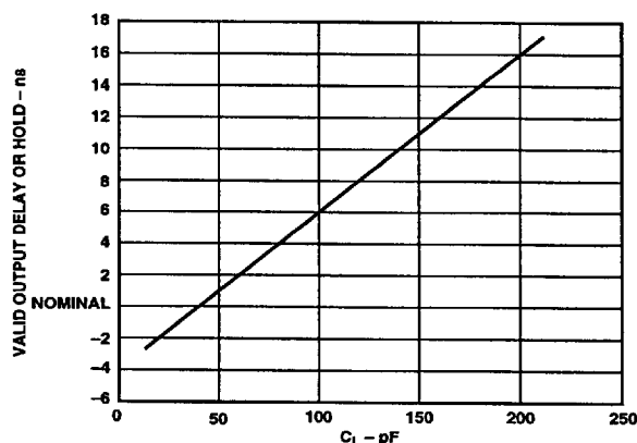
Figure 10. Typical Output Valid Delay or Hold vs. Load Capacitance, C_L (at Maximum Ambient Operating Temperature)
