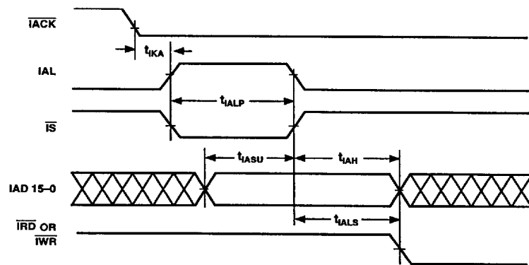
Figure 20. IDMA Address Latch
