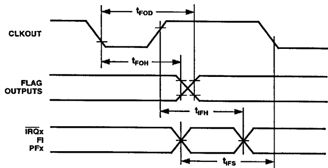
Figure 15. Interrupts and Flags
