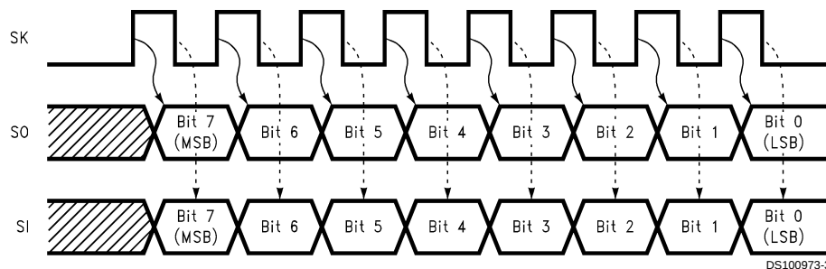
FIGURE 23. MICROWIRE/PLUS SPI Mode Interface Timing, Alternate SK Mode, SK Idle Phase being Low
