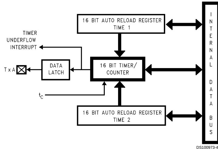
FIGURE 12. Timer in PWM Mode
