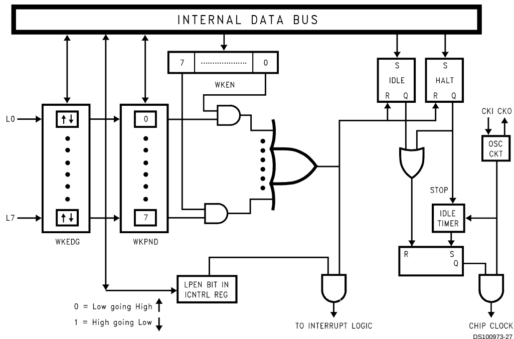
FIGURE 17. Multi-Input Wake Up Logic
