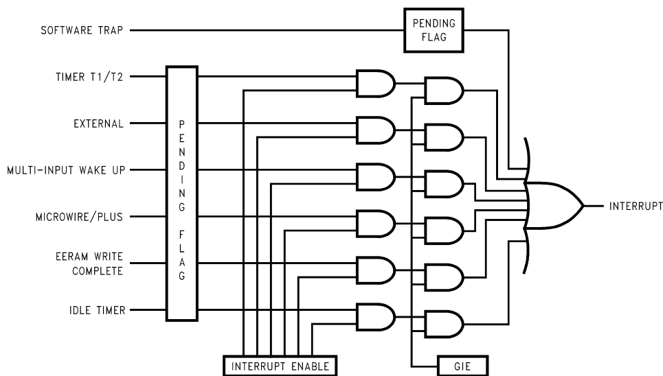
FIGURE 18. Interrupt Block Diagram
