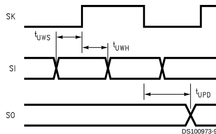
FIGURE 4. MICROWIRE/PLUS Timing
