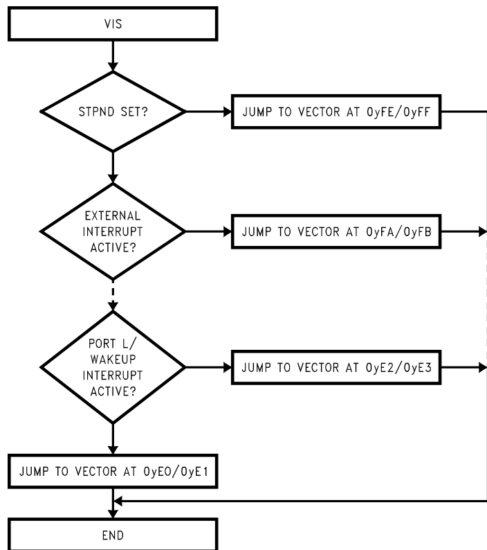
FIGURE 20. VIS Flowchart
