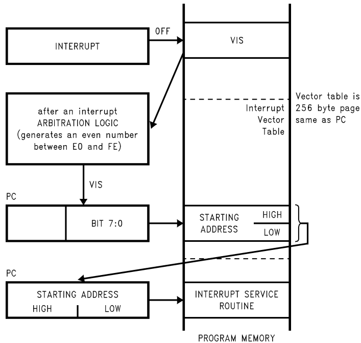
FIGURE 19. VIS Operation
