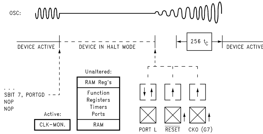
FIGURE 15. Wakeup from HALT
