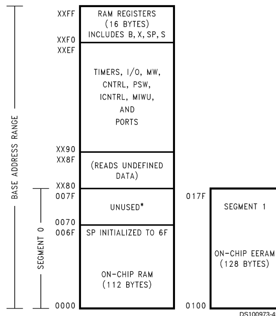
FIGURE 8. RAM Organization
