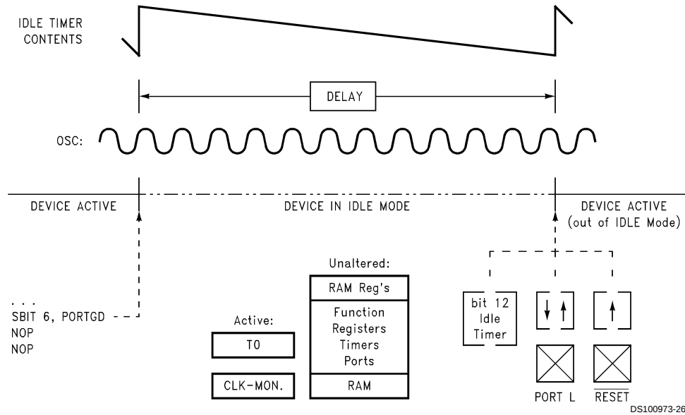
FIGURE 16. Wakeup from IDLE
