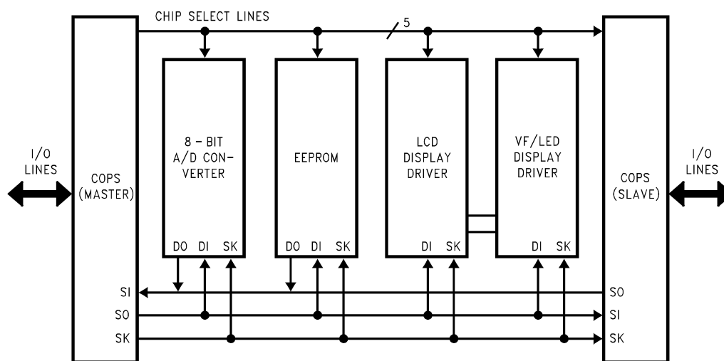
FIGURE 21. MICROWIRE/PLUS Application
