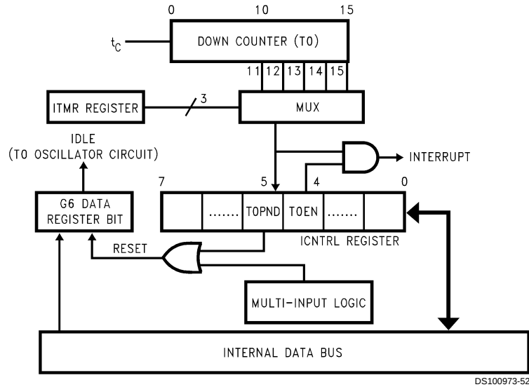
FIGURE 11. Functional Block Diagram for Idle Timer T0
