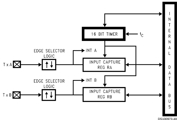
FIGURE 14. Timer in Input Capture Mode
