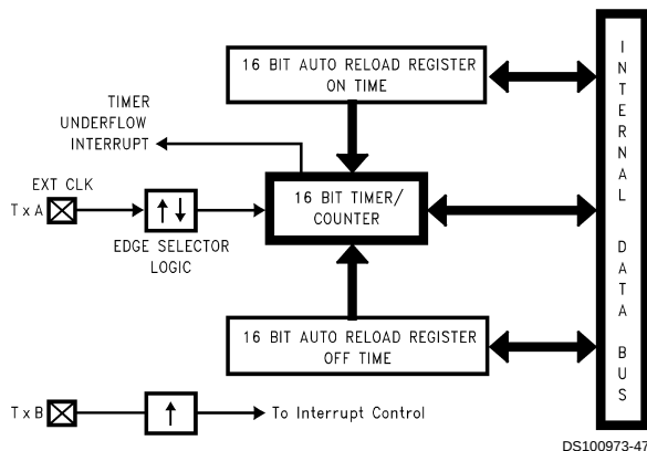
FIGURE 13. Timer in External Event Counter Mode
