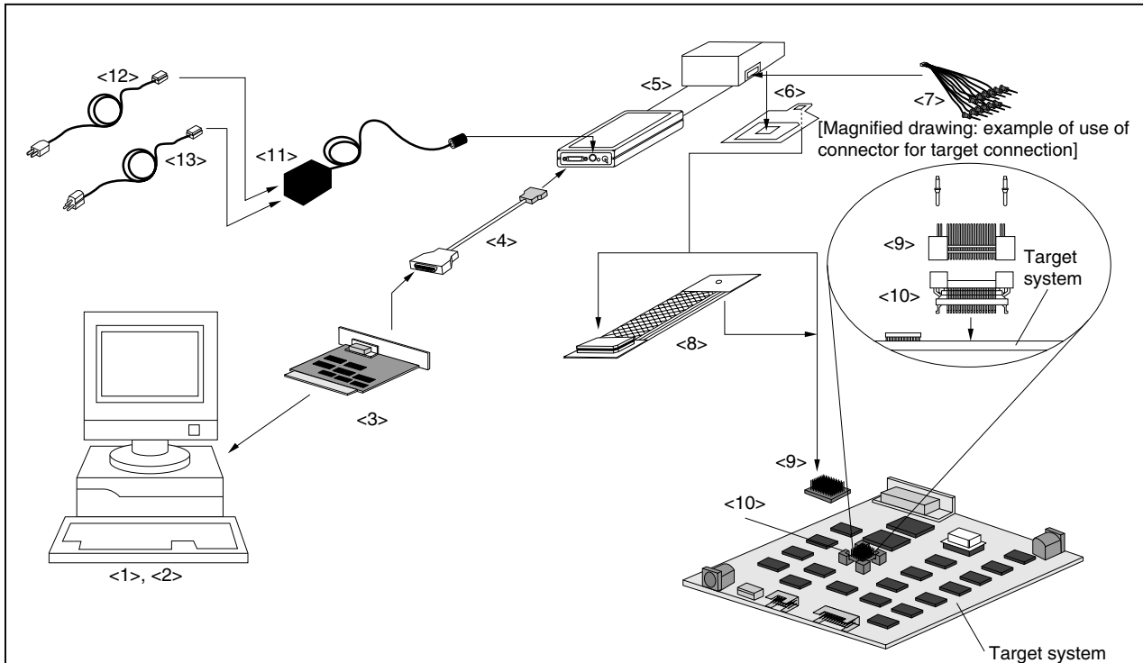
Figure 1-1. System Configuration
