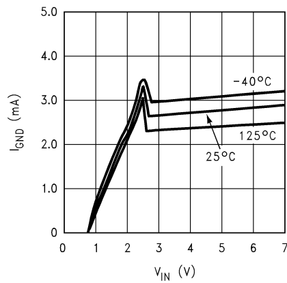
Ground Pin Current Vs Input Voltage ( V_{SD}=V_{IN} )
