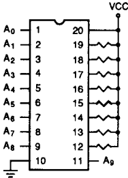
PAL10H8/H8-2 PAL10L8/L8-2
