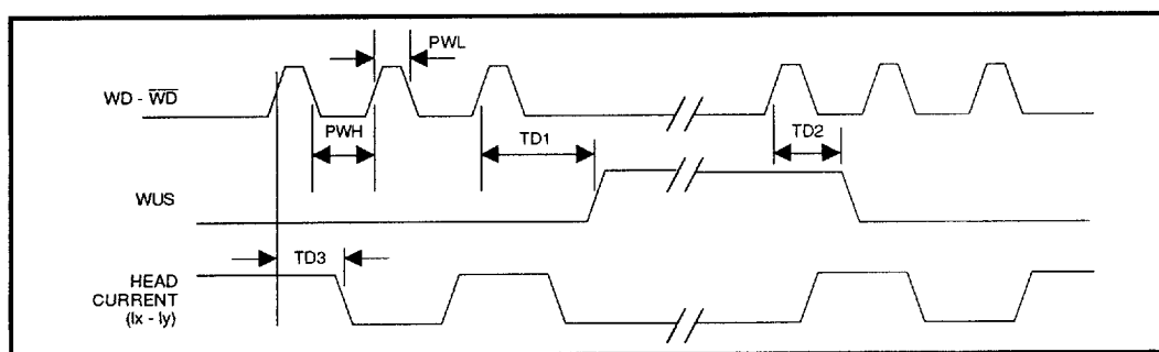
FIGURE 1: 32R2200R/2203R Write Mode Timing Diagram
