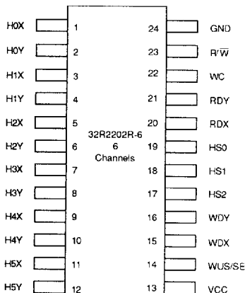
6-Channel 24-Lead SOV, SOL
