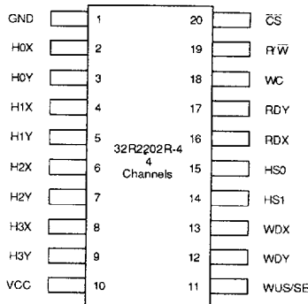
4-Channel 20-Lead SOV, SOL
