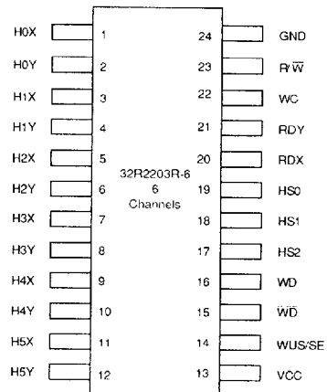
6-Channel 24-Lead SOV, SOL
